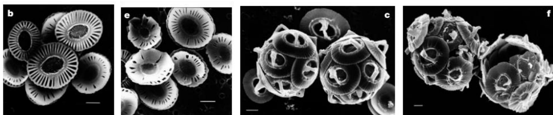
Figure 2.3 - Scanning electron microscopy photographs of coccolithophores under OA.
