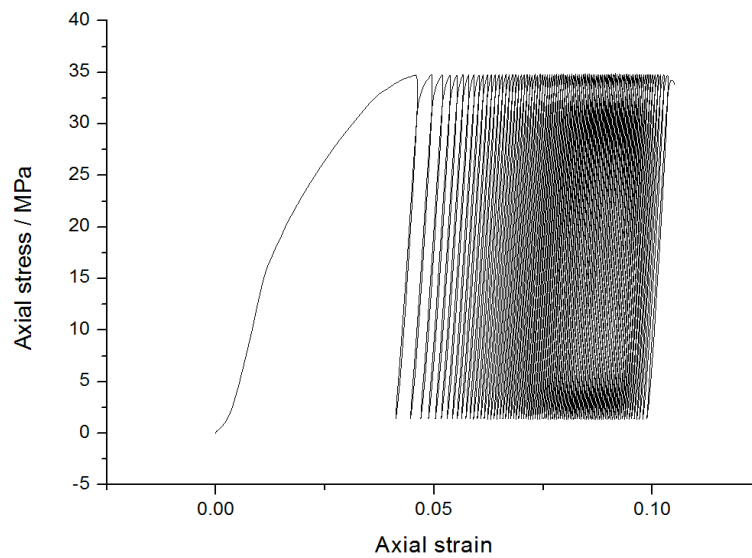
(a) Conventional fatigue test
