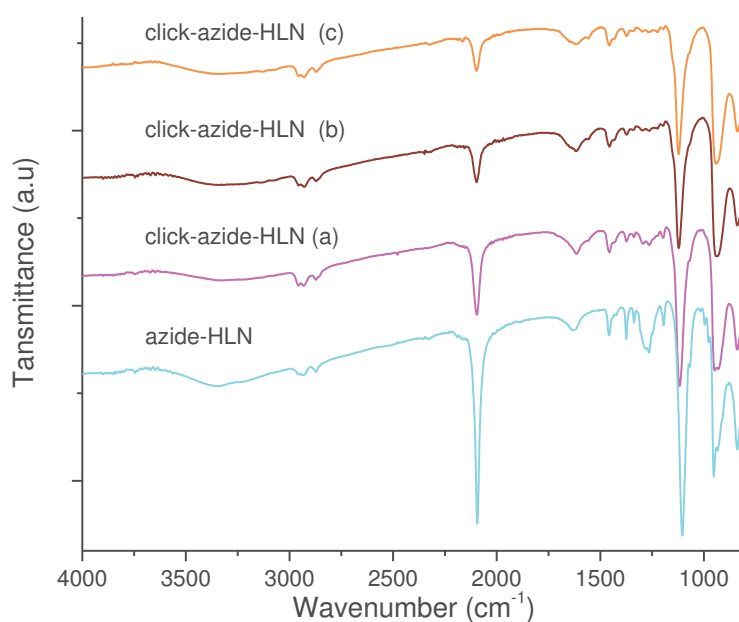
Figure III.30. IR spectra of azide-HLN and its reaction product with 1-hexyne by using different molar amount of \text{CuBr}(\text{PPh}_3)_3 catalyst : (a) : 100 mol %; (b) : 200 mol %; (c) : 400 mol % of catalyst.
