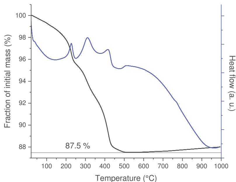
Figure III.28. TGA and DTA curves for azide-HLN.
