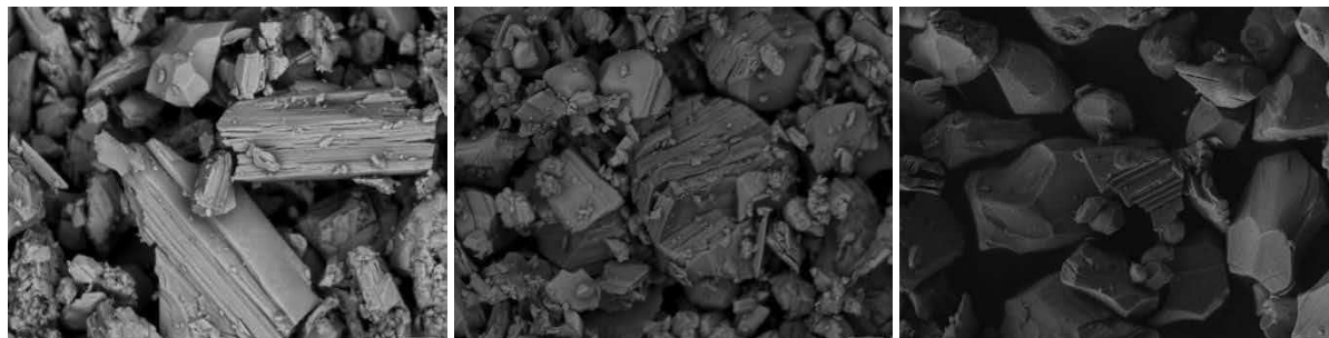
Figure I.9. SEM images of \text{C}_2\text{N}_2\text{-HST} (left), \text{C}_4\text{N-HST} (middle) and \text{HST} (right) (the scale bar corresponds to 1\ \mu\text{m} ).
