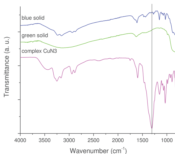
Figure IV.9. Infrared spectra of green solid, blue solid and the complex \text{CuN3}(\text{NO}_3)_2 .
