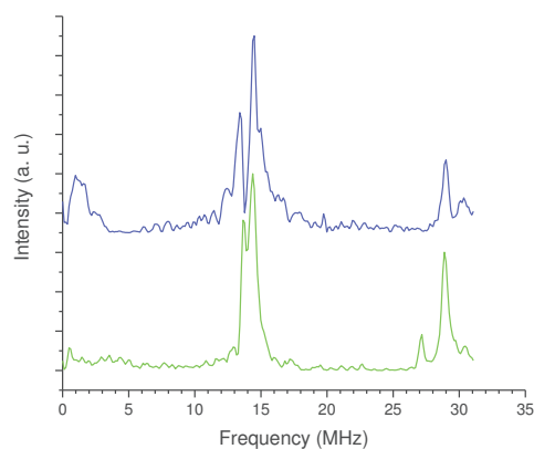
Figure IV.18. ESEEM-2P spectra of the green solid (green) and the blue solid (blue) at 10 K.
