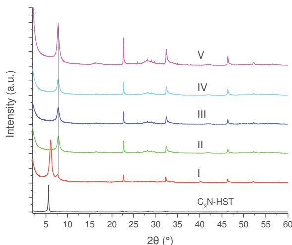
Figure IV.34. PXRD pattern of C_2N -HST and its reaction products with different quantities of copper nitrate (I: 0.006 mmol; II: 0.018 mmol; III: 0.036 mmol; IV: 0.054 mmol; V: 0.090 mmol) according to the conditions presented in Table IV.7 .
