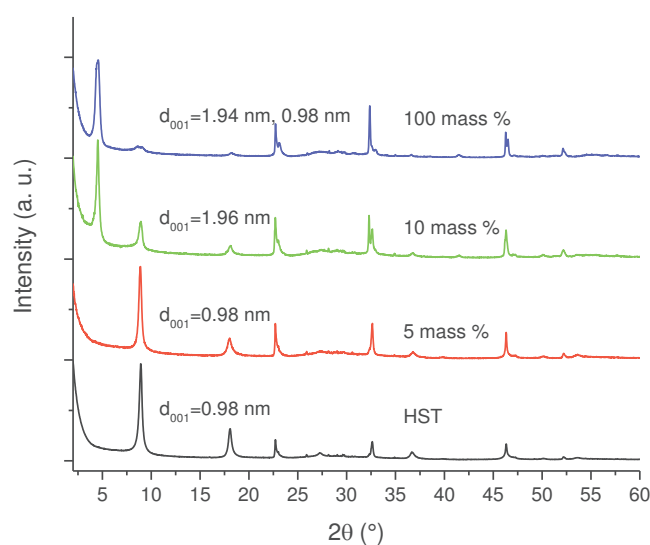
Figure II.34. XRD patterns of HST and its reaction products with 5-amino-1-pentanol by using different amount of water.
