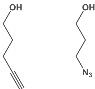
Scheme III.2. 4-pentyn-1-ol (left) and 3-azidopropan-1-ol (right).
