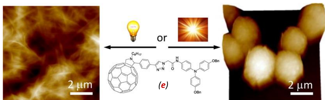
Figure 24 | TAA-fullerene conjugate self-assemblies. Chemical structure and AFM images of the self-assemblies, formed upon irradiation with different light sources. (Left image) nanofibres obtained after irradiation with visible light emitted by halogen lamp; (right image) nanospheres formed upon irradiation with sun light. Figure is reproduced from ref. 114
