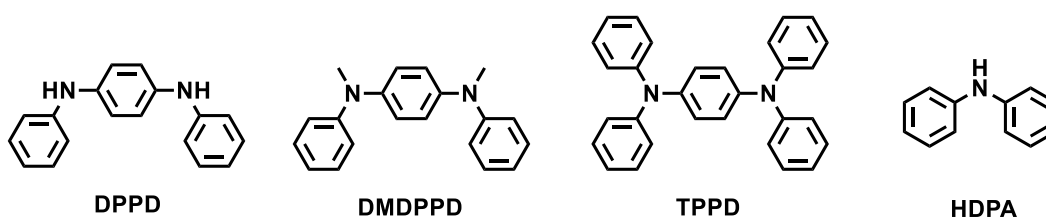
Figure S1 | Chemical structures of molecules studied by Richtol et al. 75
