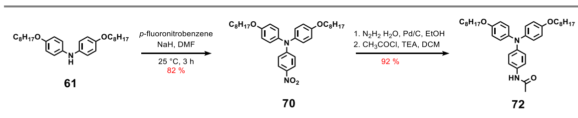
Scheme 20 | Scheme for the synthesis of triaryamine mono-amide, 72 .
