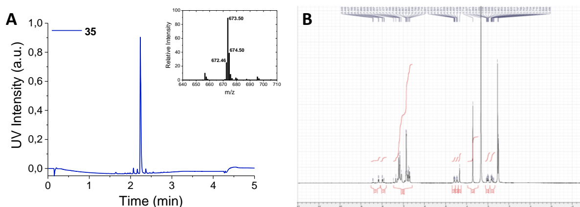
Figure S19 | (A) UPLC chromatograms of control molecule 35 and (B) corresponding 1 H NMR spectrum.
