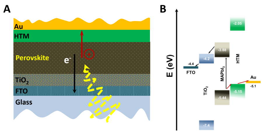
Figure 133 | (A) Scheme of the perovskite solar cell device with planar architecture, used to study TAA derivatives as HTMs. (B) Energy level diagram of a perovskite solar cell built from 52 as example of HTM.
