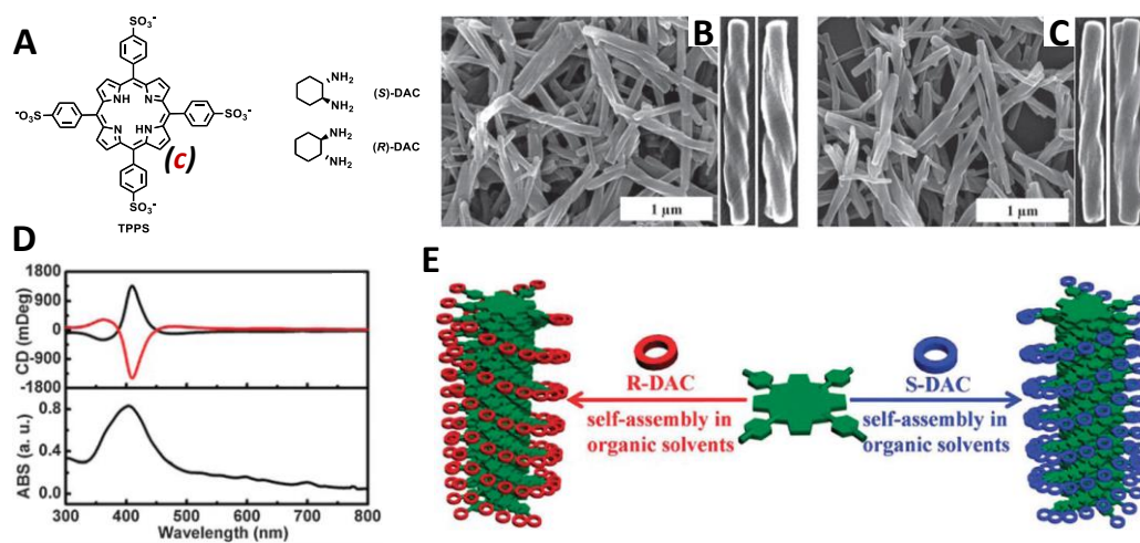
Figure 37 | (A) Chemical structure of water soluble porphyrin, TPSS ( c ) and chiral (S)-DAC and (R)-DAC diamines. (B,C) SEM image of M and P twisted nanorods, obtained after the coassembly of TPSS with chiral diamines. (D) CD (top, black and red line corresponds to R - and S -DAC respectively) and UV-Vis (bottom) spectra of coassemblies. (E) Schematic representation of the supramolecular chirality transfer occurring during the co-assembling process. Figure is adapted from ref. 181
