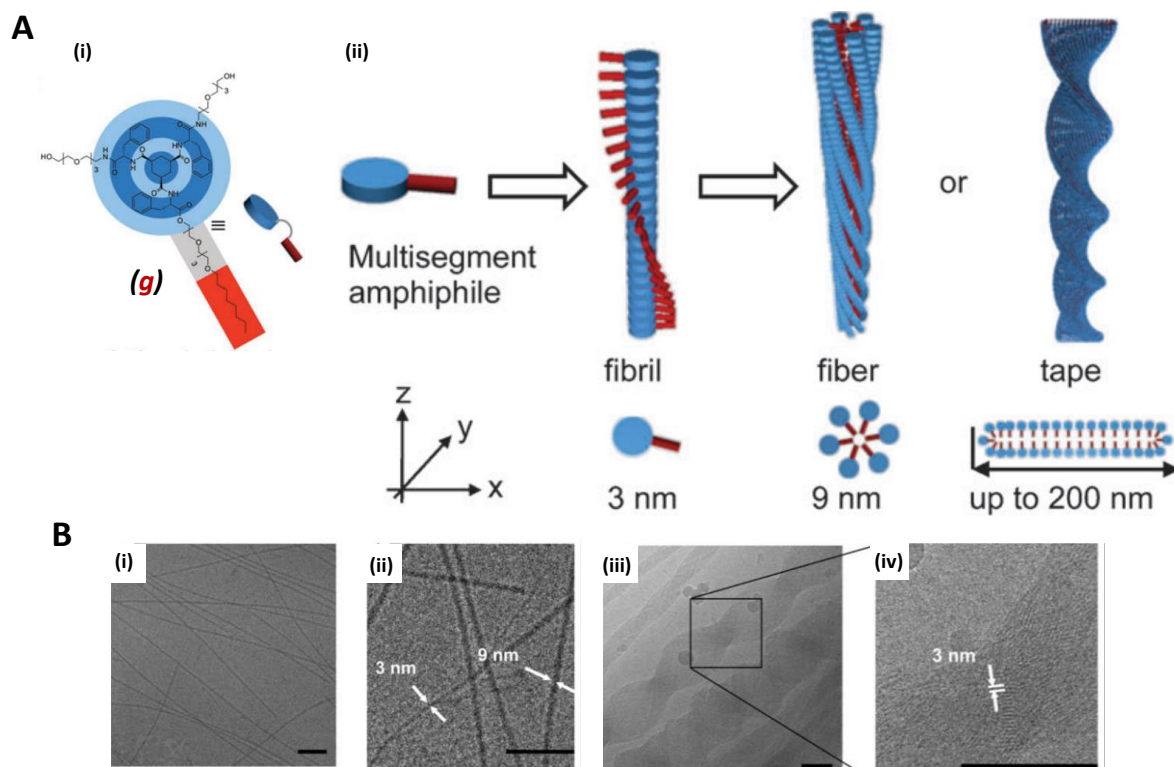
Figure 6 | (A) (i) Multisegment amphiphile g , where light areas represent hydrophilic domains whereas dark areas represent hydrophobic domains. (ii) Schematic representation of the self-assembly of g into fibril, hydrogen bonded in the z-direction. Additionally, due to hydrophobic interactions between the surfactant segments, 5 to 7 fibrils assemble into 9 nm fibers or up to 200 nm tapes depending on the concentration. (B) Cryo-TEM images of (i) fibrous network of g at 0.25 mM displaying fibers with a diameter of 9 nm; (ii) magnification of Fig. B(i) ; (iii) fibrous network of g at a concentration above 0.25 mM. Polydisperse twisted tapes of 50 to 200 nm in diameter are formed; (iv) magnification of Fig. B(iii) showing substructures consisting of fibrils of 3 nm in diameter. Scale bar: 100 nm. Figure is adapted from ref. 21
