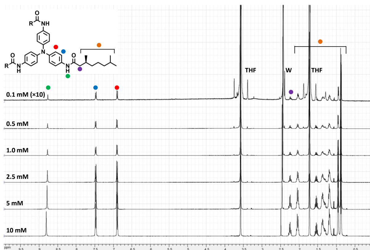
Figure 59 | ^1\text{H} NMR spectra of ( S )- TATA in deuterated THF at different concentrations.
