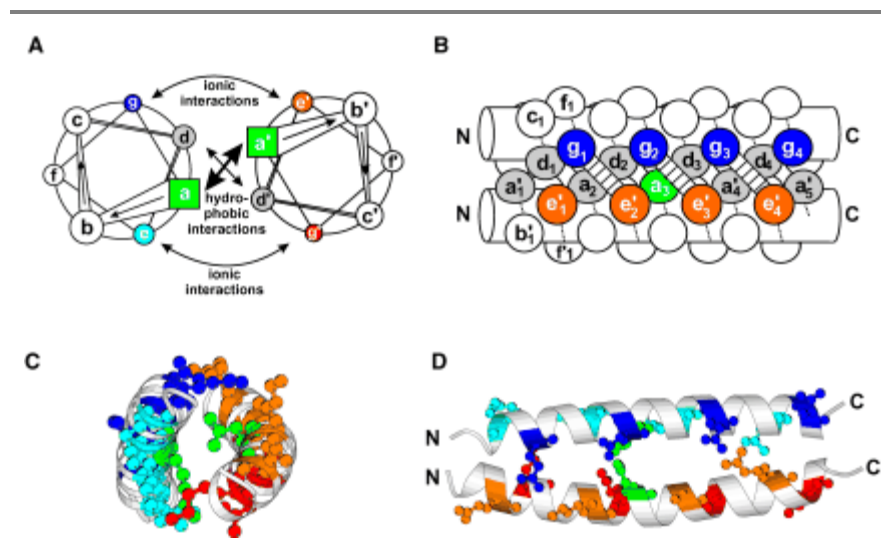
Figure 78 | (A, B) Schematic representation of a parallel dimeric coiled-coil. (C, D) X-ray structure of the leucine zipper of GCN47 as ribbon plot. Figure is reproduced from ref. 262
