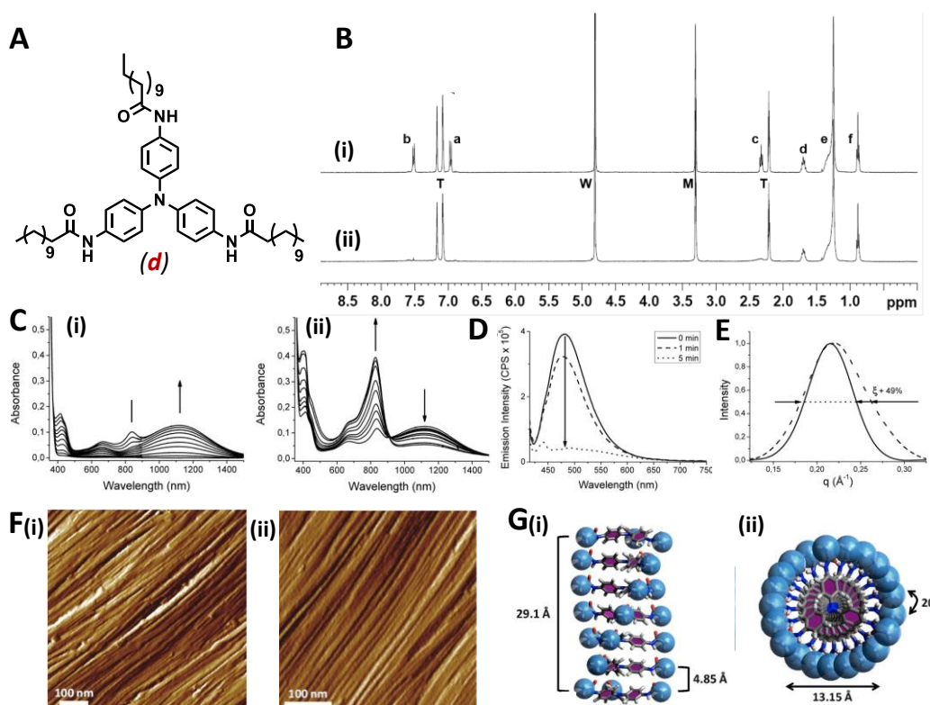
Figure 23 | Second generation of self-assembling triarylamine. (A) Chemical formula of TATA- d and (B) associated 1 H NMR of TATA- d in a 5:3 methanol:toluene mixture, in the presence of CDCl 3 (5 vol %) before (i) and after (ii) light irradiation. (C) Effect of light irradiation on TATA self-assemblies. (i,ii) Sequential absorbance spectra taken during light irradiation of a 0.1 mM solution of TATA- d in CHCl 3 ; (i) first 6 min of light irradiation, (ii) from 7 to 73 min of light irradiation. (D) Fluorescence emission of TATA- d upon light irradiation showing the quenching induced by the polaron formation. (E) SAXS of nonirradiated (dotted line) and irradiated (full line) thin films demonstrating a 49% increase in the correlation length (calculated as 4\pi/\text{fwhm} ). (F) AFM image of TATA- d obtained from the drop cast of a chloroform solution before light irradiation (i) and after 15 min of light irradiation (ii) showing the healing of structural defects. (G) Side view (i) and top view (ii) of the proposed stacking structure of TATA- d , as obtained from DFT calculations, and with a longitudinal periodicity of 29.1 Å, a nitrogen–nitrogen distance of 4.85 Å between adjacent molecules, and a dihedral angle of 20° between each plateau. Figure is adapted from ref. 113
