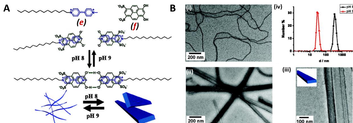
Figure 5 | (A) Schematic illustration of the hierarchical nanoribbons self-assembly of aromatic amphiphiles. (B) TEM images of the aggregates of ( e-f ) at pH 9 (i). (ii and iii) Magnified TEM images of the aggregates at pH 8. (iv) Distribution of the hydrodynamic diameter of ( e-f ) at pH 9 and pH 8. Figure is adapted from ref. 20
