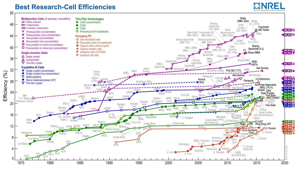
Figure 116 Timeline chart of the certified reported photoconversion efficiencies of the most common types of solar cells recorded since 1975. Chart is taken from the web page of the National Renewable Energy Laboratory. 298
