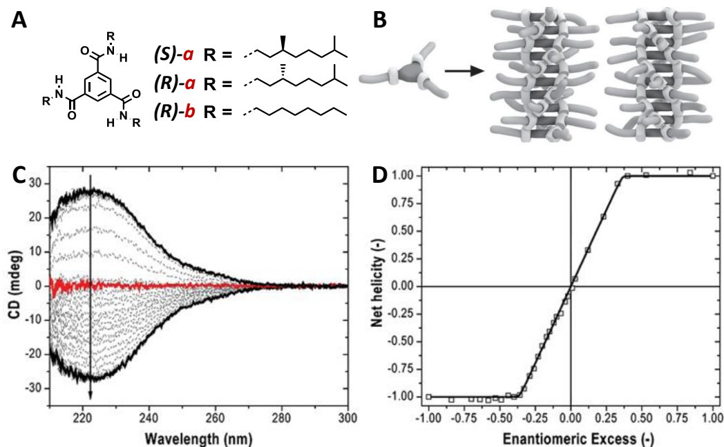
Figure 35 | (A) Chemical structure of BTA molecules decorated with chiral ( S/R )- a and achiral alkyl chains ( b ). (B) Schematic representation of right and left-handed helices formed during the self-assembling process. (C) CD spectra of pure ( R )-BTA (top black), pure ( S )-BTA (bottom black) and their equimolar mixture (red). (D) Dependence of the helicity of the system based on its composition. Figure is adapted from ref. 176
