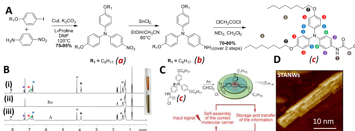
Figure 21 | Light-triggered self-assembly of triarylamine nanowires. (A) Synthetic scheme and chemical structure of a first generation self-assembling triarylamines ( c ). (B) 1 H-NMR spectra of c in chloroform (i) immediately after the purification, (ii) after irradiation with visible light and (iii) after heating for 60 °C overnight. The insets shows the solution of c in the NMR tube before and after irradiation. (C) Schematic representation of the light-induced self-assembly process. (D) AFM image of the supramolecular corn-like TAA fiber. Figure is adapted from ref. 81
