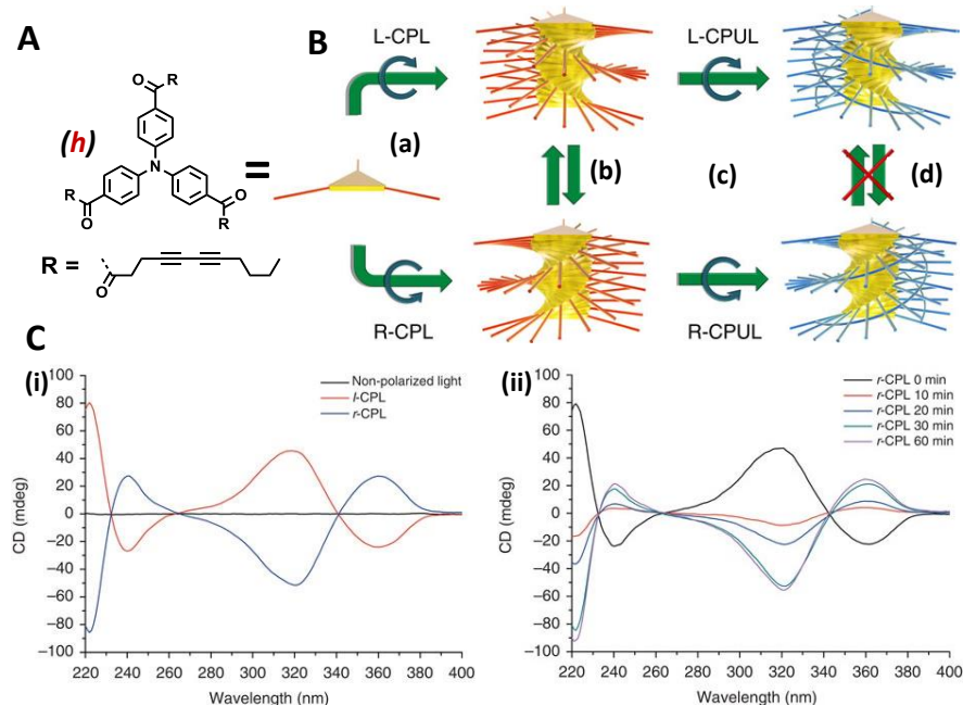
Figure 42 | (A) Chemical structure of achiral TATA molecule ( h ) decorated with diyne side-chains. (B) Schematic representation of the self-assembling process. (a) R-CPL or L-CPL dictates the helicity of nanofibres of TATA, (b) M/P helix transformations upon irradiation with corresponding CPL. (c) Cross-photopolymerization of diyne-functions with corresponding CPUL. (d) After the polymerisation chirality of assemblies do not change upon irradiation with CPL. (C) CD spectra of self-assemblies. (i) CD spectra demonstrating process (a) of Fig.B . (ii) CD spectra, demonstrating chirality inversion, described as (b) on Fig.B . Figure is adapted from ref.120
