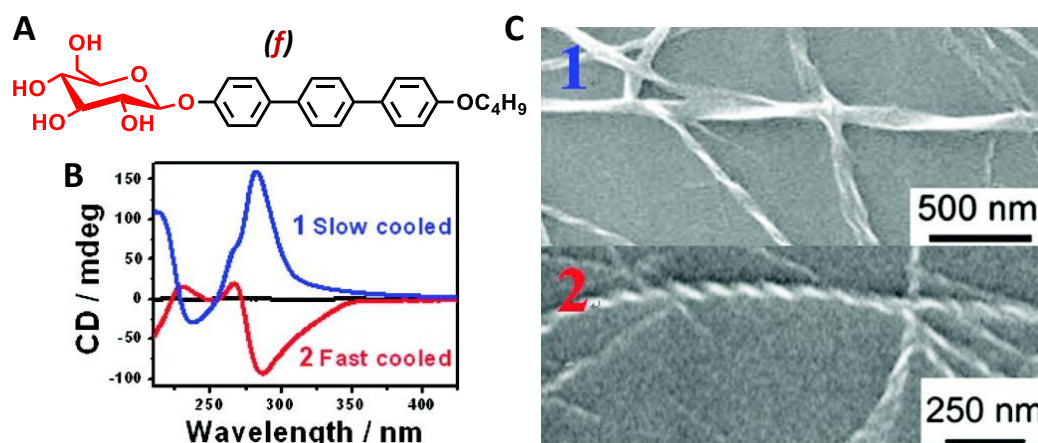
Figure 40 | (A) Chemical structure of sugar-based gelator ( f ). (B) CD spectra corresponding to the slow cooling and the fast cooling gels. (C) SEM images of aggregates, obtained during the slow cooling ( 1 ) and fast cooling ( 2 ) processes. Figure is adapted from ref. 183
