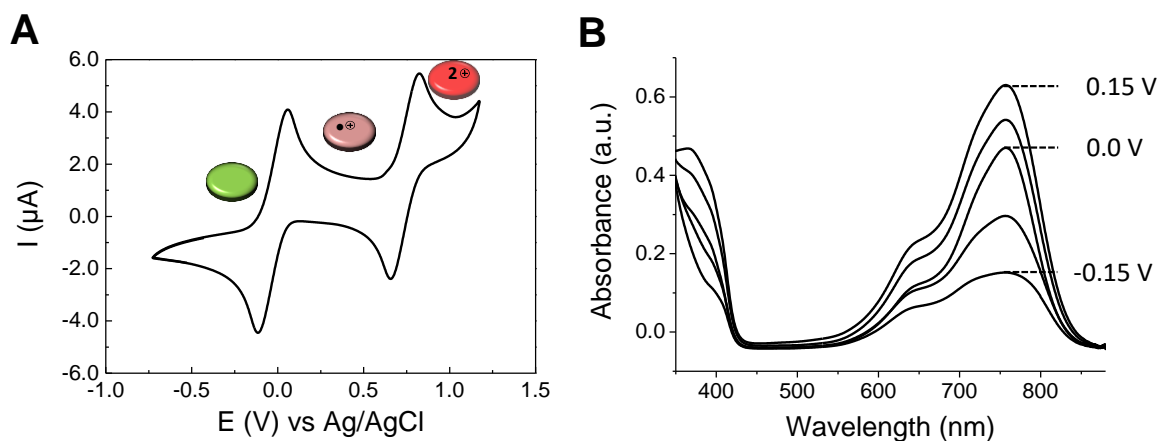
Figure 144 | (A) Cyclic voltamogram of compound 72 at a concentration of 1 mM in TCE with 0.1 M TBAHFP and at a speed of 100 mV·s -1 . (B) Spectroelectrochemical behavior of 72 for different potential scans over the first oxidation wave in the range -0.15 to 0.15 V vs Fc/Fc + in TCE with 0.1 M TBAHFP.
