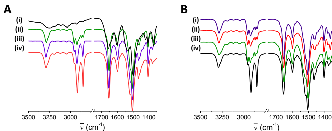
Figure 60 | FTIR spectra on solid samples for (A) TATAs as obtained after purification; (i) TATA-Ac (reported by Armao et al. 130 see Figure 61), (ii) (S)-TATA, (iii) (C 9 )-TATA, (iv) (C 14 )-TATA, and (B) (S)-TATA, which was assembled in different solvents (i) acetonitrile, (ii) acetone, (iii) toluene, (iv) (C 14 )-TATA assembled in chloroform. 225
