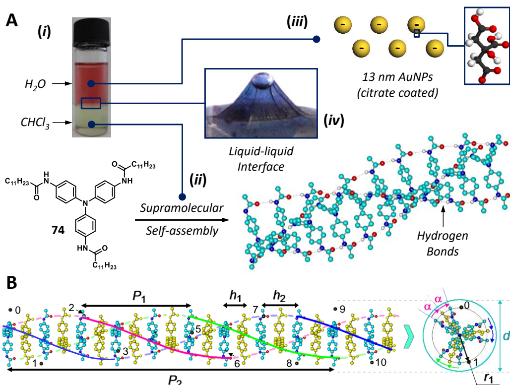
Figure 160 | (A) Different components involved in the formation of the hybrid TATA/Au film at the liquid/liquid interface. (i) Photograph of the biphasic system with chloroform (lower layer) and water phases (upper layer) after shaking. (ii) The chloroform layer contains TATA supramolecular nanowires, doped upon light irradiation with TATA radical cations. (iii) The aqueous layer contains a suspension of citrate stabilized 13 nm size gold nanoparticles (Au NPs). (iv) An air bubble, trapped under the hybrid film, formed at the interface. (B) Characteristics of a TATA nanofiber doped with radical cations, composed from 22 TATA units. Chlorine counterions are marked as black dots numbered from 0 to 10; coloured lines represent the three chains of H-bonded amide groups; h_1 = 0.485 nm, distance between the central nitrogens of neighbouring TATA molecules; P_1 = 6h_1 , apparent helical period; P_2 = 3P_1 = 18h_1 , full helical period; h_2 = 2h_1 contour length per radical.
