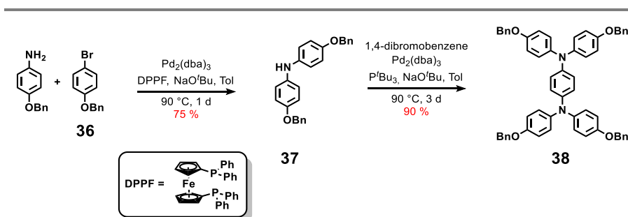
Scheme 18 | Synthesis of two-center tetrabenzoyloxy compound 38 .
