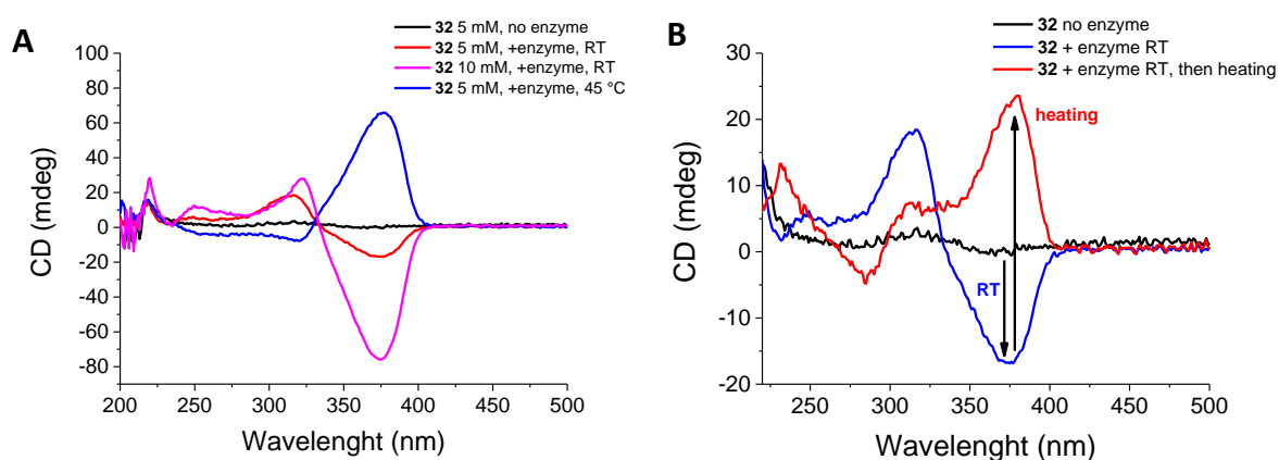
Figure 114 | CD spectra for enzymatically triggered self-assemblies of 32 (A) incubated at different temperatures and (B) Thermal chirality switching.
