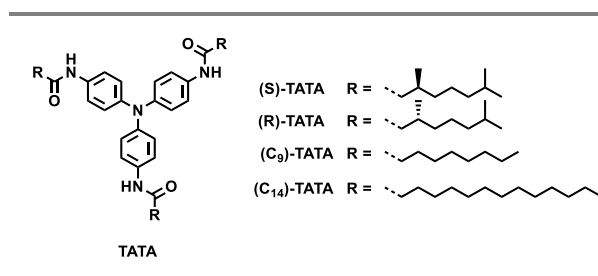
Figure 32 | Molecular structures of C_3 -symmetrical TATAs, bearing different alkyl substituents.
