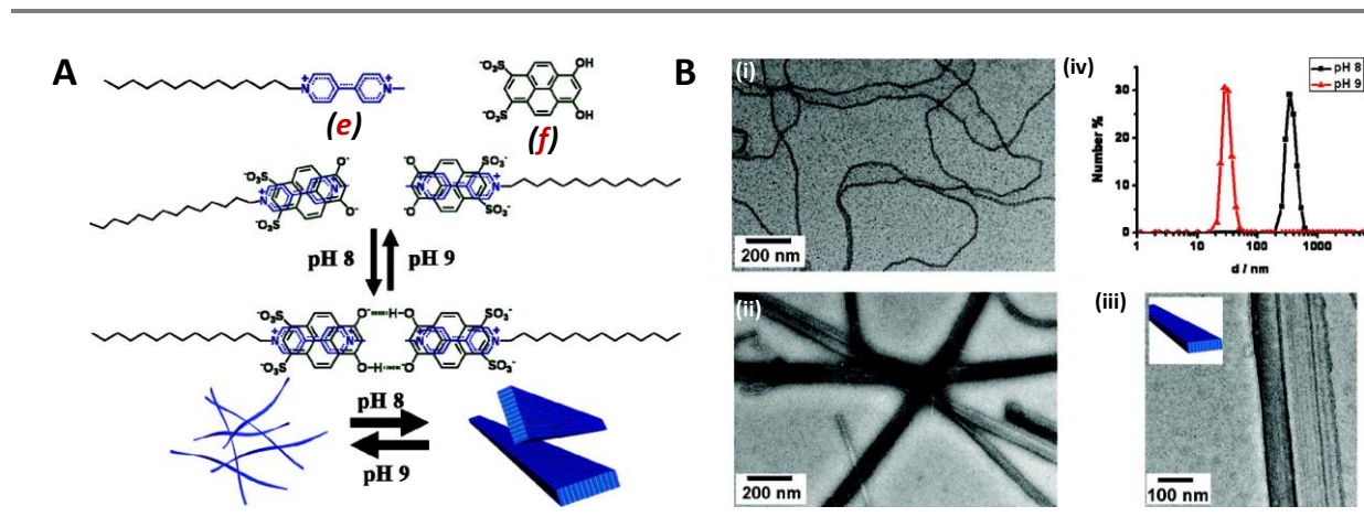
Figure 5 | (A) Schematic illustration of the hierarchical nanoribbons self-assembly of aromatic amphiphiles. (B) TEM images of the aggregates of ( e-f ) at pH 9 (i). (ii and iii) Magnified TEM images of the aggregates at pH 8. (iv) Distribution of the hydrodynamic diameter of ( e-f ) at pH 9 and pH 8. Figure is adapted from ref. 20
