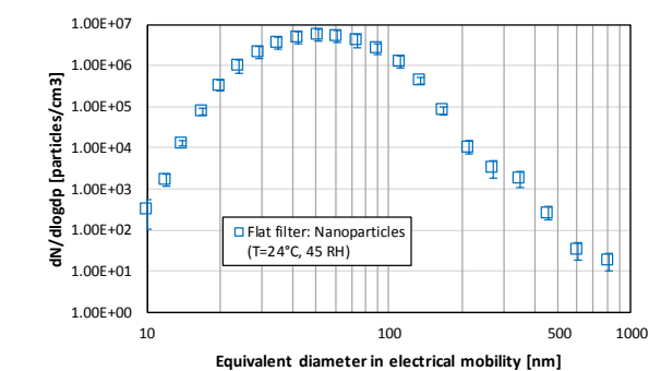
c) Upstream of flat filter T=24^\circ\text{C} , \text{RH}=45\%
