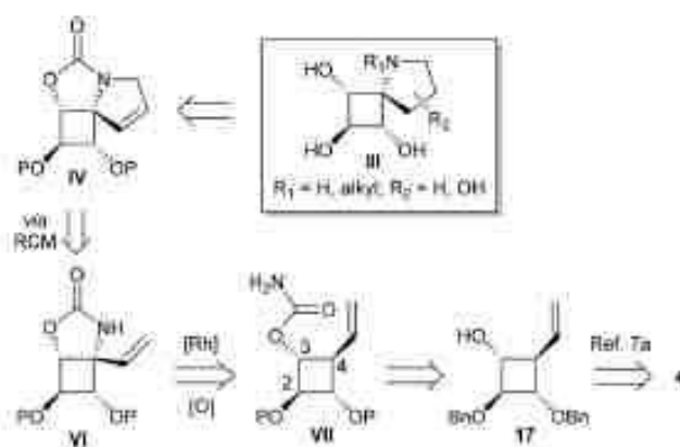
Fig. 4 Retrosynthetic analysis towards azaspiro[3.4]octane derivatives.
