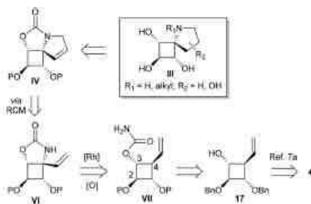
Fig. 4 Retrosynthetic analysis towards azaspiro[3.4]octane derivatives.
