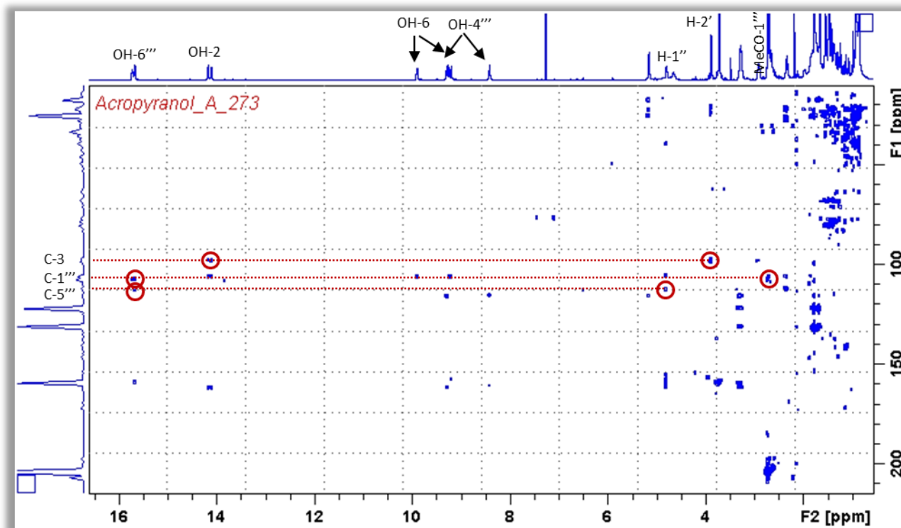
Figure A 20: HMBC (600 MHz, \text{CDCl}_3 , 0 °C) spectrum of Acropyranol A (2)
