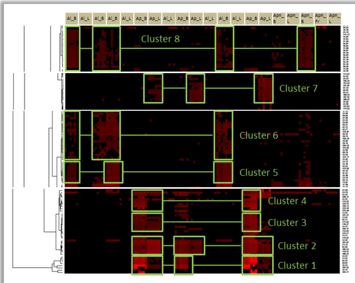
Figure 45: ^{13}\text{C} NMR chemical shift clusters revealed after HCA of the ^{13}\text{C} NMR data obtained from different Acronychia samples, particularly A. laurifolia barks are abbreviated as Al_B, A. laurifolia leaves as Al_L, A. porteri barks as Ap_B, A. porteri leaves as Ap_L, A. pedunculata barks as Apn_B, A. pedunculata fruits as Apn_Fr and A. pedunculata leaves as Apn_L
