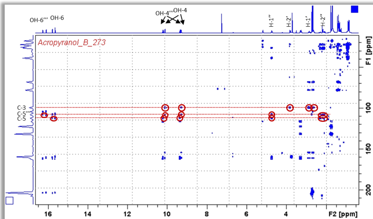
Figure A 28: HMBC (600 MHz, \text{CDCl}_3 , 0 °C) spectrum of Acropyranol B (3)
