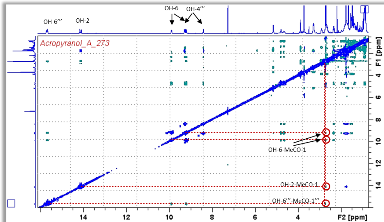
Figure A 19: NOESY (600 MHz, \text{CDCl}_3 , 0 °C) spectrum of Acropyranol A (2)
