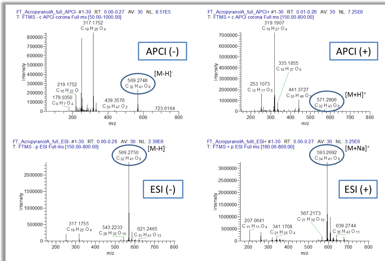
Figure A 71: Full scan mass spectra of acropyranoI A (5) in APCI (±) and ESI (±); molecular and adduct ions are highlighted
