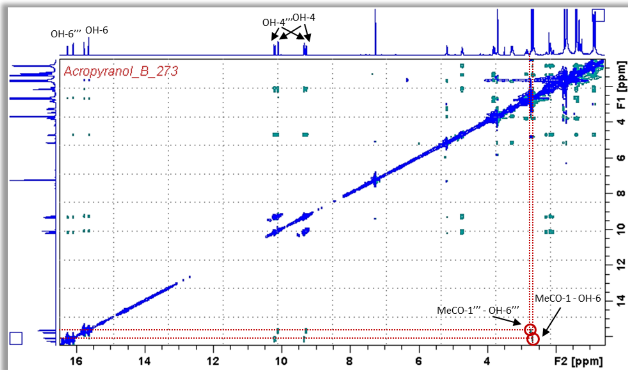
Figure A 27: NOESY (600 MHz, \text{CDCl}_3 , 0 °C) spectrum of Acropyranol B (3)
