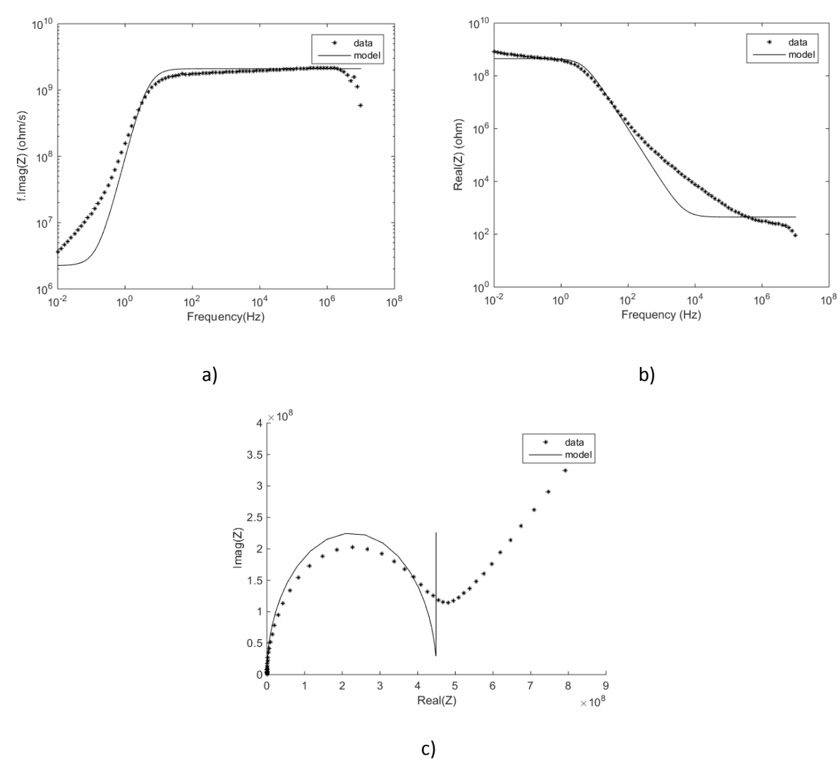
Figure 14: Impedance spectroscopy of the electrophoretic cell, the surface is 1.0 cm 2 and the thickness is 50µm. a) The imaginary part ( -Z_{Im} ) versus f b) The real part ( Z_{Re} ) versus f c) The Nyquist plot ( -Z_{Im} versus Z_{Re} )
