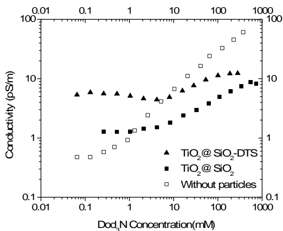
Figure S2.1. Conductivity of pigments TiO 2 @SiO 2 (filled squares), TiO 2 @SiO 2 -DTS (filled triangles), Dod 3 N (empty squares). Given error bars are smaller than 0.01 pS/m.
