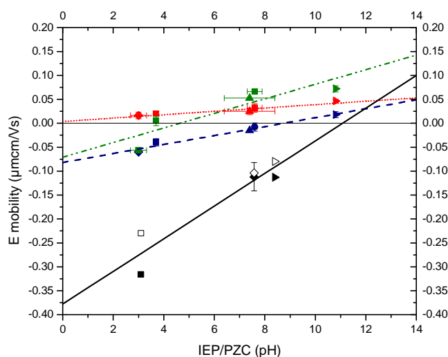
Figure 3. Charging of mineral oxide series: the zero-field electrophoretic mobility. Hydrophilic pigments silica (◆), titania(■), alumine (▲) , zinc oxide,(●)and magnesia(▶)particles dispersed in Isopar L is plotted against their aqueous PZCs. Hydrophobic pigments of TiO_2@SiO_2 (□), TiO_2 (◇) and Fe_2O_3 (▷) with OTS (filled) or DTS groups (empty). The green symbols ( - - - - - ), red ( ..... ), blue ( - - - - - ) slopes represent respectively particles dispersed with AOT, Span 80, OLOA 11000. The solid black slope( _____ ) represents hydrophobic pigments and charged with Dod_3N . Values for hydrophilic pigments were reported from the review of Berg et al. [34] The horizontal straight line corresponds to the zero mobility.
