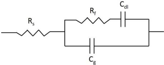
Figure 13: The equivalent circuit used for the electrophoretic cell
