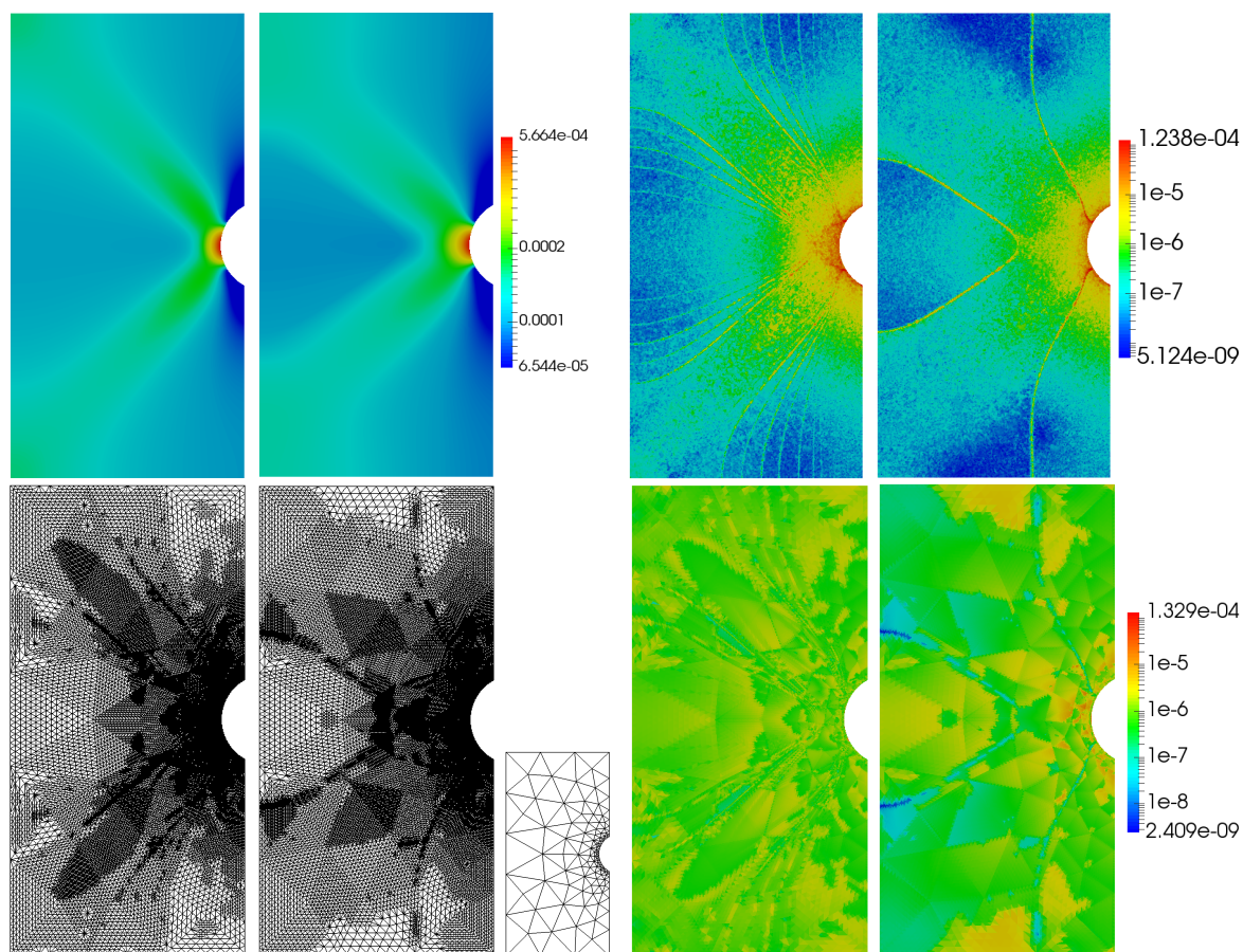
Figure 3.6 – Notched specimen plate, comparison between Hencky–Mises (left in each picture) and damage model (right). Top left: \text{tr}(\underline{\nabla}_s \underline{u}_h) . Top right: \eta_{\text{disc}} on a fine mesh (no adaptive refinement). Bottom left: meshes after six adaptive refinements. Bottom middle: initial mesh. Bottom right: \eta_{\text{disc}} on the adaptively refined meshes.
