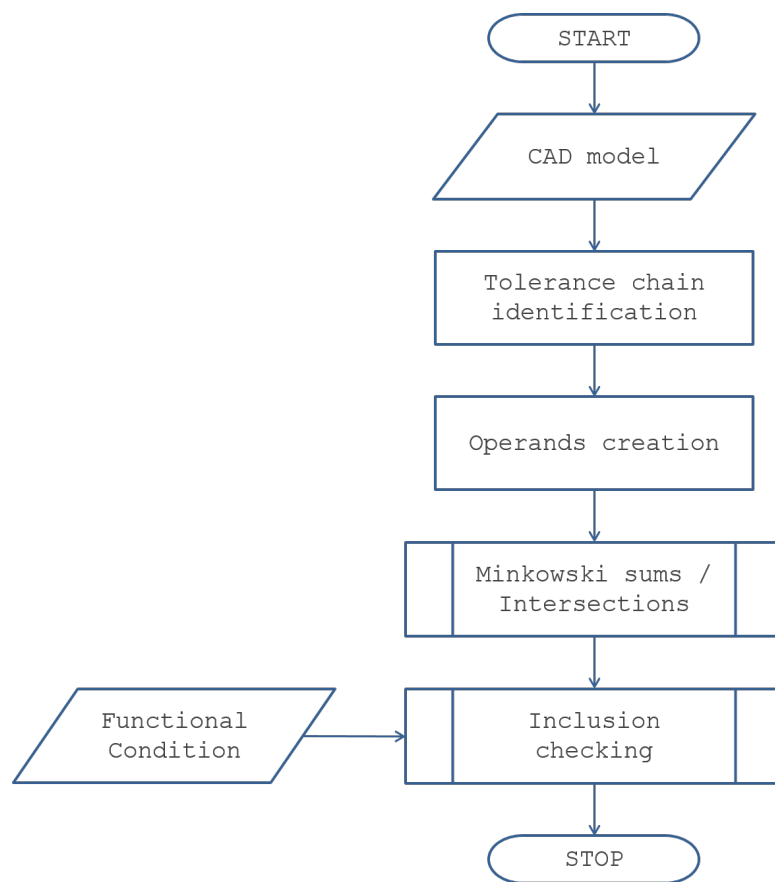
Figure 2.18: Flowchart of the current methodology for tolerance analysis with polytopes.
