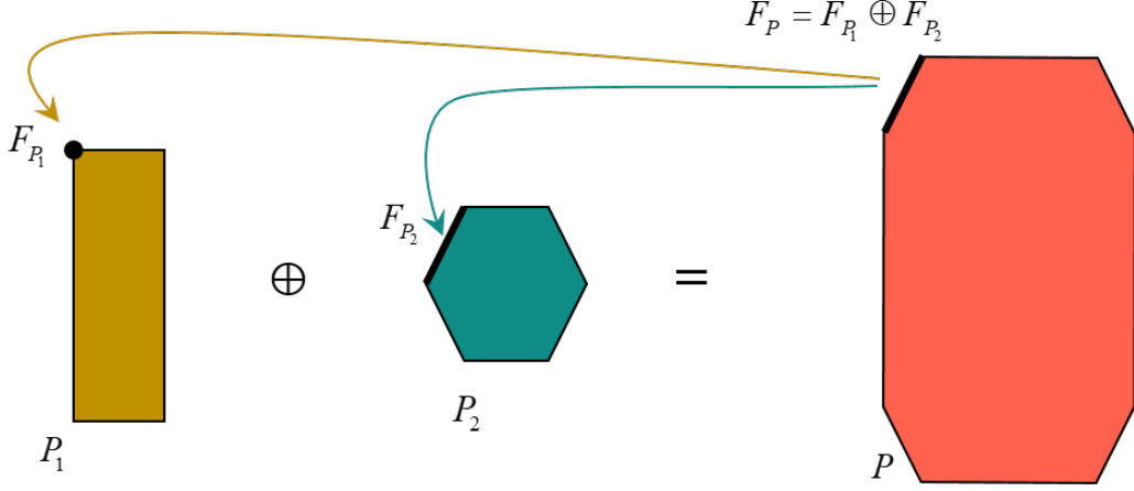
Figure 3.3: Faces decomposition in Minkowski sums.
