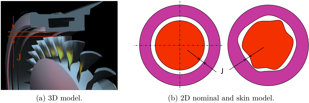
Figure 1.3: Functional requirement in a turboshaft engine (Pierre, 2011).
