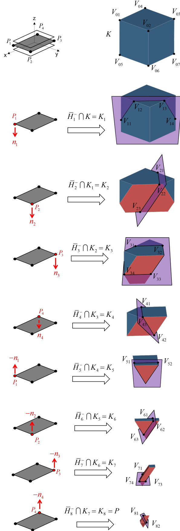
Figure 2.15: Example of the truncation process (Arroyave-Tobón et al., 2017c).
