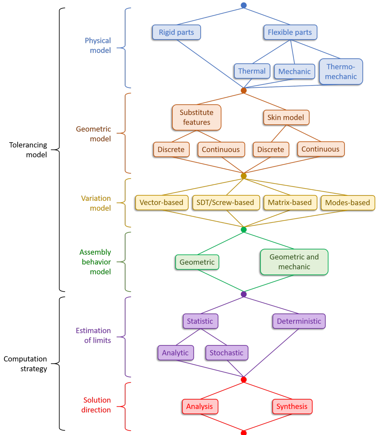
Figure 1.2: Map of geometric tolerancing approaches.
