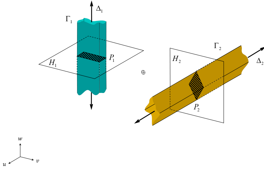
(a) Step 1: polyhedra decomposition.
