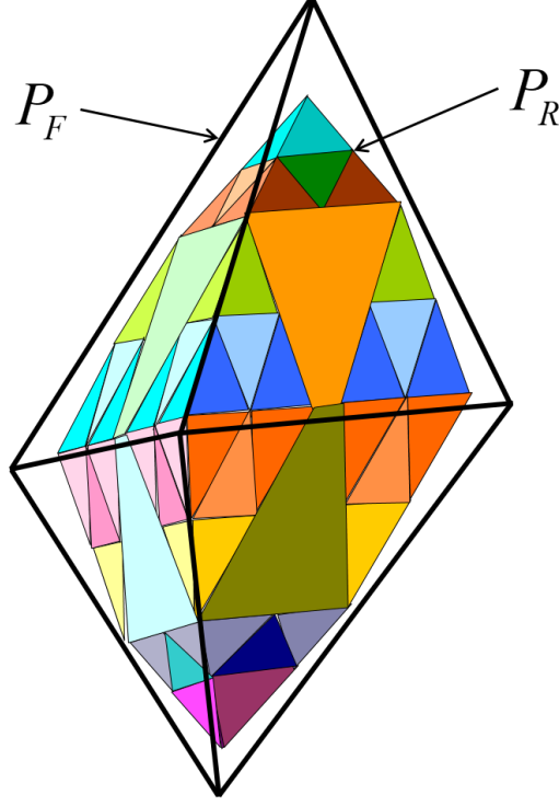
Figure 2.13: Polytopes inclusion test (Teissandier, 2012).
