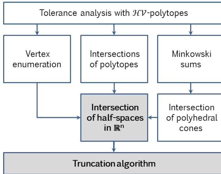
Figure 2.17: Truncation algorithm in tolerance analysis (Arroyave-Tobón et al., 2017c).
