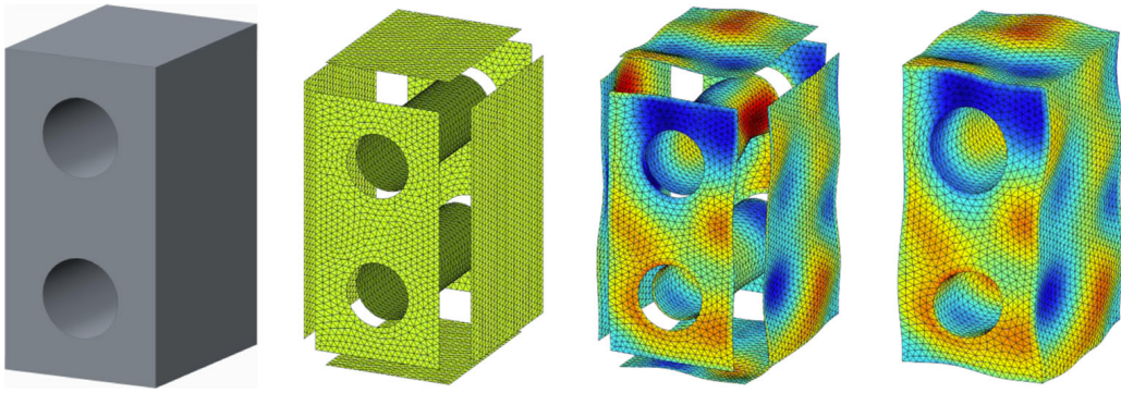
Figure 1.4: Skin model shape generation (Yan and Ballu, 2017).
