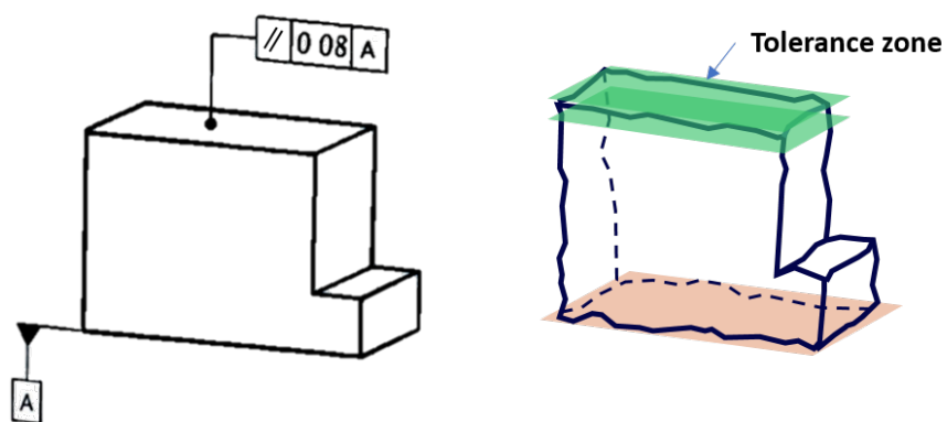
(c) Parallelism specification.
