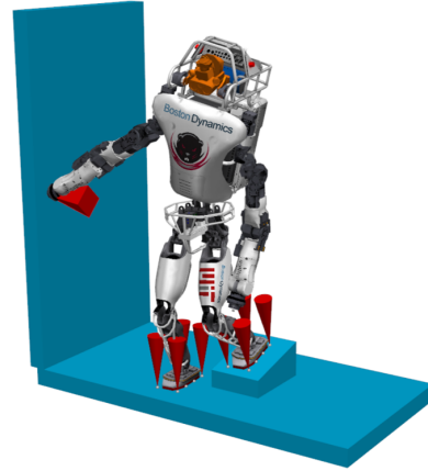
(b) Polyhedral cones representing reaction forces (Dai, 2016).
