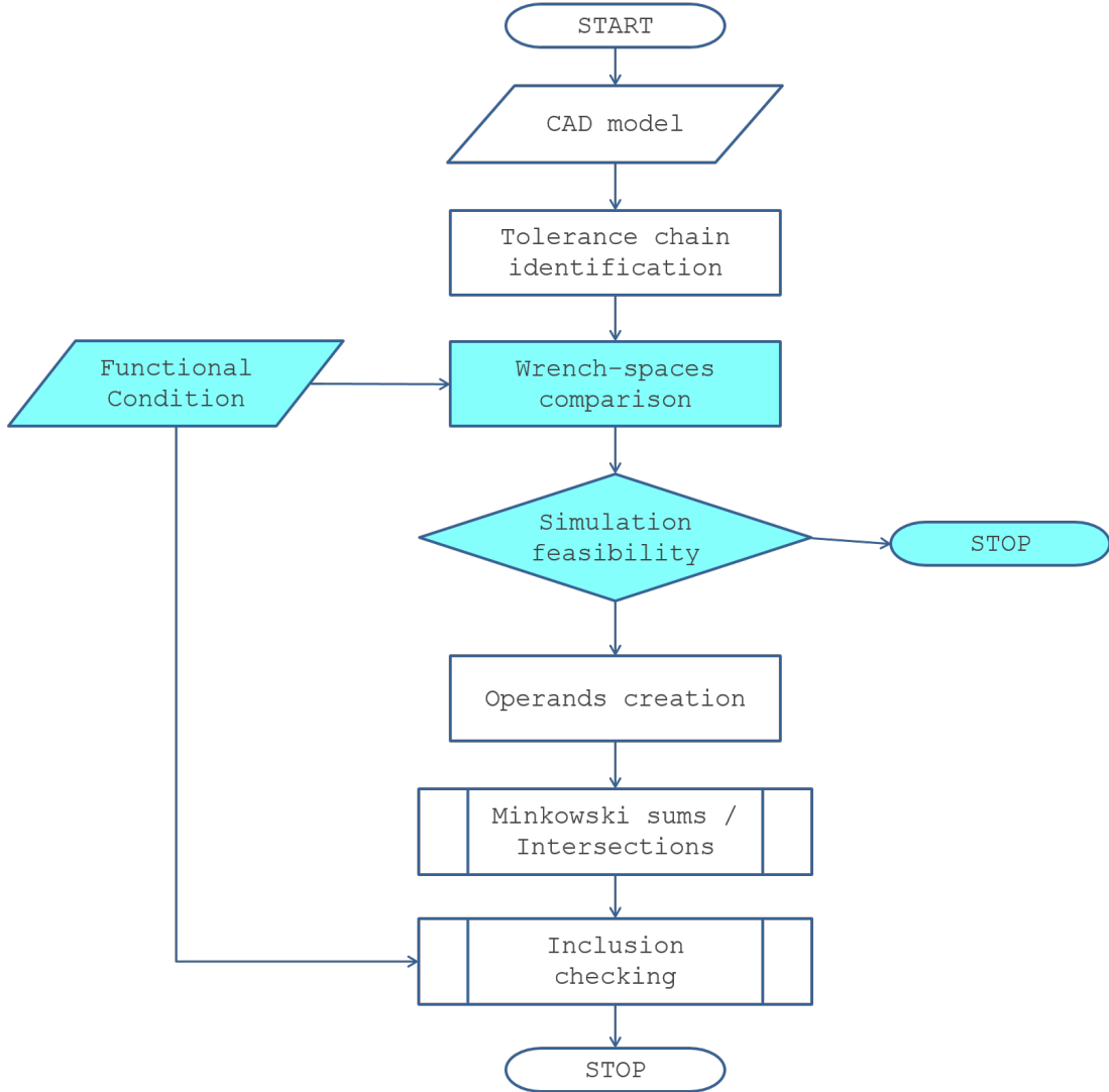
Figure 4.9: Flowchart of the proposed methodology considering the simulation feasibility.
