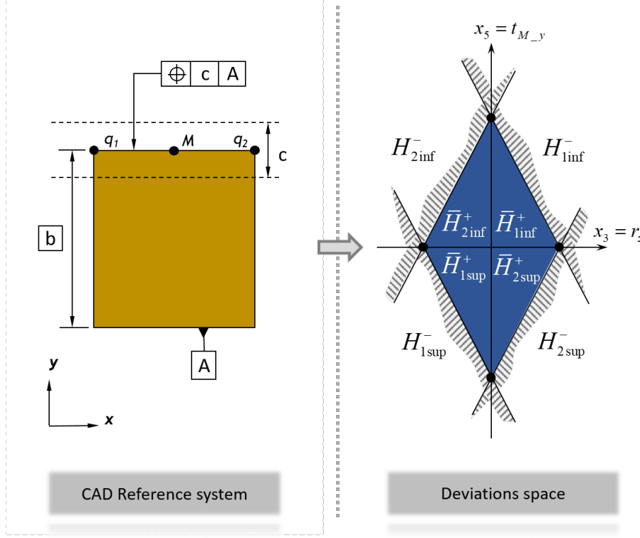
Figure 2.4: A polytope representing geometric deviations in 2D.
