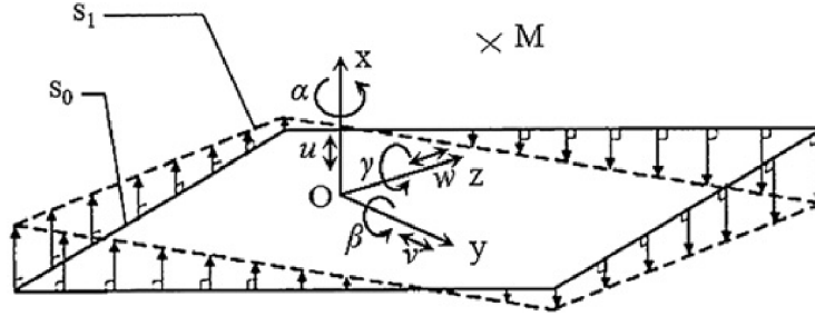
Figure 1.8: Rotation linearization (Chen et al., 2014).
