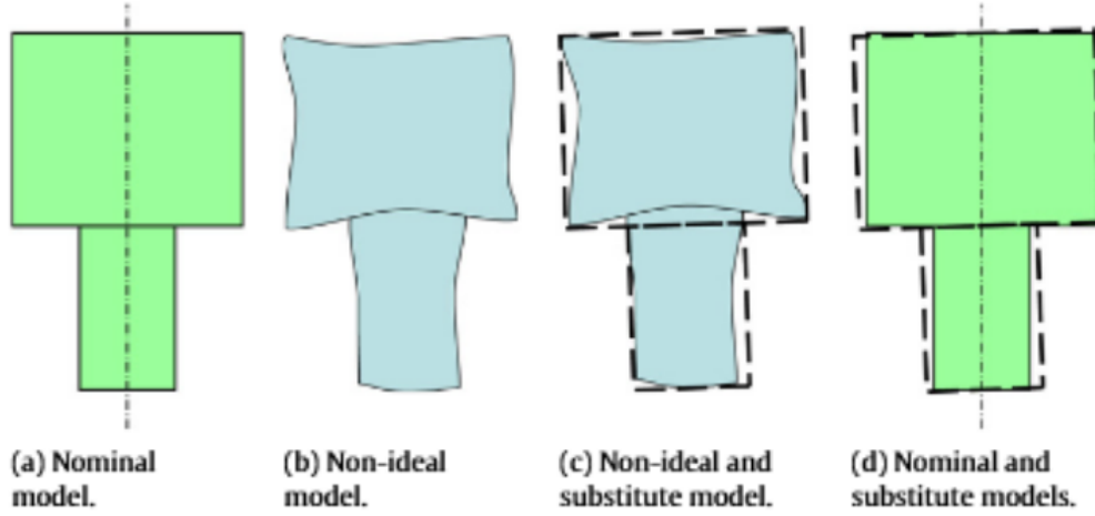
Figure 1.6: Substitute surface association (Dantan and Qureshi, 2009).
