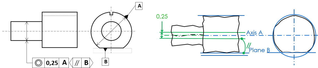
(a) Coaxiality specification.
