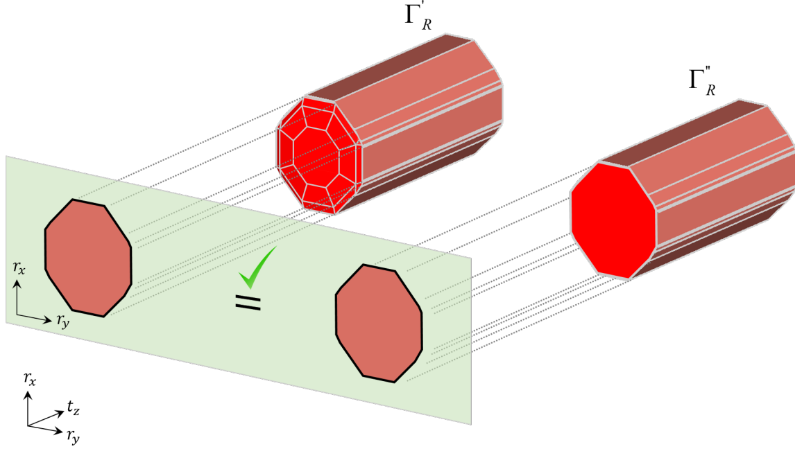
Figure 3.10: Comparison of the results of the simulation without (at the left-hand side) and with caps removal (at the right-hand side).
