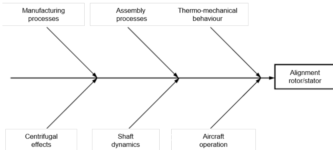
Figure 1.1: Phenomena causing geometric deviations in a turboshaft engine (Pierre, 2011).
