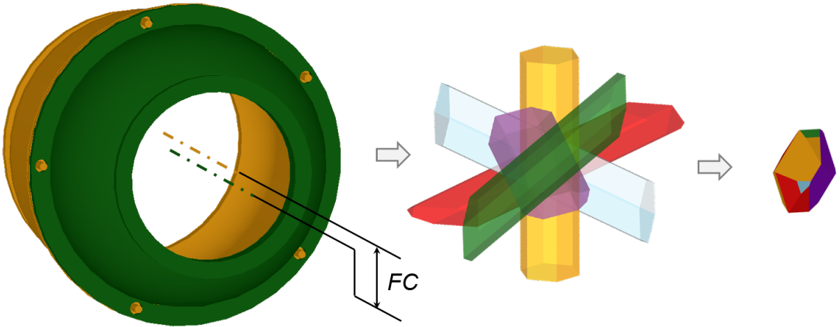
Figure 2.7: Modelling stack-up of deviations as the intersection of polyhedra (Gouyou et al., 2016).
