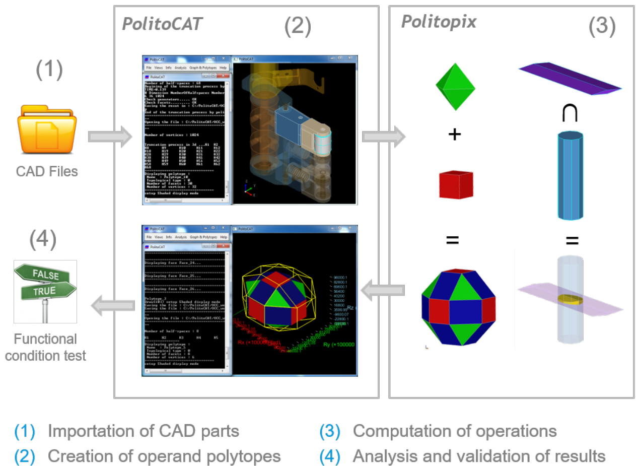
Figure 2.19: Tolerance analysis process using PolitoCAT and politopix software tools.
