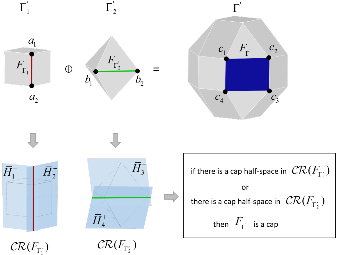
Figure 3.4: Illustration of Algorithm 2.
