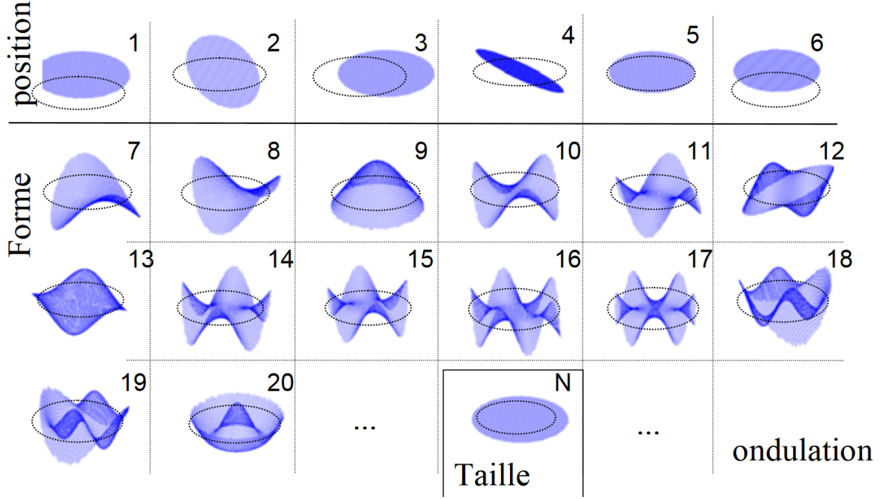
Figure 1.7: Natural modes of a disc (Samper, 2007).
