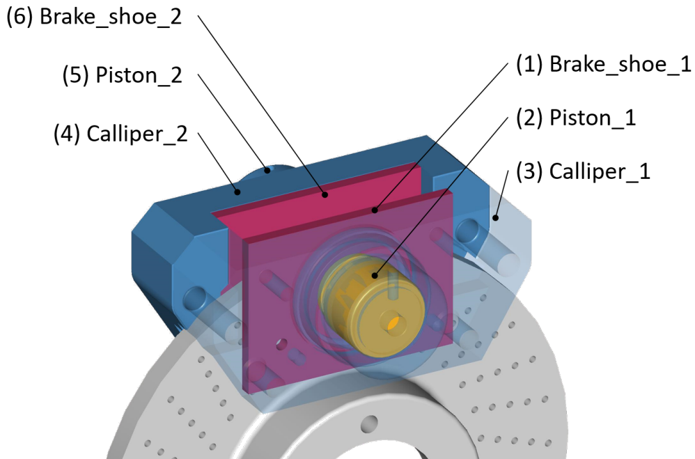
Figure 2.22: Case study: breaking system (Arroyave-Tobón et al., 2017c).
