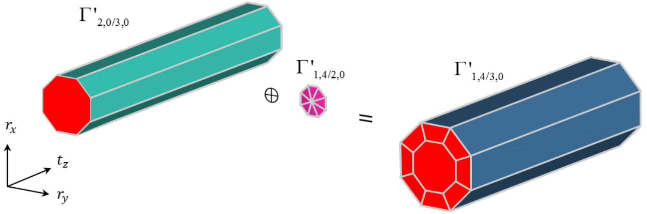
(a) Computation of \Gamma'_{1,4/3,0} .
