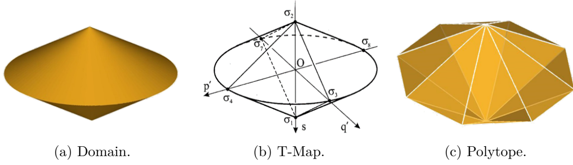
Figure 1.9: Comparison of domains, T-Maps and polytopes.
