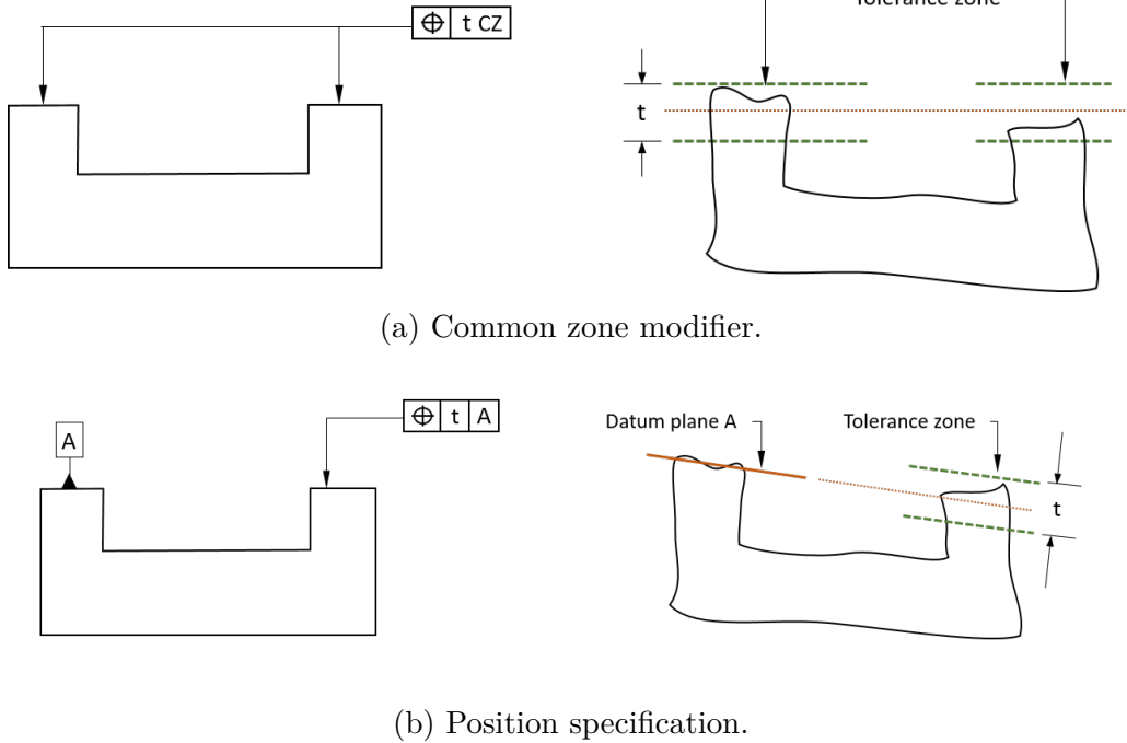
Figure 4.12: Tolerance zone definition with the common zone (CZ) modifier.
