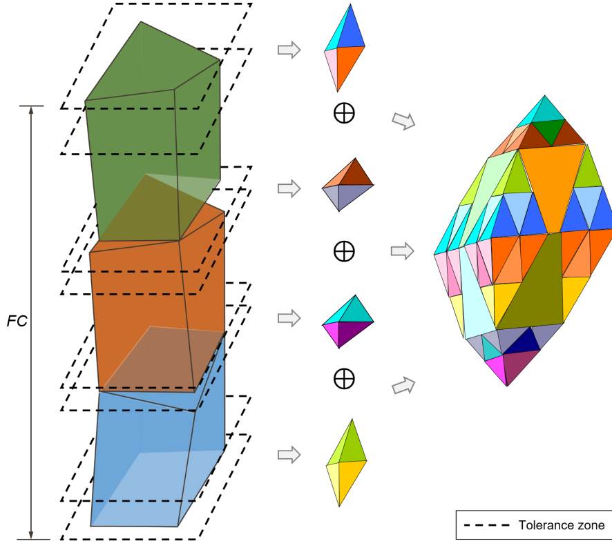
Figure 2.8: Modelling stack-up of deviations as the sum of polytopes.
