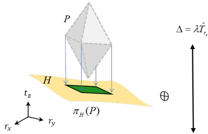
(a) Inclusion of an additional mobility.
