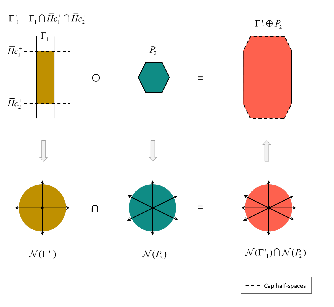
Figure 2.20: Summing 2D capped polytopes intersecting normal fans.
