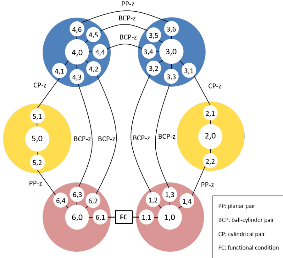
Figure 2.24: Contact graph of the mechanism (Arroyave-Tobón et al., 2017c).
