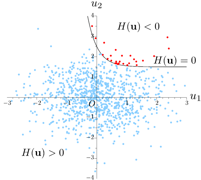
Figure 1.11: Monte Carlo simulation (Dumas, 2014).
