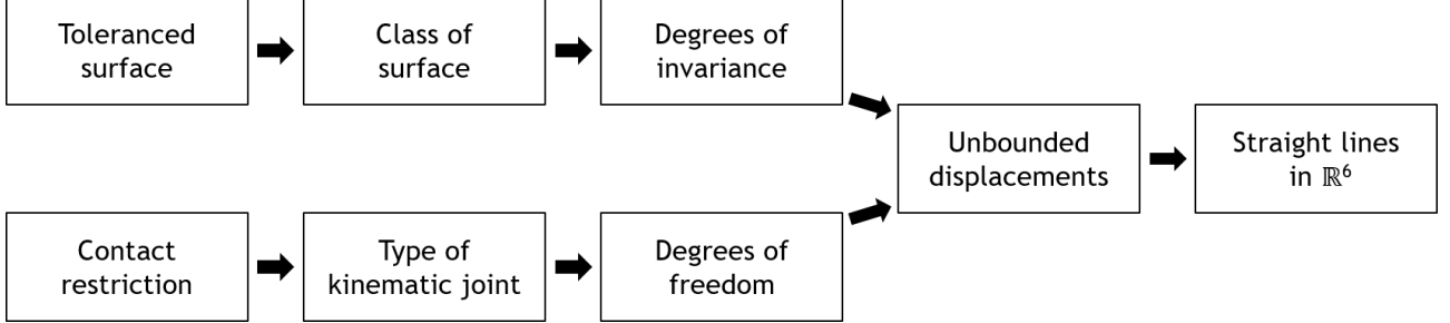
Figure 4.4: Flow chart of the decomposition of polyhedra (Arroyave-Tobón et al., 2017a).
