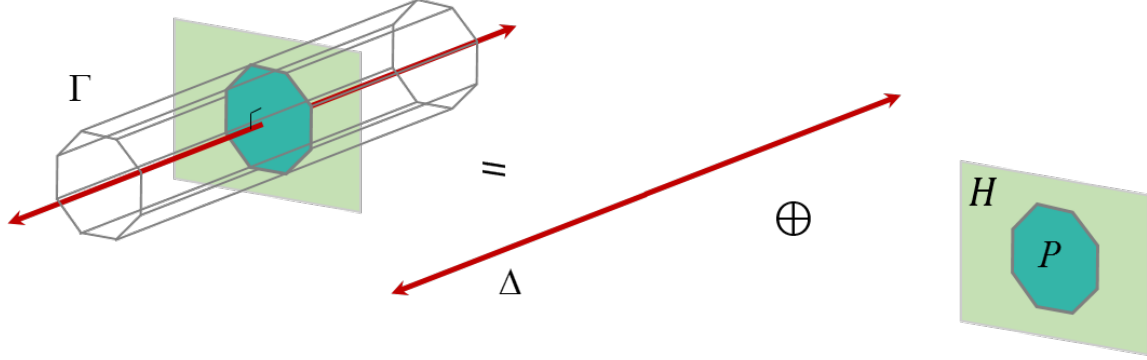
Figure 4.3: Decomposition of a polyhedron into the sum of a polytope and a straight line.
