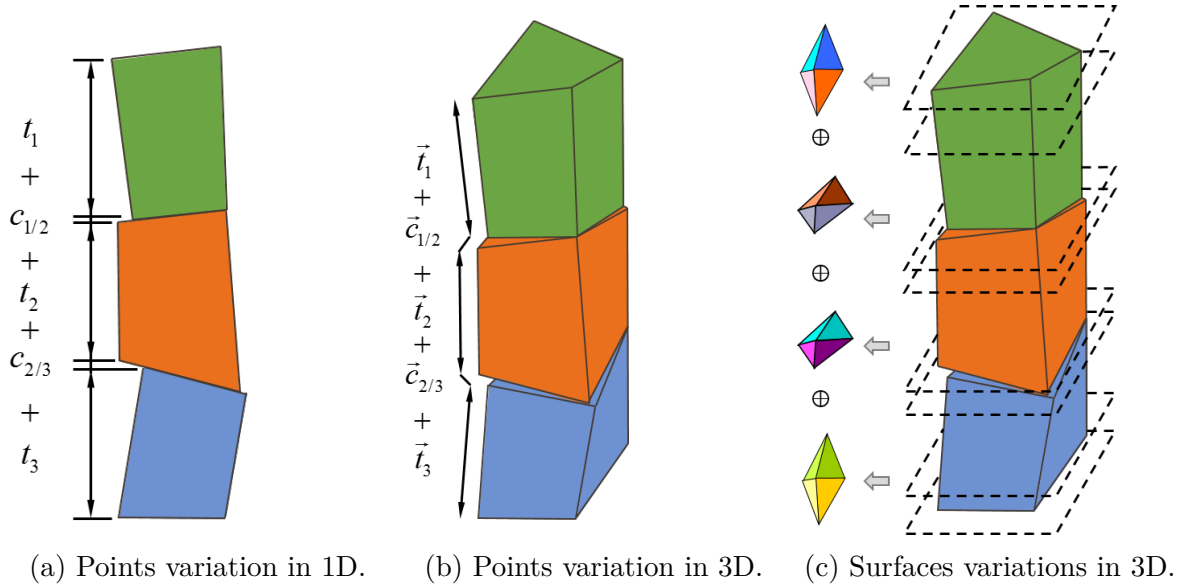
Figure 1.10: Models for representing geometric variations and their accumulation.
