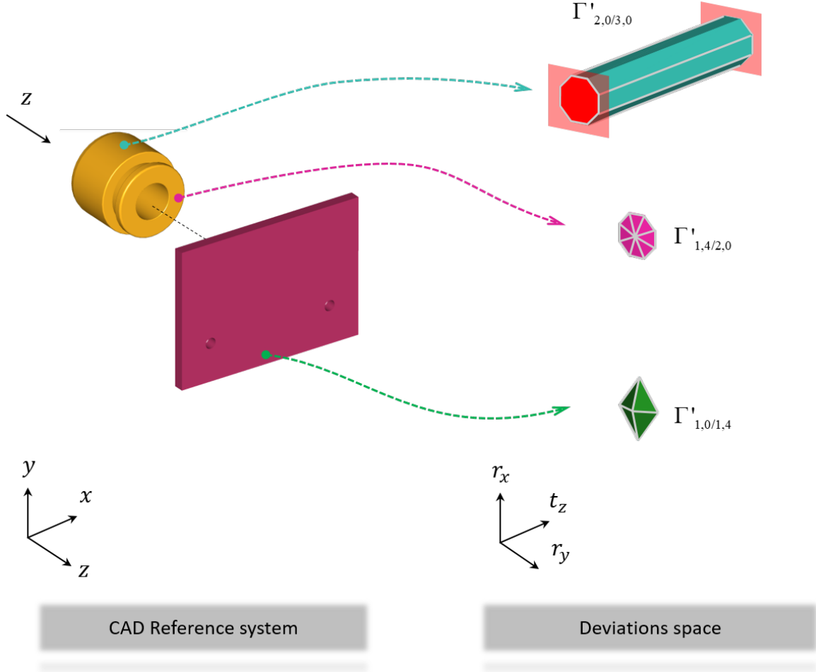
Figure 2.25: 3D representation of some operands. Cap facets are shown in red.
