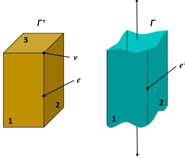
Figure 3.2: Combinatorial representation.
