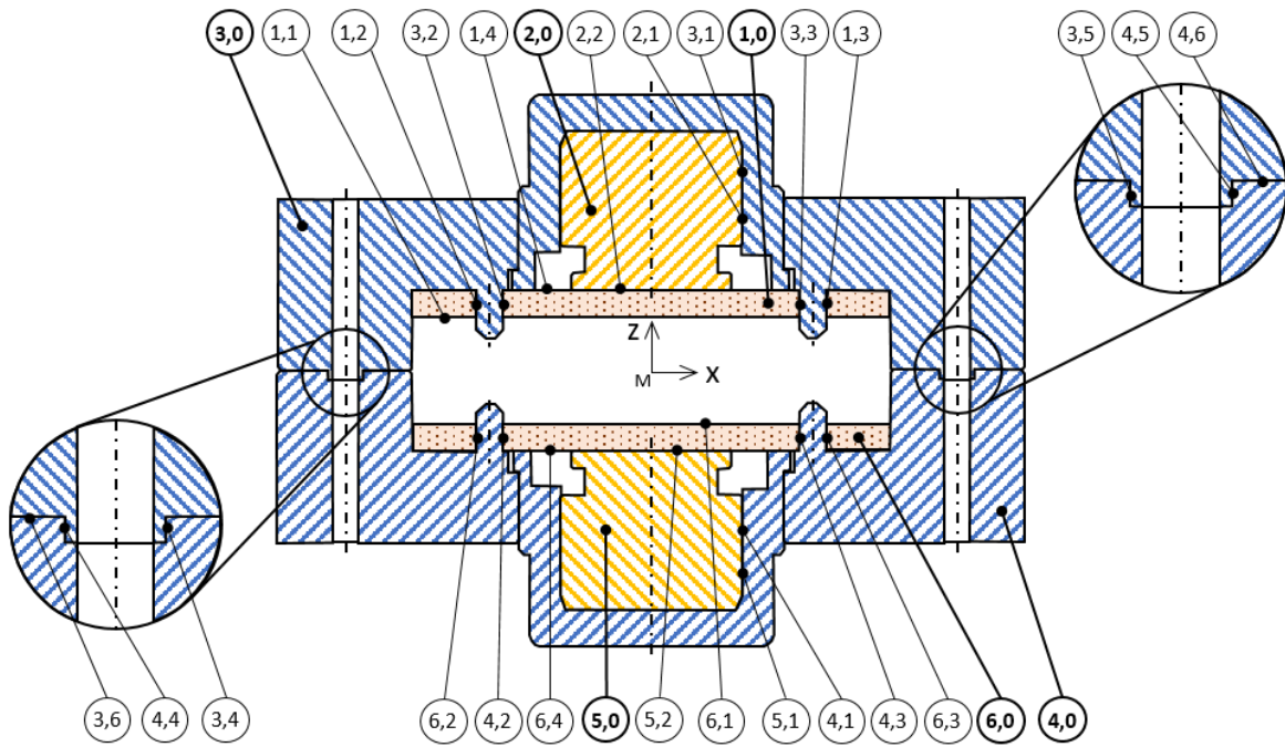
Figure 2.23: Parts and surfaces enumeration (Arroyave-Tobón et al., 2017c).
