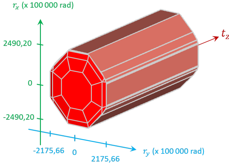
Figure 2.27: 3D representation of \Gamma'_R .
