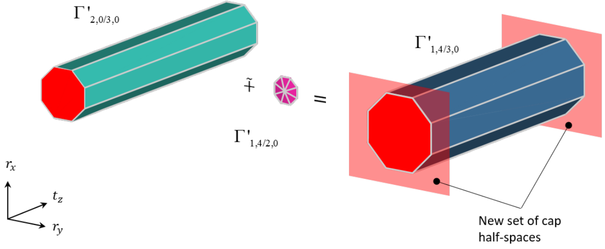
(a) Computation of \Gamma'_{1,4/3,0} .
