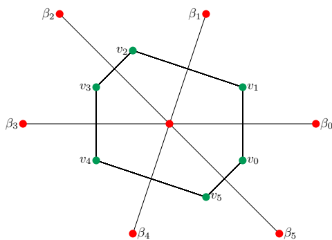
FIGURE 7. The vectors \beta_i and the vertices of the hexagon.
