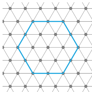
(B) The Cayley graph \tilde{G} .
