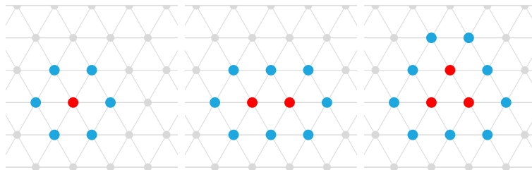
FIGURE 6. The possible cliques and their neighborhoods.
