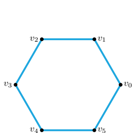
(A) The regular hexagon.
