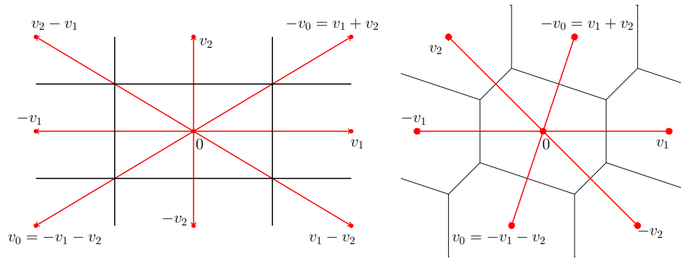
FIGURE 7. The two kinds of parallelehedra in dimension 2.
