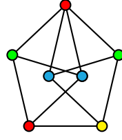
FIGURE 16. \chi(G) = 4 .
