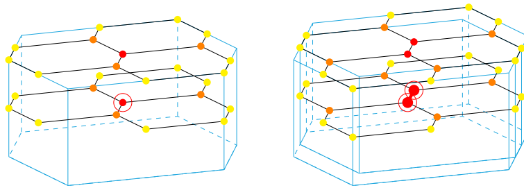
FIGURE 14. For one point in G_{\mathcal{H}} contributing to a clique, there are two points giving the same contribution in G , so that the local density of a clique is reduced by one half. This is the analogue in that situation of Figure 9.
