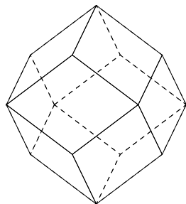
FIGURE 11. The rhombic dodecahedron.
