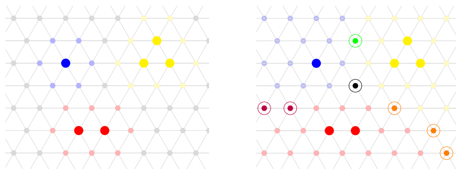
(A) The neighborhoods of the connected components for the function of Example 8, when the auxiliary graph has (Property D). They only contain the neighbors of the connected component in the auxiliary graph \tilde{G} .
