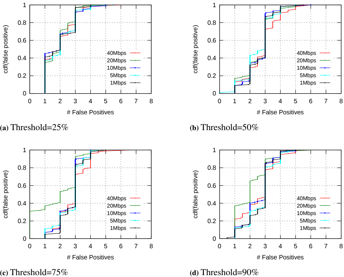
Figure 4.12: Number of false positive detections of segment failures with PortStats.
