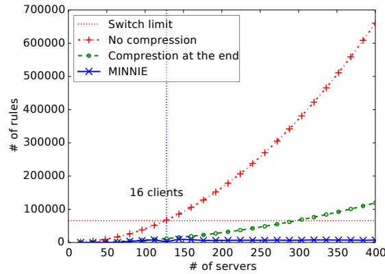
Figure 3.3: Total number of rules installed as a function of the number of servers, in a k = 4 Fat-Tree configuration.
