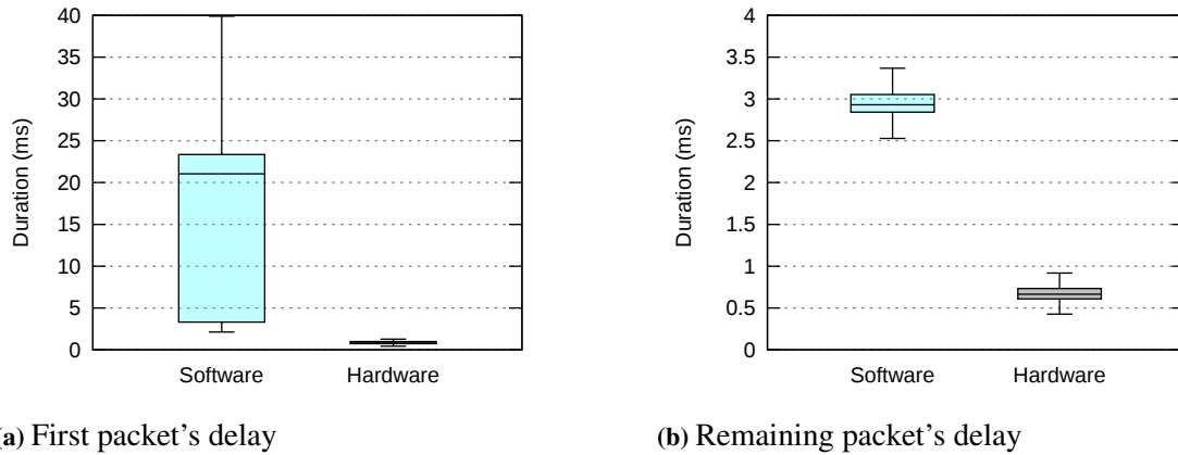
Figure 3.1: Packet delay boxplot
