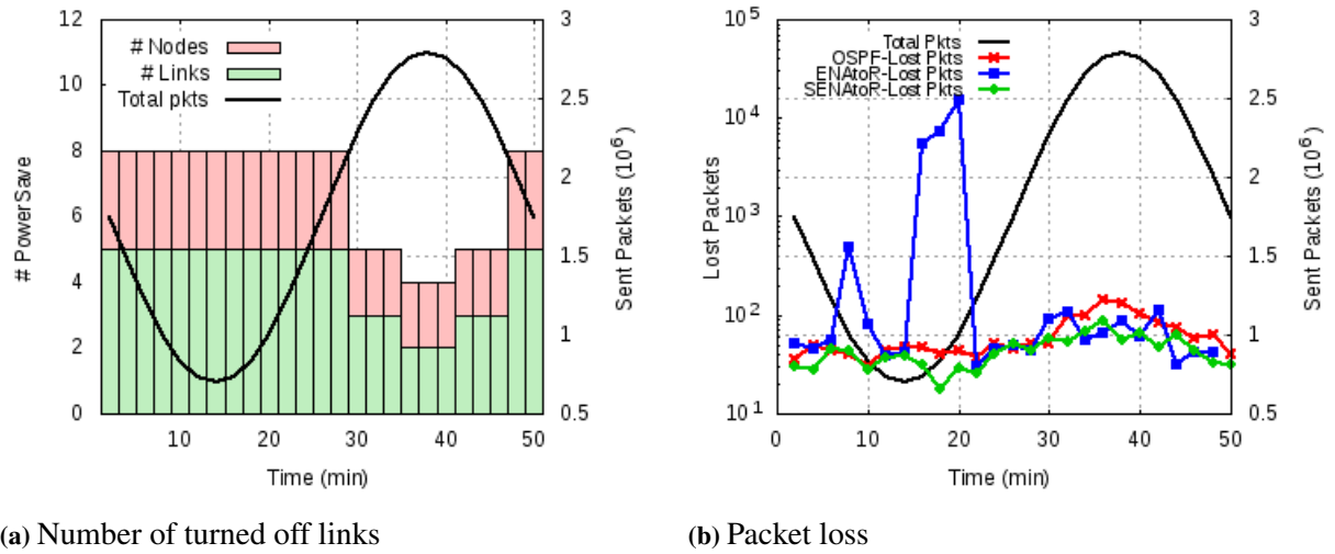
Figure 5.2: Senator impact on atlanta topology using sinusoidal traffic flow.
