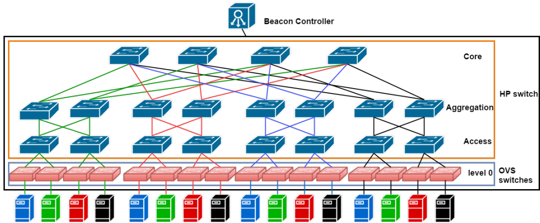
Figure 3.2: Our k=4 Fat-Tree architecture with 16 OvS switches, 8 level 1, 8 level 2, and 4 level 3 switches.
