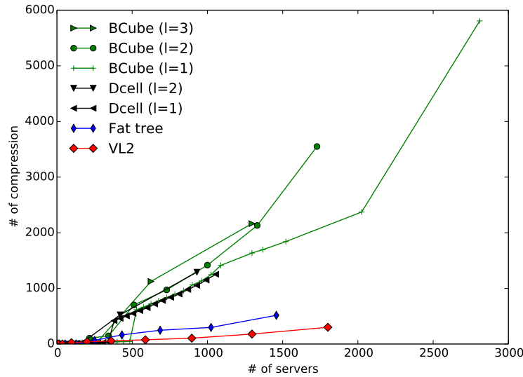
Figure 3.17: Number of compression executed for different topologies
