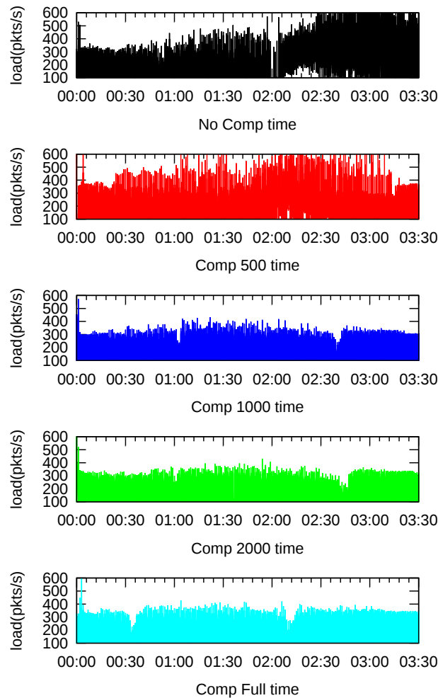
Figure 3.7: Network traffic between the switches and the controller.
