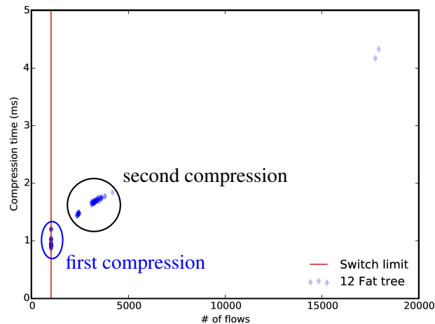
Figure 3.6: Scatter plot of the time to compress a routing table of a k = 12 Fat-Tree.
