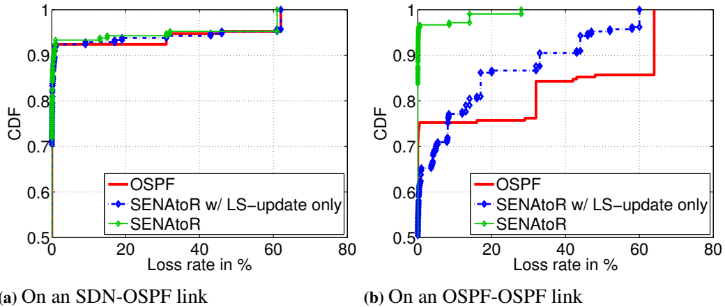
Figure 5.4: Link failure experiment with the atlanta topology
