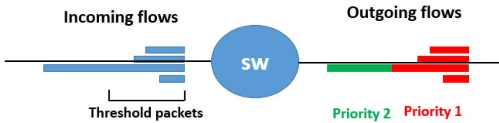
Figure 4.1: State-full scheduler mode of action.
