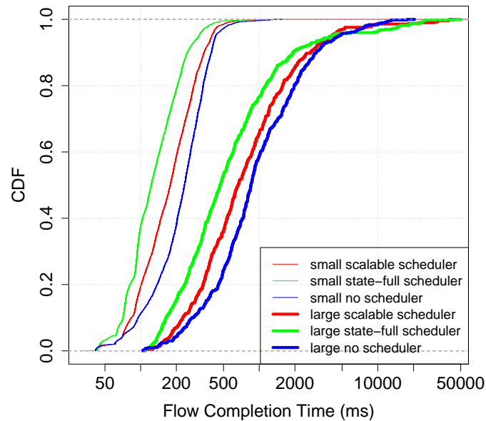
Figure 4.4: Flow completion time CDF for long and short flows
