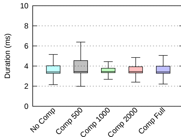
Figure 3.10: Average packet's delay boxplot for packets 2 to 5
