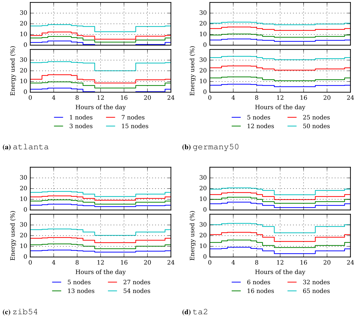
Figure 5.6: Daily energy savings over the day for the (a) atlanta, (b) germany50, (c) zib54 and (d) ta2 networks. with 10, 25, 50 and 100% SDN nodes deployment. Top plots: power model of the HP switch. Bottom plots: power model of an ideal energy efficient SDN switch.
