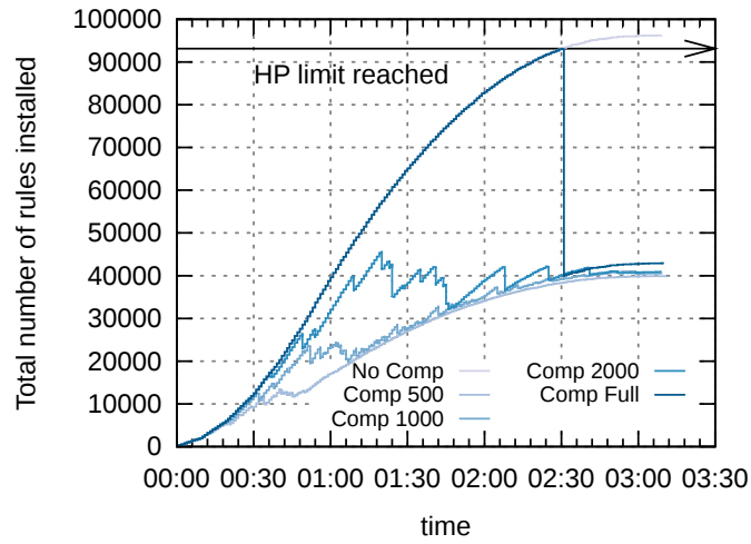
Figure 3.4: Total number of rules installed in the whole network
