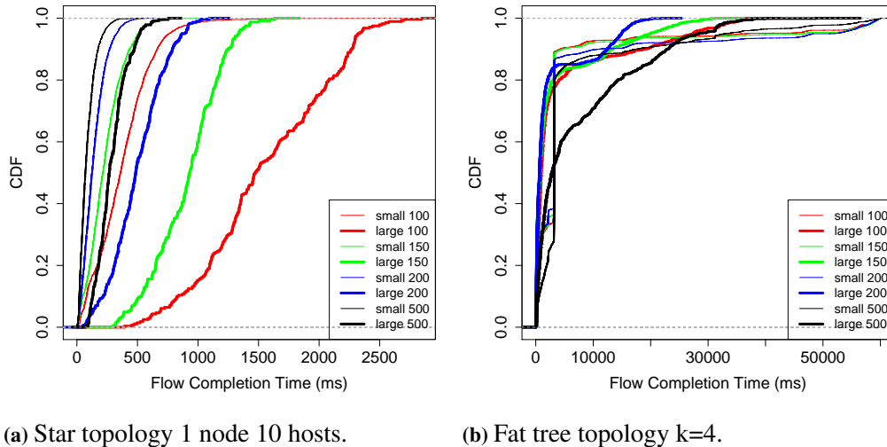
Figure 4.6: Flow completion time with respect to bandwidth transmitted.
