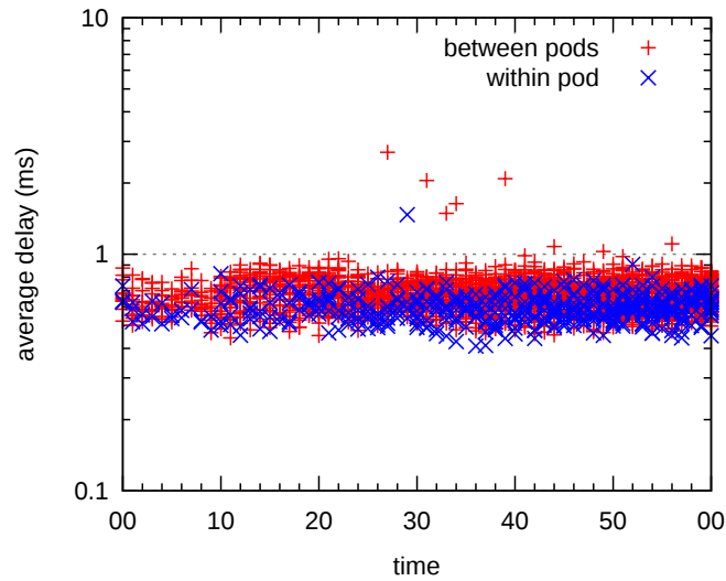
Figure 3.14: High load and hardware rules: Delay of packets 2 to 5 - Compression at 20 entries
