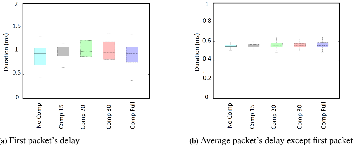
Figure 3.12: Packet delay boxplot under high load
