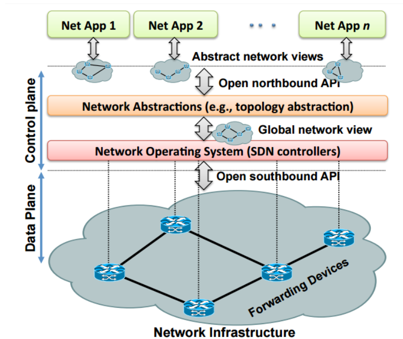
Figure 1.2: SDN network structure. [KREV + 15]
