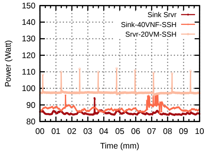
Figure 5.15: Energy consumption of the sink server with VNFs compared to the same server with VMs.
