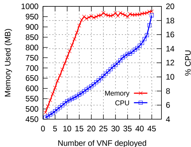
Figure 5.14: RAM and CPU used as a function of number of deployed Apache 2 with PHP module VNF .
