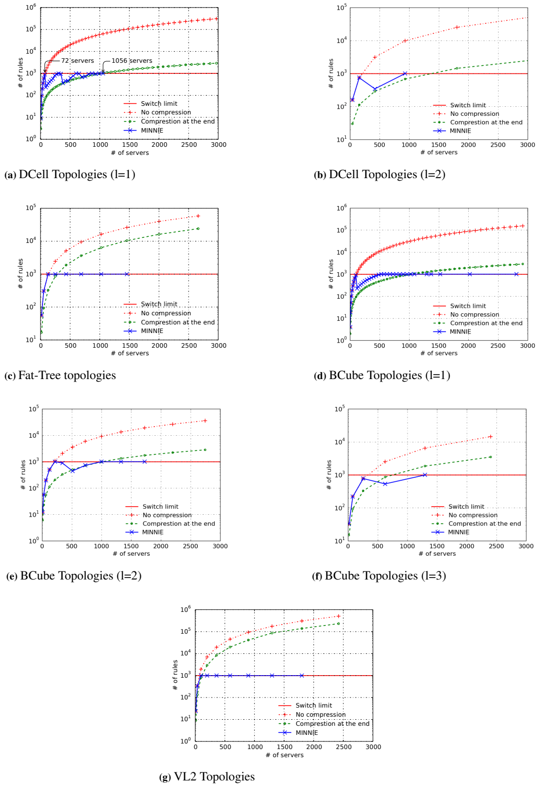
Figure 3.18: Maximum number of rules on a forwarding device as a function of the number of servers for different data center architectures.
