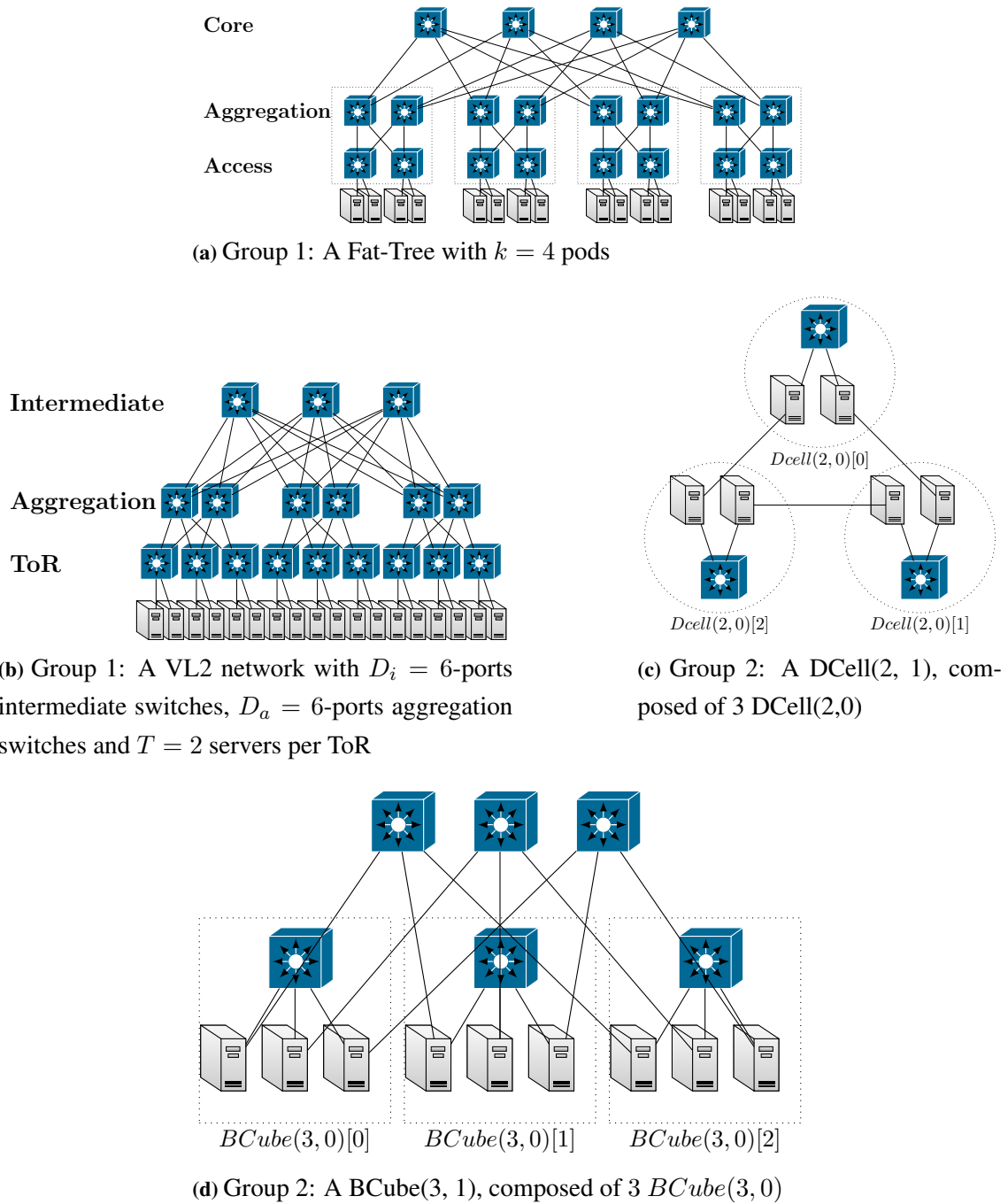
Figure 3.15: Example of topologies studied.
