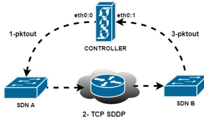
Figure 4.9: Packet_out transmission over the network.
