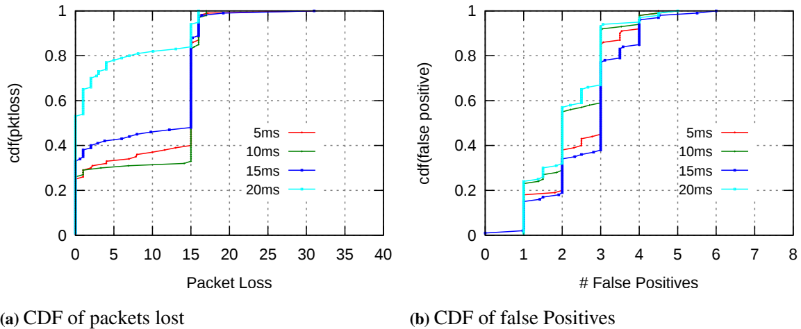
Figure 4.14: Packet loss and false positive variation with the variation of delay on the failed island using PRoPHYS PortStats 50% methodology
