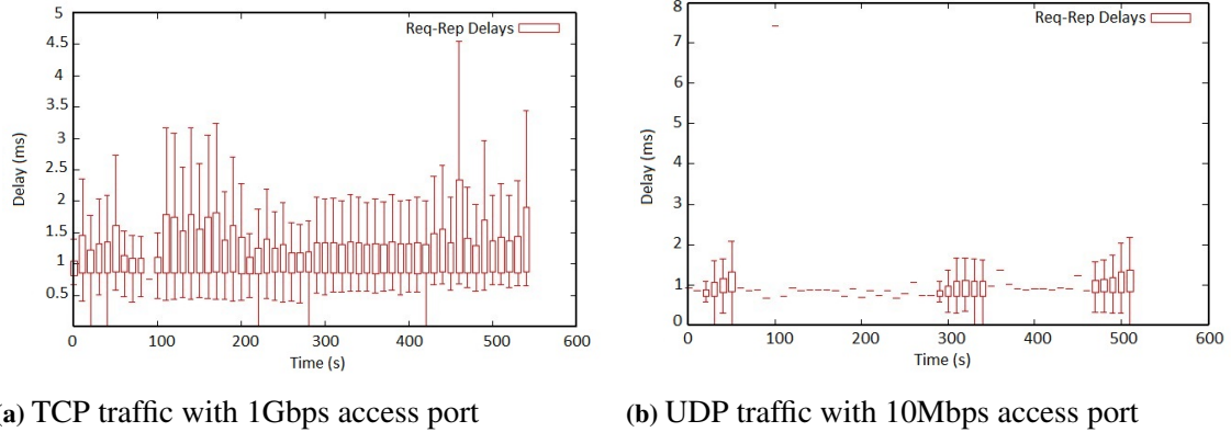
Figure 4.5: Switch response time.
