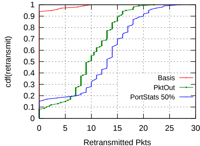
Figure 4.13: Number of packets retransmitted by TCP.
