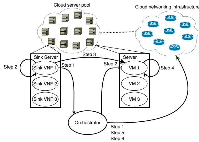
Figure 5.13: Migration procedure from a Sink Server to a working virtual machine
