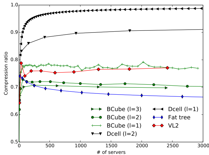
Figure 3.16: Compression ratio for the different topologies in Scenario 2.
