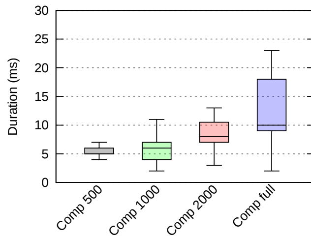
Figure 3.5: Average duration of compression period.
