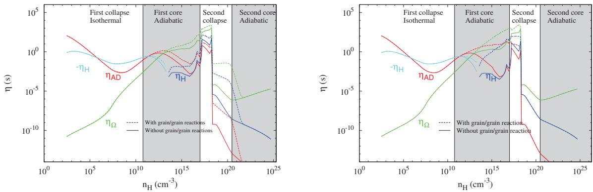
Figure 2.19: Comparison of the resistivities with (dashed lines) and without (solid lines) charge transfer between grains, for 1-charged grains (left figure) and 1 and 2-charged grains (right figure).
