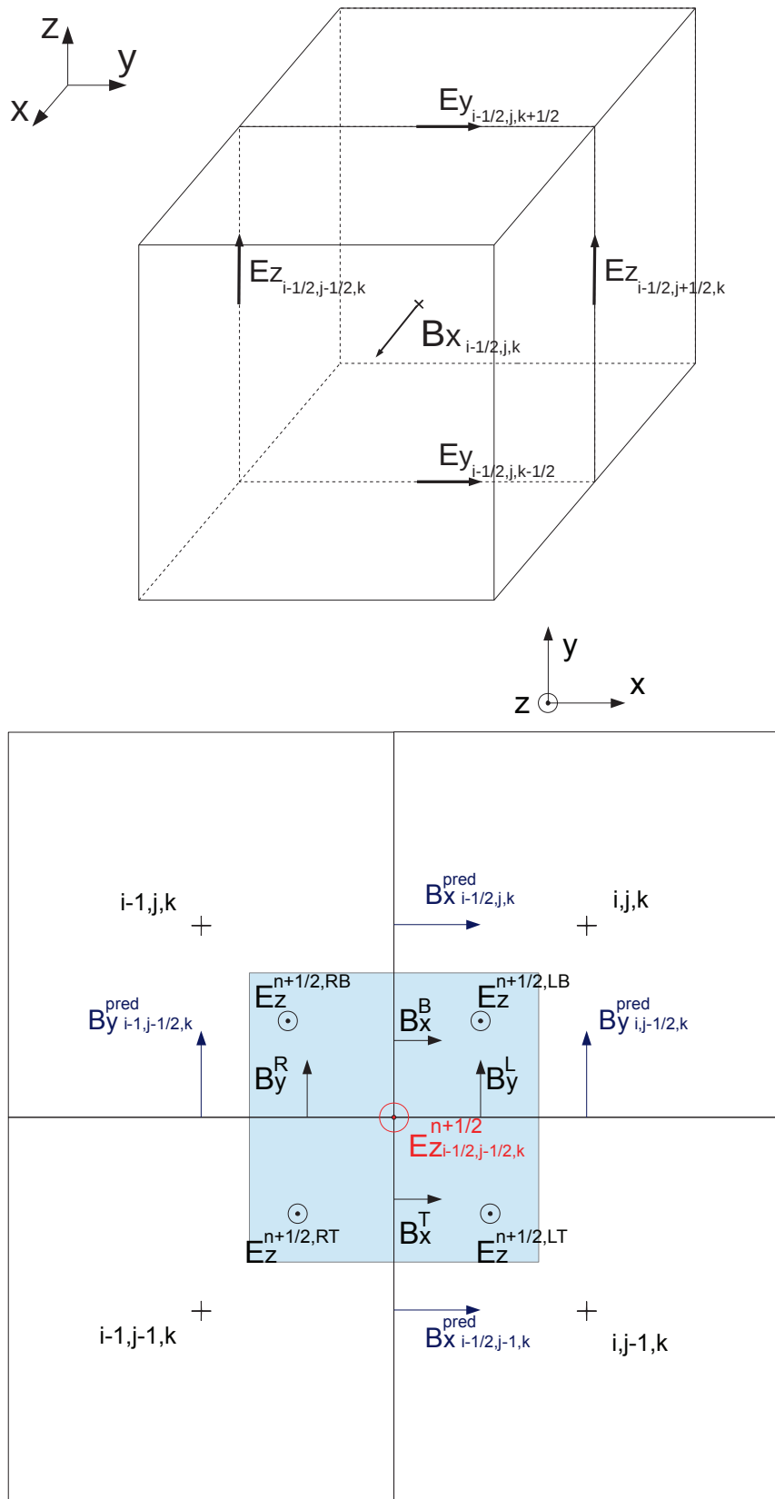
Figure 3.7: Scheme of a 2D Riemann problem in the z -direction. The blue area represents the states at the corner for each cell at i - 1/2, j - 1/2, k .
