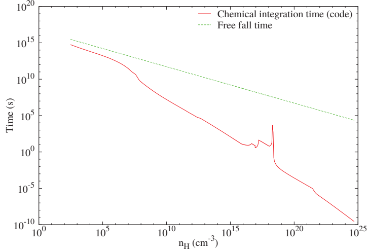
Figure 2.23: Characteristic time for reaching chemical equilibrium (solid red line) and free-fall time (dashed green line) as a function of density.
