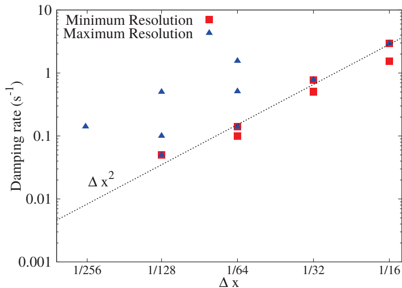
Figure 3.16: Damping coefficient of the whistler wave as a function of the maximum resolution (blue triangles) and minimum resolution (red squares) of the grid. The superimposed points are the regular grids, and the dashed lines represents the least-square fit in \Delta x^2 of the regular grids.
