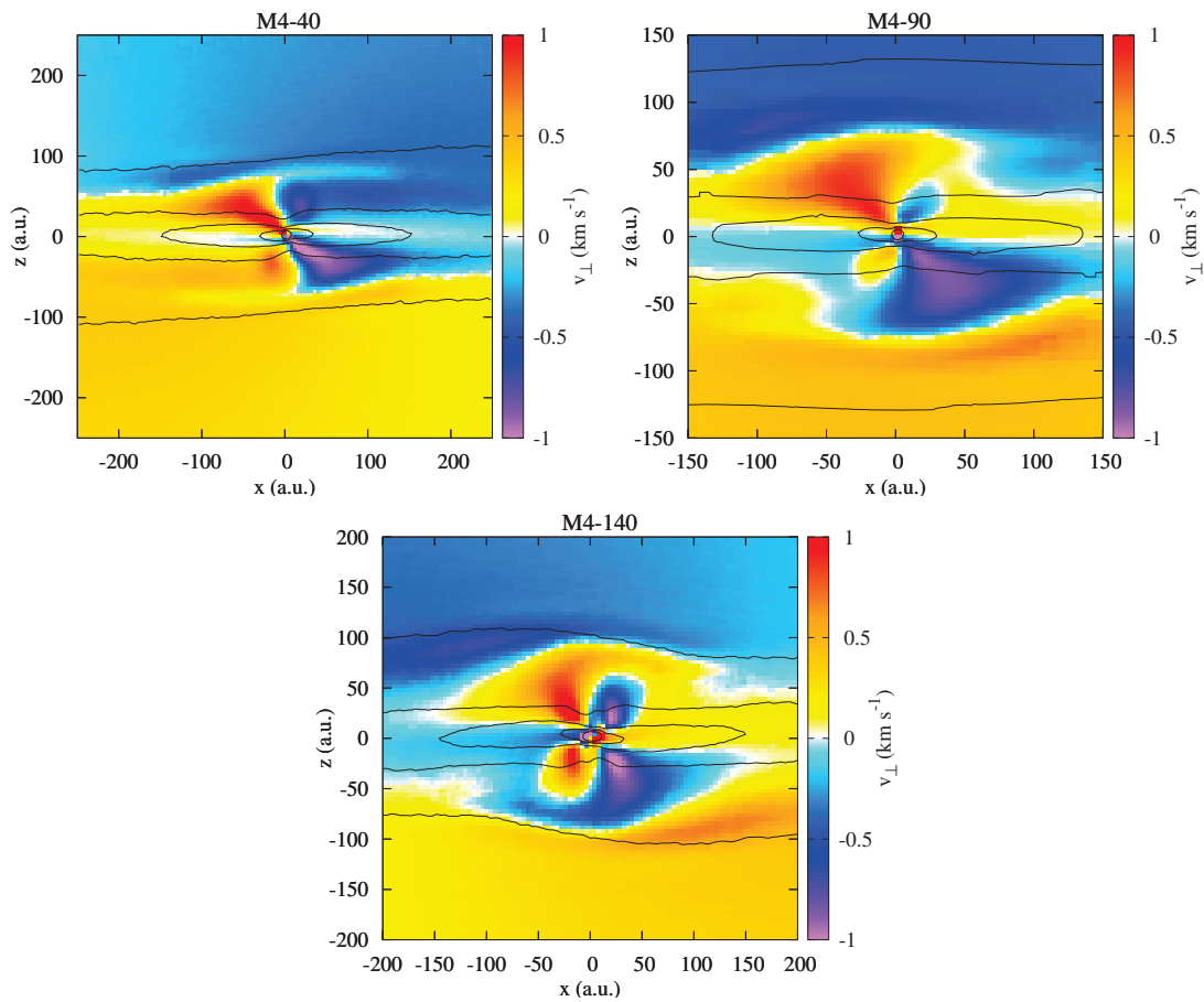
Figure 4.23: Velocity of the fluid coming "out" from the plane (yellow colors) and coming "in" (blue colors) for the tilted setups of \mu = 4 simulations at t = tc + 0.350 kyr. Top left: M4-40, top right: M4-90, bottom: M4-140.
