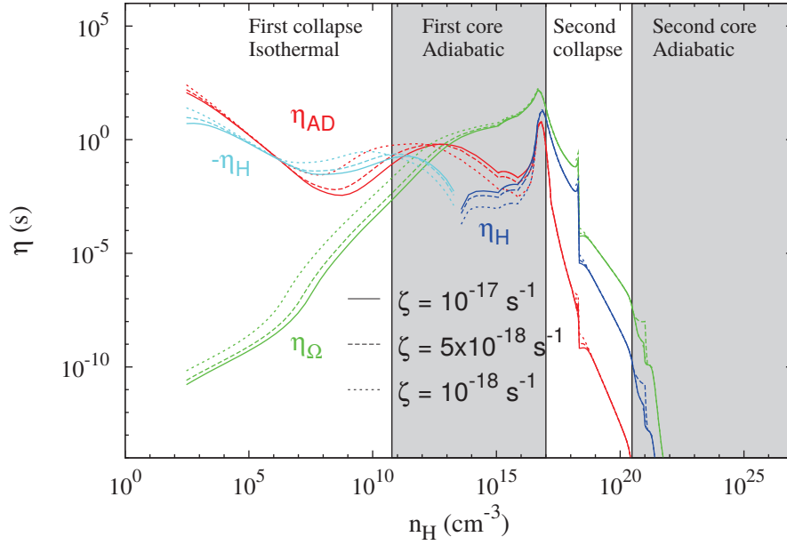
Figure 2.11: Resistivities for different cosmic ray ionisation rates, with the barotropic EOS. Solid lines: fiducial value \zeta_{\text{CR,ref}} = 1 \times 10^{-17} \text{ s}^{-1} . Long dashed lines: \zeta_{\text{CR}} = \frac{\zeta_{\text{CR,ref}}}{2} = 5 \times 10^{-18} \text{ s}^{-1} . Short dashed lines: \zeta_{\text{CR}} = \frac{\zeta_{\text{CR,ref}}}{10} = 1 \times 10^{-18} \text{ s}^{-1} . Same color coding as figure 2.7
