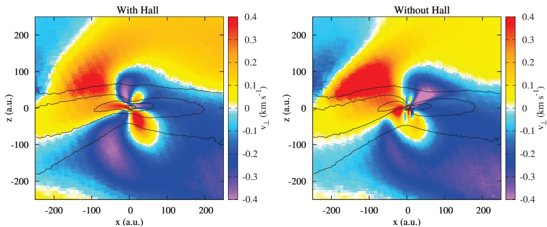
Figure 4.24: Velocity of the fluid coming "out" from the plane (yellow colors) and coming "in" (blue colors) for M4TURB, with and without the Hall effect (left and right panels) t = tc + 0.400 kyr.
