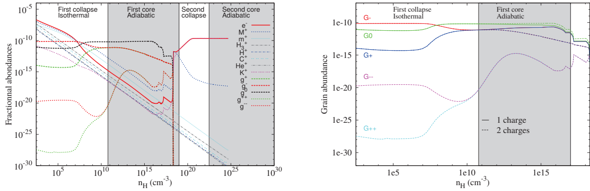
Figure 2.15: Left panel: abundances of the chemical species with double-charge grains, without Na, thermal ionisation of H and thermionic emission. Right panel: abundances of the grains with and without double-charged grains presence.
