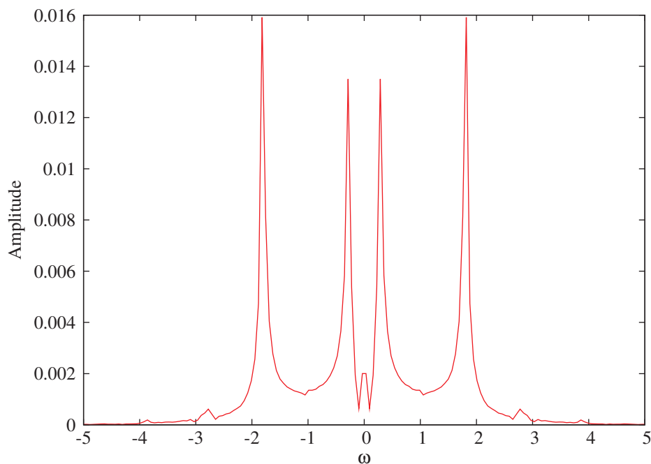
Figure 3.11: Fourier transform of B_y(t) for a random cell in the box (here x = 0.378906265 = 48.5/128 , y = 0.00390625 = 0.5/128 , z = 0.49609375 = 63.5/128 ). k = 7 \text{ cm}^{-1} , \eta_{\text{H}} = 5 \times 10^{-3} \text{ cm}^2 \text{ s}^{-1} .
