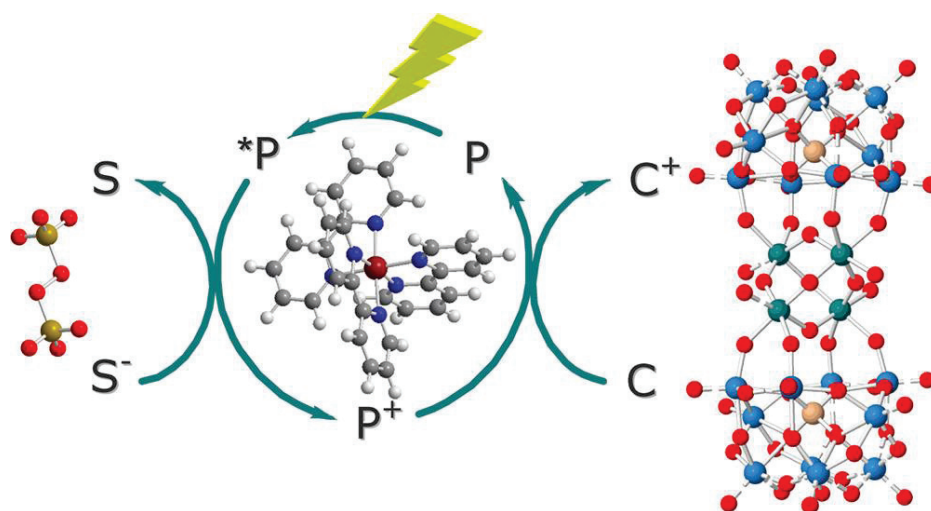
Figure 2. 13- Hybrid \text{Ru}_4\text{POM}@Ru(\text{bpy})_3 ionic system used for the photo-oxidation of water, in presence of persulfate as electron acceptor.
