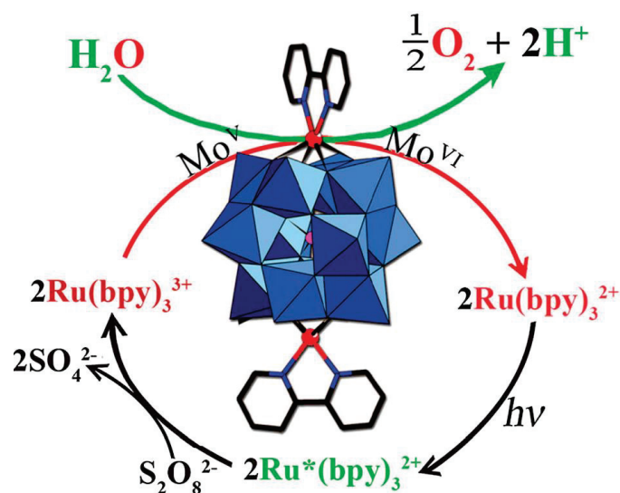
Figure 2. 15- Bicapped 2,2 bipyridine keggin POM catalyzes water oxidation to generate O 2 under visible light irradiation, using [Ru(bpy)_3]^{2+} as the photosensitizer and S_2O_8^{2-} as the sacrificial electron acceptor
