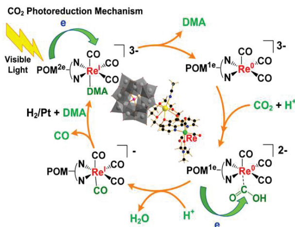
Figure 2. 41- Photoreduction mechanism of CO 2 (Re)organo-POM catalyzed.
