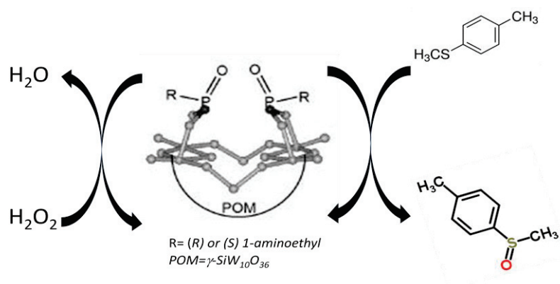
Figure 2. 29- Enantioselective oxidation reaction catalyzed by the chiral hybrid POM proposed by Carraro et al.
