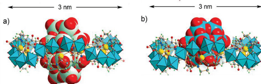
Figure 1.11- a) Well-Dawson Hybrid [(P_2W_{18}O_{62})Mo_{24}(Fe-edta)_{12}O_{72}]^{18-} ; and b) Keggin hybrid [(SiMo_{12}O_{40})Mo_{24}(Fe-edta)_{12}O_{72}]^{16-} .
