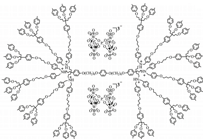
Figure 1. 3- Structure of the encapsulated-POM into polycationic dendritic units
