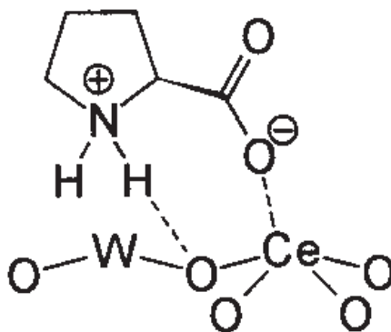
Figure 4. 5- Representation of the possible interaction between \alpha_1\text{-}[\text{P}_2\text{W}_{17}\text{O}_{61}\text{Ce}]^{7-} and Amino Acids. Here the example of L -proline.
