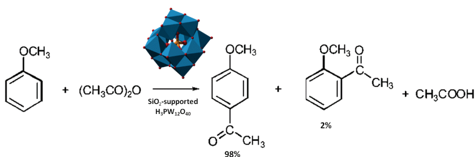
Figure 3. 1- Friedel-Craft reaction catalyzed by SiO 2 -supported HPAs, presented by Kaur et al.
