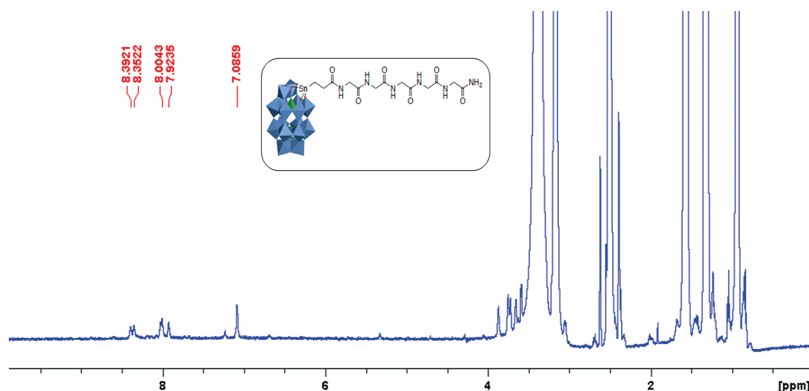
Figure 4. 19- 1 H-NMR spectrum of α 2 -Gly 5 in d 6 -DMSO. Spectrum recorded at 600 MHz, 298K, 3.3 mM.
