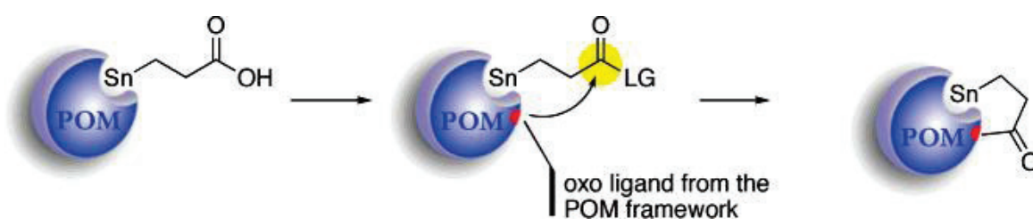
Figure 4. 8- General Strategy for Regioselective Acylation of Oxo Ligands (LG =Leaving Group)
