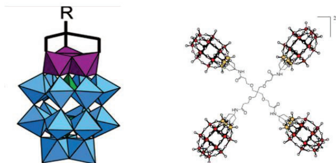
Figure 1. 24- Polyhedral representation of [(RC(CH_2O)_3)_2P_2V_3W_{15}O_{59}]^{6-} ( R = CH_3, NH_2, NO_2 ) on the left, and representation of the tetra-polyoxometalate dendrimer synthesized by Hill and co-workers, on the right.
