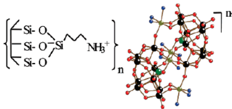
Figure 1. 8- SBA-15-apts- Fe_4X_2W_{18} ( n=6 , if X=As^{III} , Sb^{III} ; n=4 , if X=Se^{IV} , Te^{IV} )
