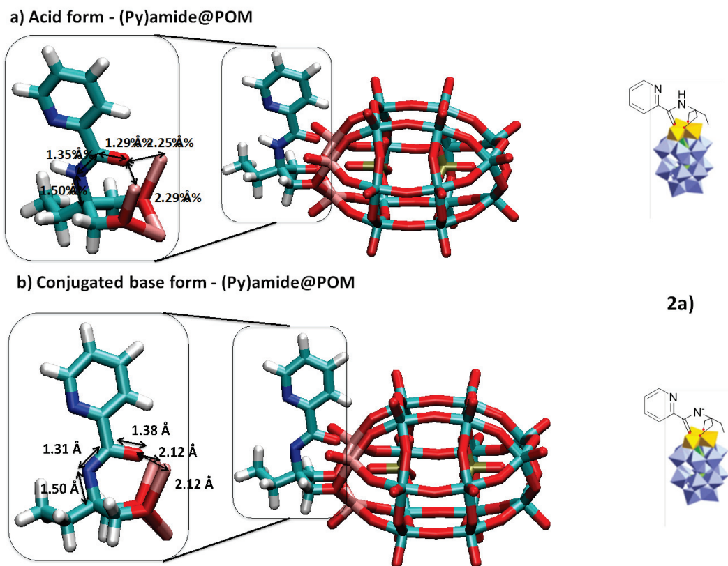
Figure 3. 13- Optimized geometries with explicit bond lengths of the acid form (a) and conjugate base form (b) for (Py)amide@POM (2a).
