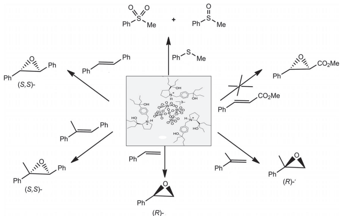
Figure 2. 27- Catalytic oxidation of different substrates by proline-derived DENDRI-POM, using \text{H}_2\text{O}_2 , presented by Jahier and Nlate.
