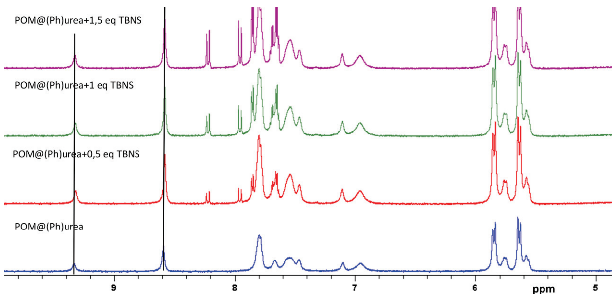
Figure 3. 19- ^1\text{H} -NMR spectra superposition of titrated \text{CD}_3\text{CN} solution of \text{POM}@\text{(Ph)urea} (8mM) with a \text{CD}_3\text{CN} solution of TBNS. Spectral width between 5 and 10 ppm to investigate the ureic proton signals shift. The vertical black lines are centered on the ureic proton signals of the catalyst. (Spectra recorded at 600 MHz, in \text{CD}_3\text{CN} , at 298K).
