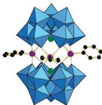
Figure 1. 18- Structure of organo-tin derivative [(PhSn) 3 -Na 3 ( \gamma -SbW 9 O 33 ) 2 ] 6- synthesized by Pope.
