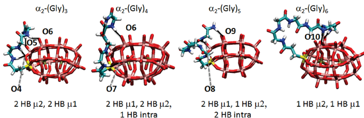
Figure 4. 22- Cartoon representation for the folded hybrid-POMs of the \alpha_2\text{-(Gly)}_n series. The number of HB is given. Acetonitrile and counterions are omitted.
