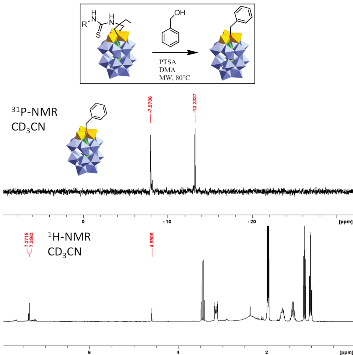
Figure 3. 17- Coupling reaction scheme between (Ph)thiourea@POM and benzyl alcohol. The 31 P-NMR and 1 H-NMR spectra, after the work-up and the re-crystallization in diethyl ether vapors, show that only the benzyl alcohol is grafted on the POM.
