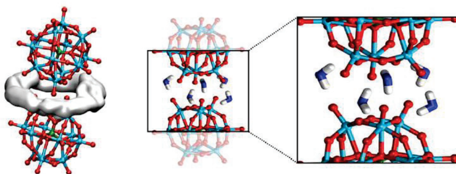
Figure 1. 34- PW_3 \dots PW_3 dimer in water: H_2O density between two PW 's (averaged over 500 ps; left) and snapshot of bridging water molecules (middle and right)
