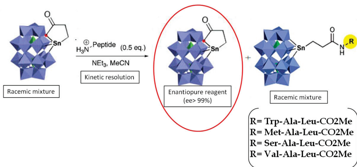
Figure 4. 9- \alpha_1 -tripeptides substituted lacunary Dawson POM, \alpha_1 -[P 2 W 17 O 61 ] 10- , presented by Micoine et al. efficiently employed for the kinetic resolution of the chiral substituted-POM.
