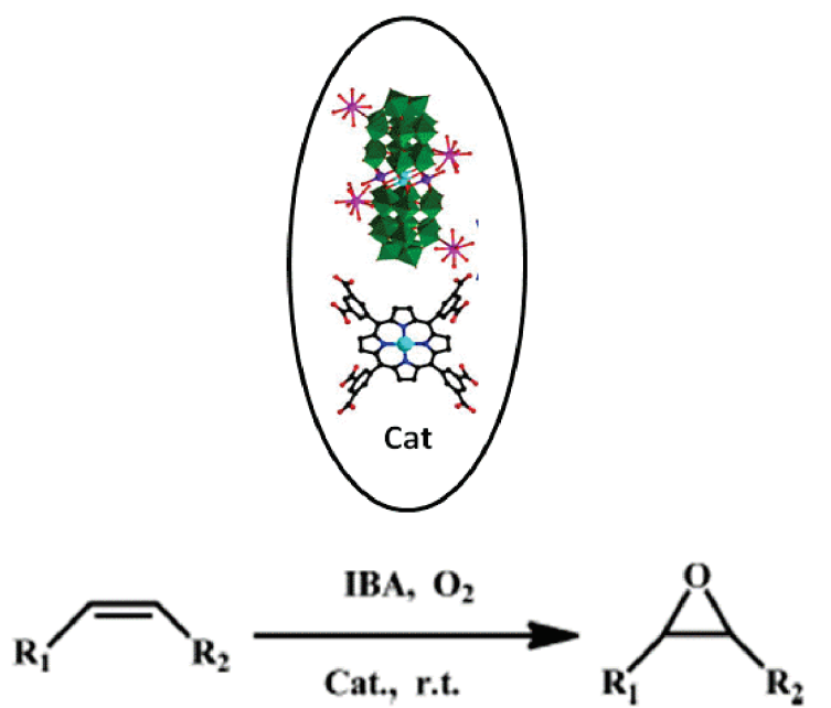
Figure 2. 10- Schematic representation of the two components of the hybrid system and catalyzed reactions scheme.
