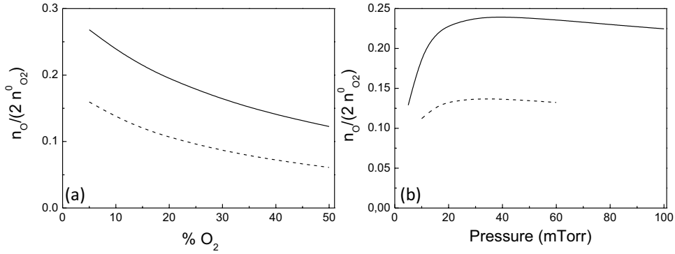
Figure 4. Oxygen dissociation as a function of O 2 fraction at 30 mTorr (a) and as a function of pressure with 10% of O 2 (b) for two different powers: 200 W (dashed line) and 400 W (solid line).
