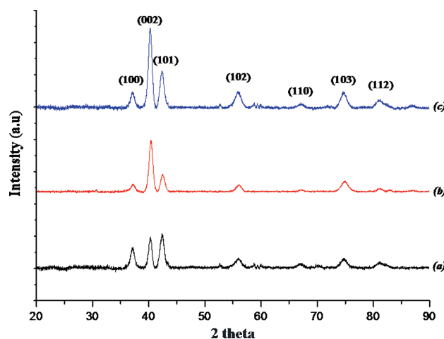
Fig. 2. XRD patterns of Al-ZnO prepared at various plasma gas composition (a) ( \text{Ar}:\text{O}_2 ) = (200:10)mL/min (b) ( \text{Ar}:\text{O}_2 ) = (200:0)mL/min (c) ( \text{Ar}:\text{O}_2 ) = (100:0)mL/min.
