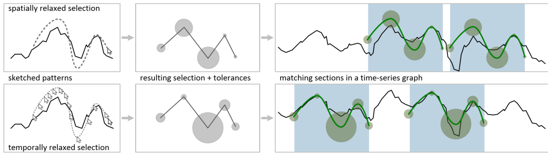
Figure 3.22: Relaxed Selection Query on Time Series [Holz and Feiner, 2009]
