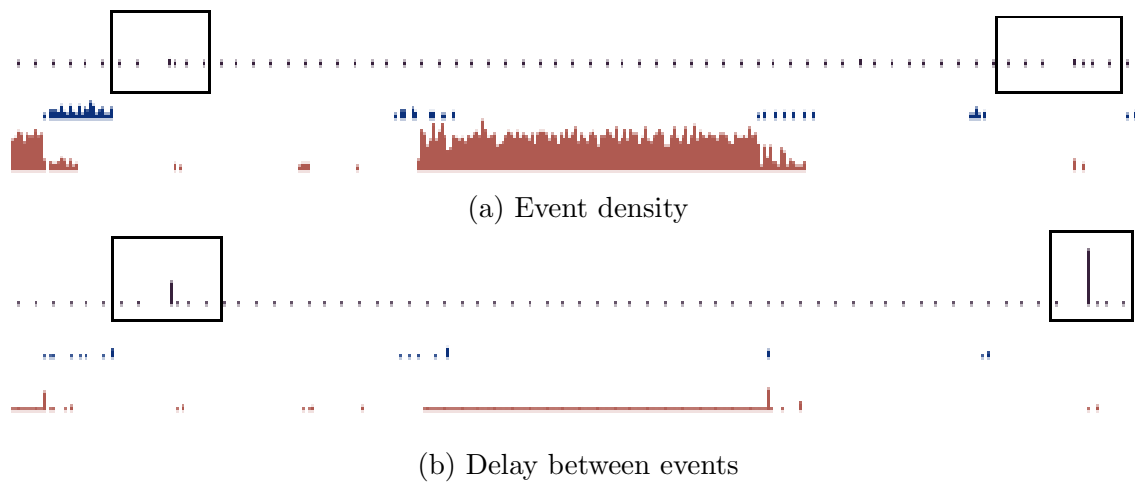
Figure 7.10: When the dd task (in brown) is unscheduled, the jbd2-sda1-8 task (in blue) loads the CPU, causing a delay on the treatment of the callback for the VSync IRQ on the main output (in purple).
