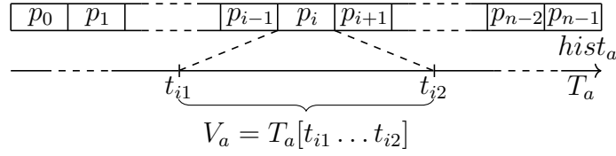
Figure 7.3: Building of the histogram hist_a for an actor a
