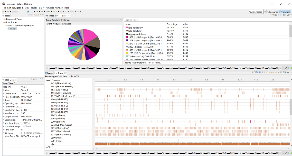
Figure 7.12: FrameSoC interface. It shows a statistics about the event producer instances as a pie chart (top left) and a tabular view (top right). On the bottom is the time chart provided by FrameSoC.
