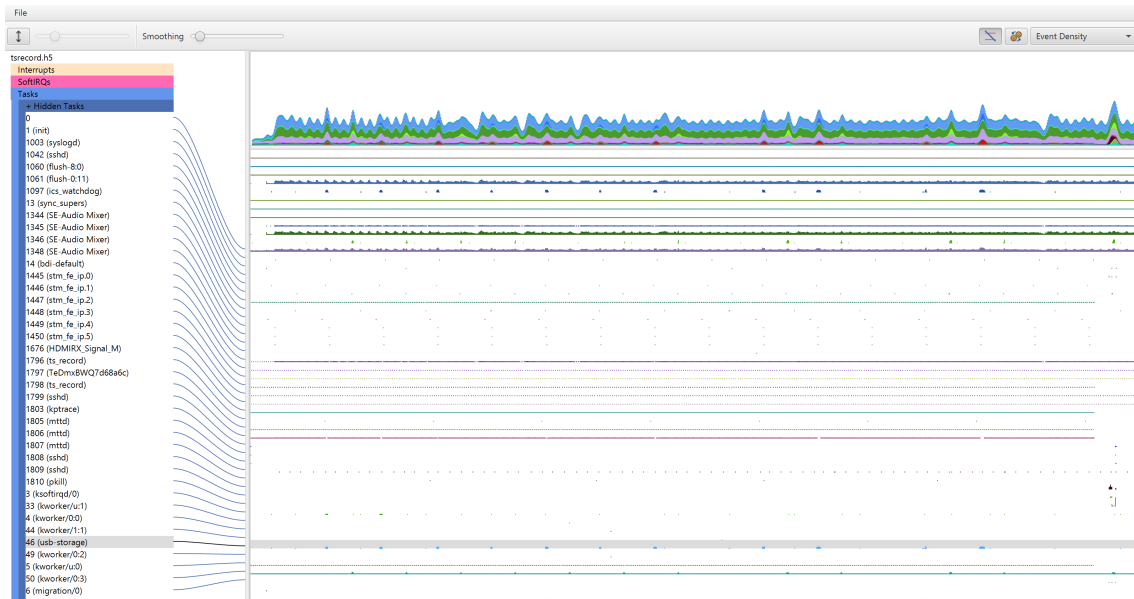
Figure 9.2: TSRecord trace visualized in TraceViz.
