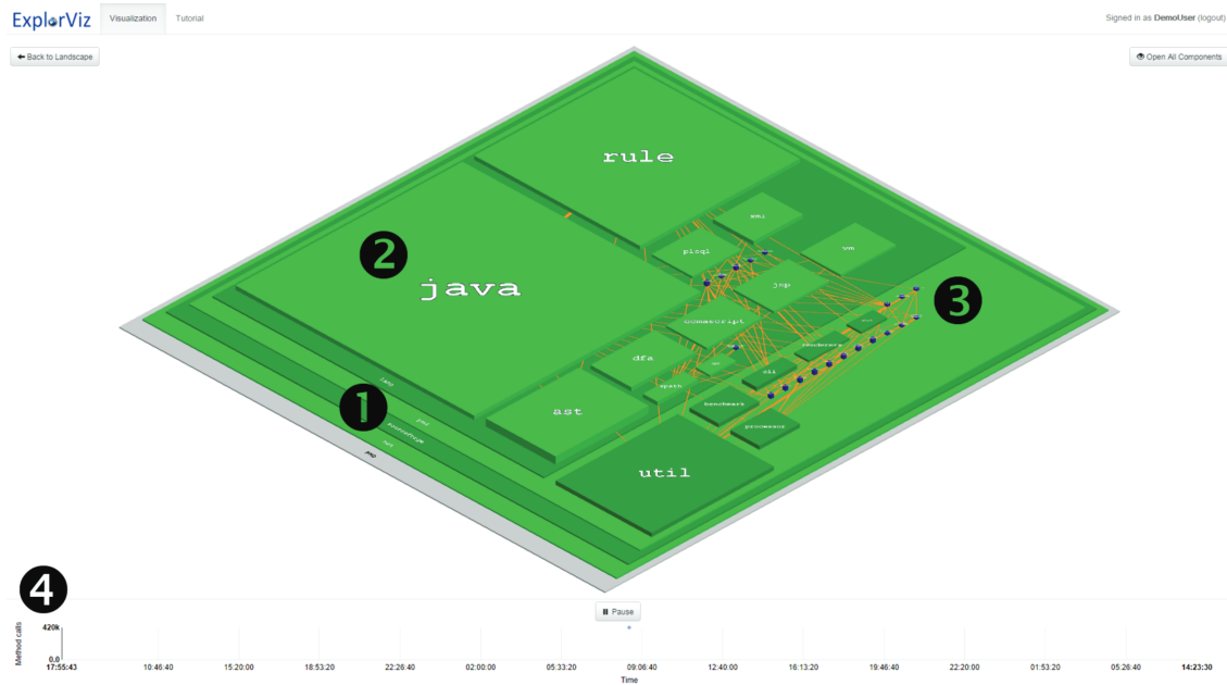
Figure 3.24: ExplorViz is a treemap-based to visualize Java programs execution [Fitkai et al., 2013]
