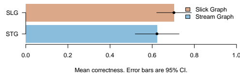
Figure 6.13: Mean correctness for the Same task.
