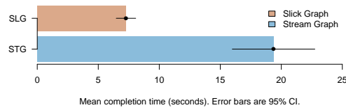
Figure 6.10: Mean completion time for the Period task.
