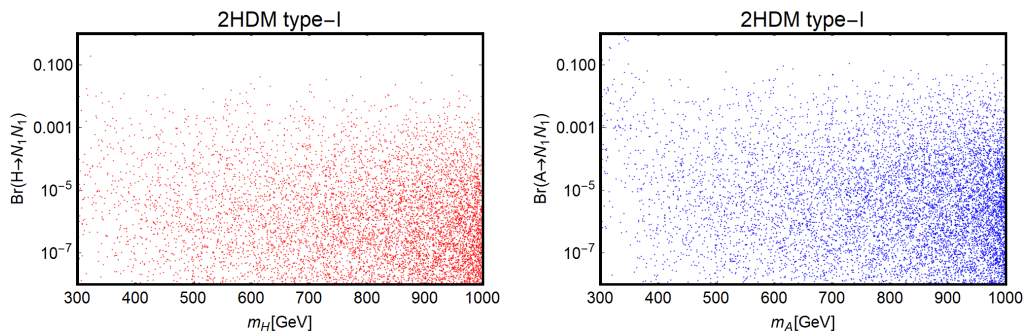
Figure 5.12 – Decay branching ratios of the Heavy CP even (left panel) and CP-odd (right panel) scalar into N_1 N_1 , as a function of their masses.
