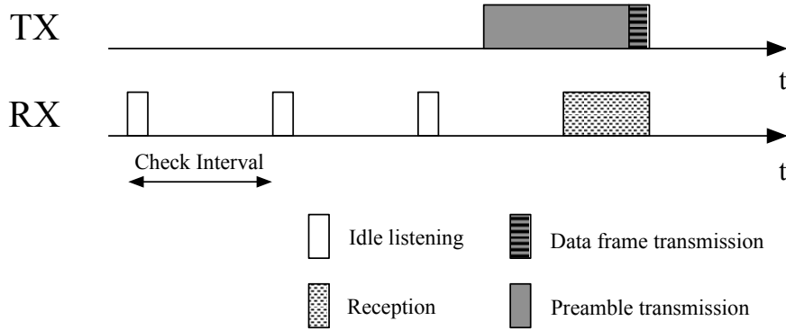
Figure 3.2: Basic principle of preamble sampling techniques.
