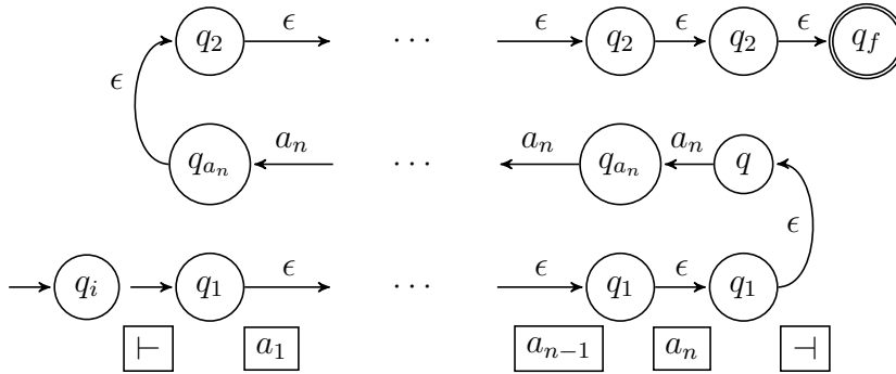
Figure 2.13: A run of \mathcal{H} on the input \vdash a_1 \cdots a_n \dashv .
