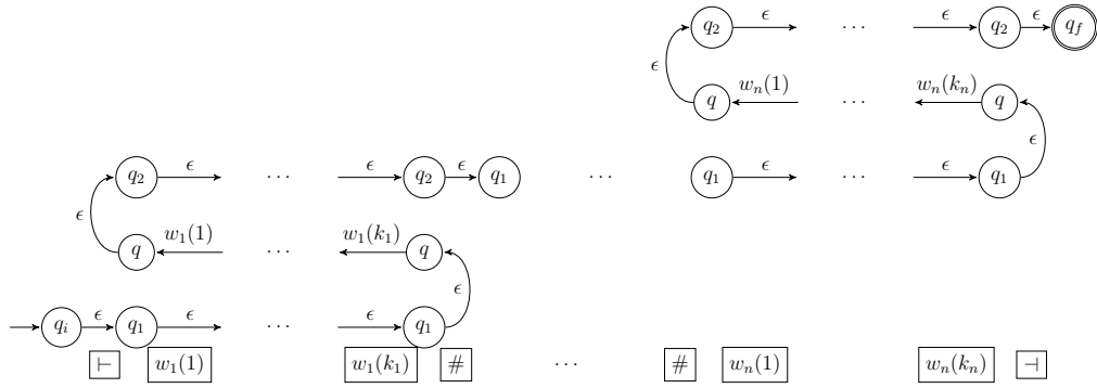
Figure 2.8: A run of \mathcal{G}' on \vdash w_1 \# \dots \# w_n \dashv .
