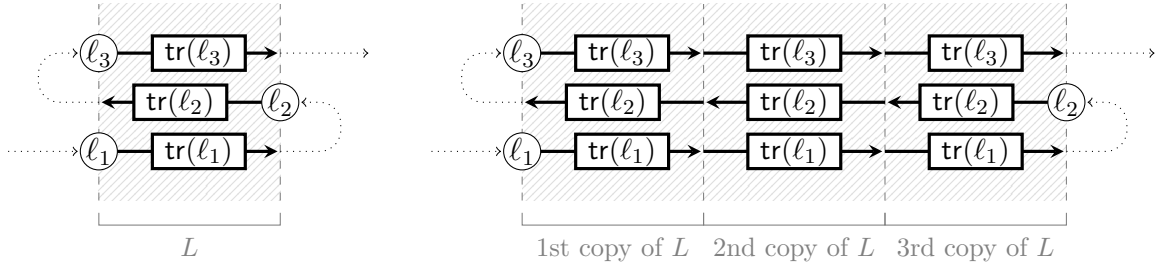
Figure 3.2: A loop L with 3 anchor points, and the result of pumping.
