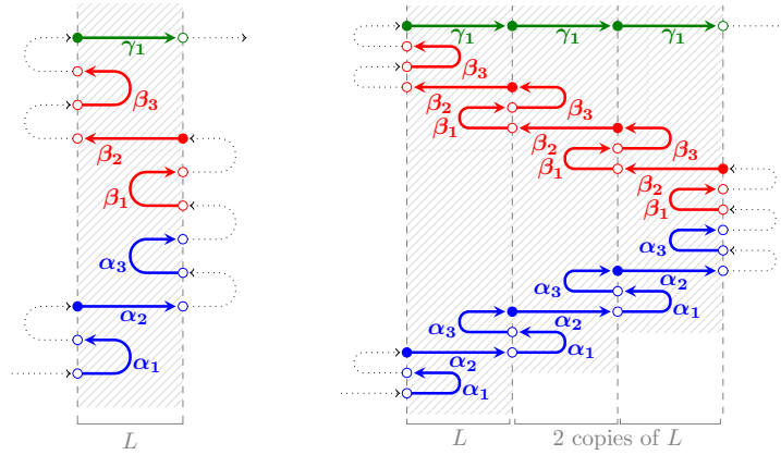
Figure 3.9: Pumping an idempotent loop with three components.
