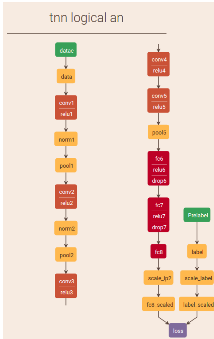
FIGURE A.2 – Structure du CNN AlexNet
