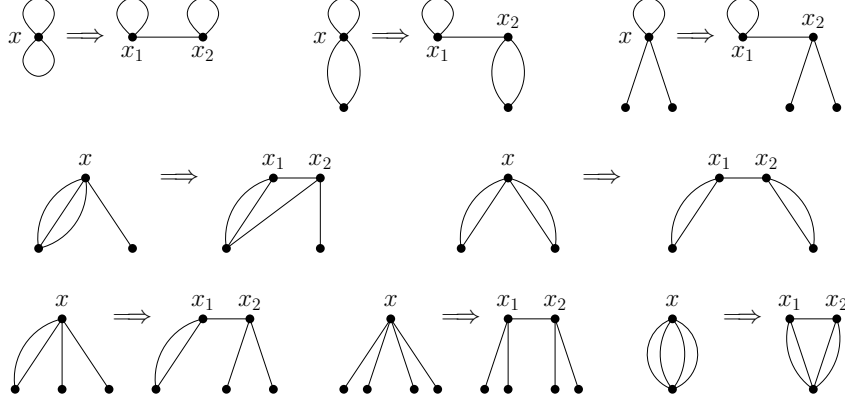
Figure 5.7: Vertex stretching.
