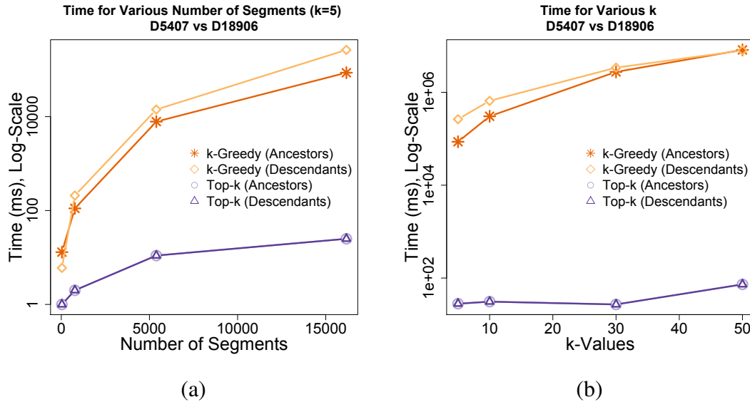
Fig. 3.10 Response time for various (a) Segments, (b) k -values
