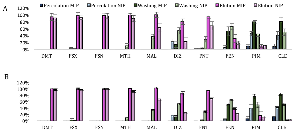
Figure III.4-3. Extraction profiles obtained when percolating the ten OPs (A) on MIP/NIP ( n=3 assays) and (B) on two MIPs/NIPs synthesized independently using the same condition of synthesis ( n=3 assays on each synthesis of MIP, n=6 ). The extraction procedure was the same as in Figure III.4-2.
