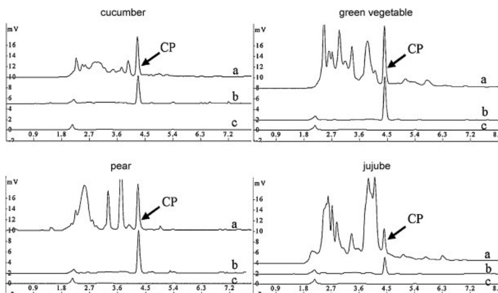
Figure II.5-2. HPLC chromatograms of (a) spiked sample solution containing 1 \mu\text{g mL}^{-1} chlorpyrifos (CP), (b) spiked sample solution extracted with CP-imprinted nanoparticles, and (c) spiked sample solution extracted with non-imprinted nanoparticles [41].
