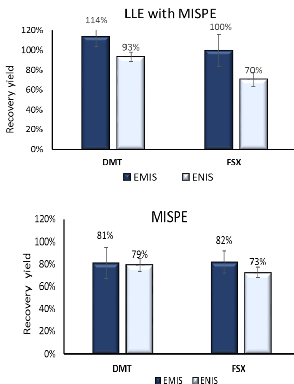
Figure IV.4-7. Recovery yield (%) \pm SD (n= 3) of the DMT and FSX in the elution fraction of MISPE using 10 mL of almond oil extract spiked with 100 \mu g/kg, with and without a previous LLE step.
