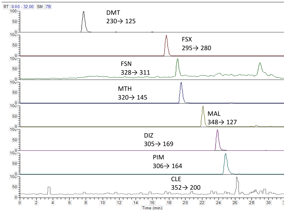
Figure 1. LC-MS chromatograms (MRM mode) of the elution fraction of an almond oil extract spiked at 100 \mu\text{g}/\text{kg} with eight OPIs issued of the MIP. Extraction procedure was described in part III.3.5.2 (washing volume of 0.65 mL).
