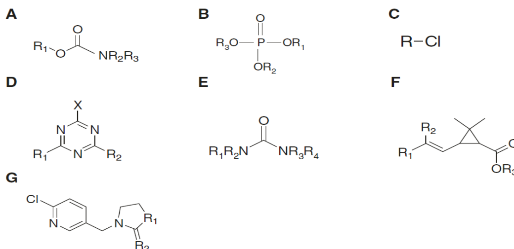
Figure I.1-1. Generic chemical structures of pesticides: A, carbamate pesticides; B, organophosphorus pesticides; C, organochlorine pesticides; D, triazines (X= halogen); E, urea analogs; F, pyrethrum-derived pyrethroids ( R_1, R_2= H, \text{halogen or other functions} ); and neonicotinoid [4].
