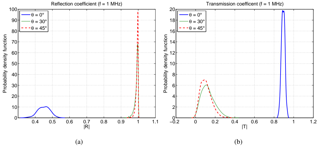
Figure 2.22: See caption of Fig. 2.21. These results are obtained with f = 1 MHz.
