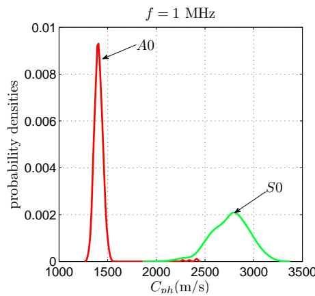
Figure 3.6: (Color online) Probability density functions (PDF) of A_0 and S_0 modes at a given frequency f = 1 MHz when \delta = 0.1 .
