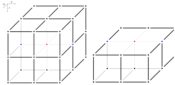
Figure 4.6: 9-point sparsity pattern. The source point is marked by the red bullet at the center of the cube. The discretization points involved in the stencil are colored in blue. It is the grid points which are adjacent to the source and are located on the axis where the force source is applied ( Ox in this case). The particle velocities v_y and v_z are set to 0.
