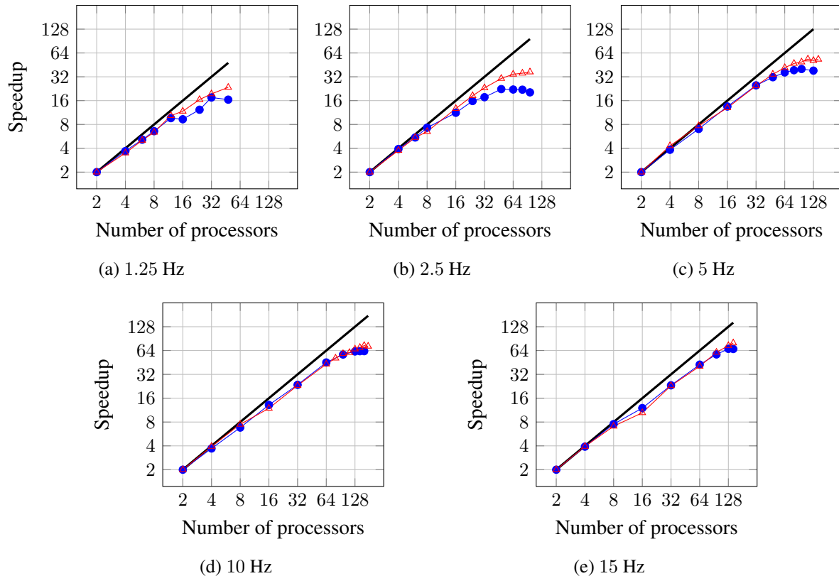
Figure 3.21: Speedup analysis for the 2D frequency-domain elastic wave simulations with the FSBC and the space-dependent Poisson's ratio Marmousi 2 model at 1.25 Hz (a), 2.5 Hz (b), 5 Hz (c), 10 Hz (d) and 15 Hz (e). The blue curves \bullet are used to plot the results of the CARP-CG method without preconditioning and the red curves \blacktriangle are used for the CARP-CG method with preconditioning. The black solid lines represent the ideal speedup.
