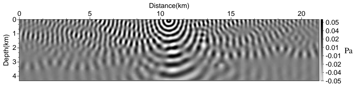
Figure 2.11: Marmousi 2 acoustic pressure wavefield (real part) solution at 5 Hz.
