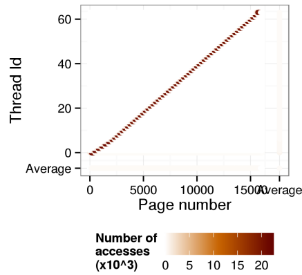
(a) Access distribution
