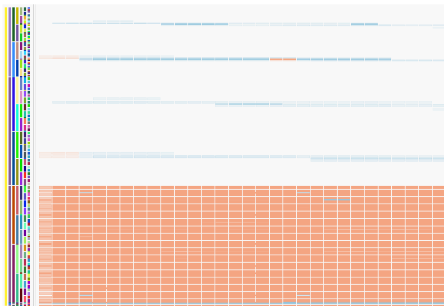
Figure 6.7 – Sharing view of the memory usage of a naive parallel matrix multiplication, computing phase.
