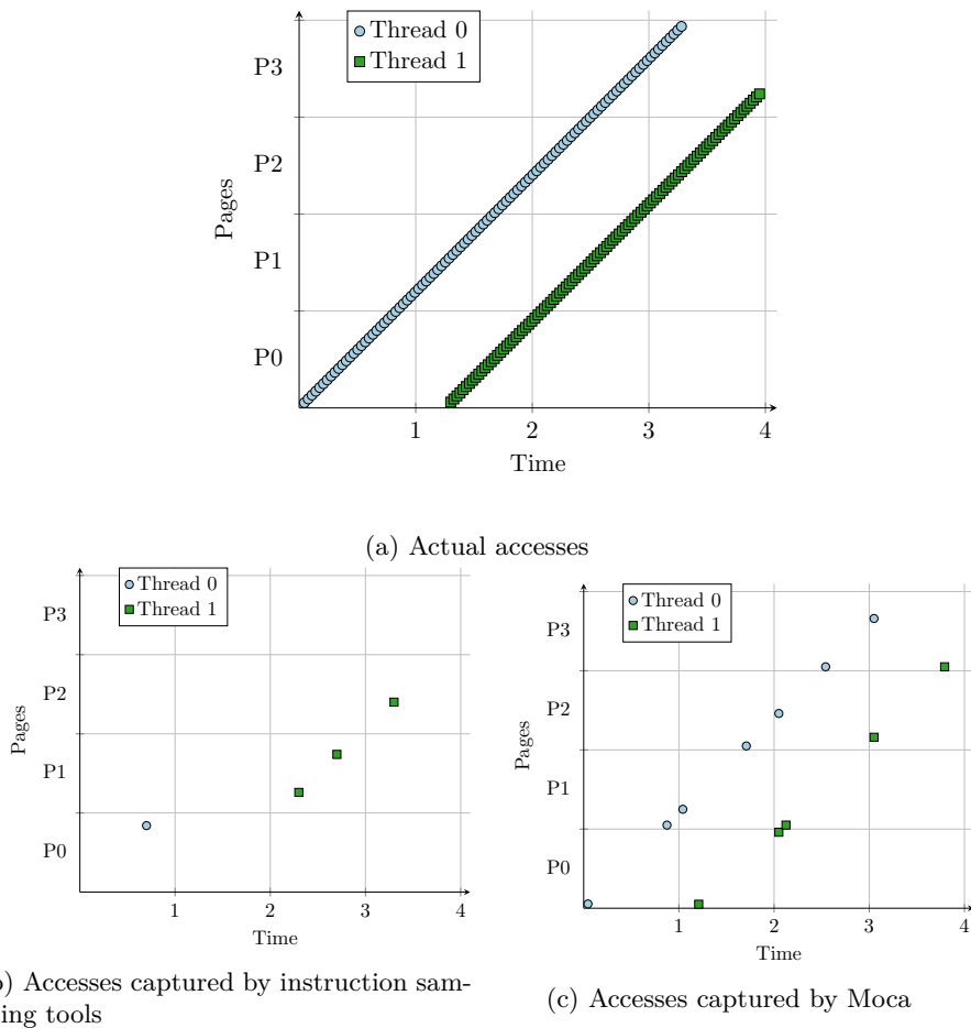
Figure 5.1 – Accesses done by two threads on a set of pages, captured by instruction sampling tools and by Moca.
