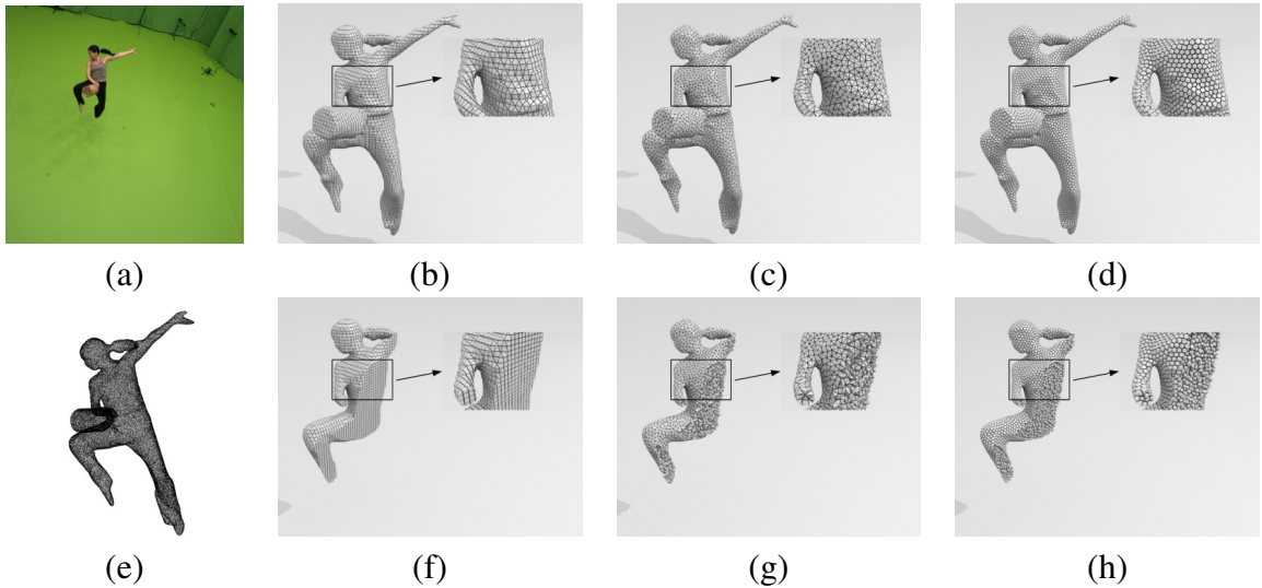
Figure 6.3 – (a, e) Input multi-camera observations and surface reconstruction (15k points). (b,f) Tessellations generated using voxels [152]. (c,g) Tetrahedralisations generated using Delaunay refinement [153]. (d,h) Clipped centroidal Voronoi tessellations (14455 sites).
