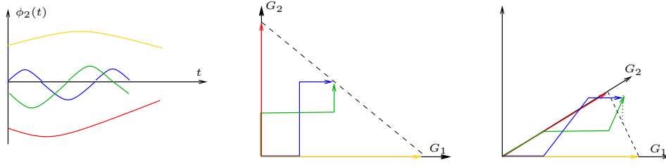
Figure 17: Extremals when |f_{41}| < -f_{51}
