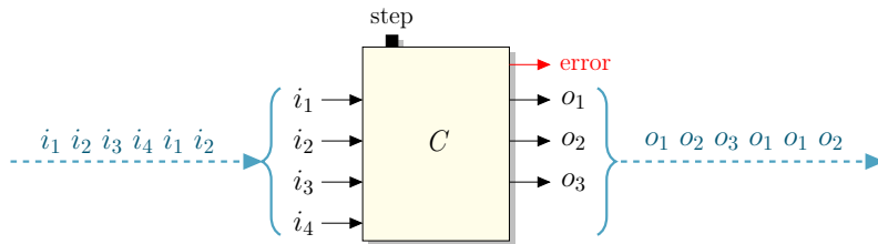
Figure 8.11 A stub receiving (resp. producing) a sequence of inputs (resp. outputs).
