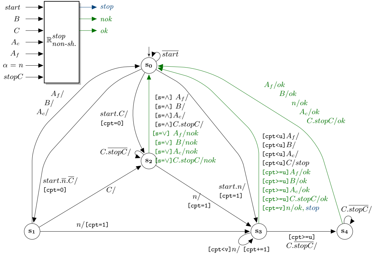
Figure 5.10 The stopping elementary recognizer \mathbb{R}^{\text{stop}}_{\text{non-shuffled}} of a range appearing in a fragment with the non-shuffled semantics ( \sqcup = \text{Non-Shuffled} ).
