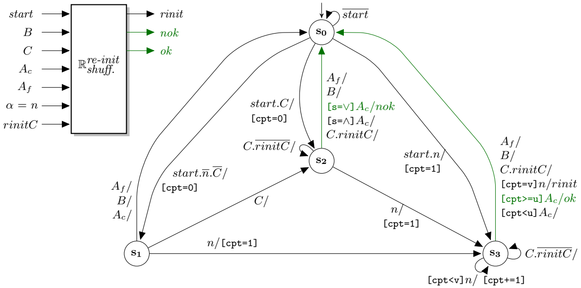
Figure 5.9 The re-initializing elementary recognizer \mathbb{R}^{re-init}_{shuffled} of a range appearing in a fragment with the shuffled semantics ( \sqcup = Shuffled ).
