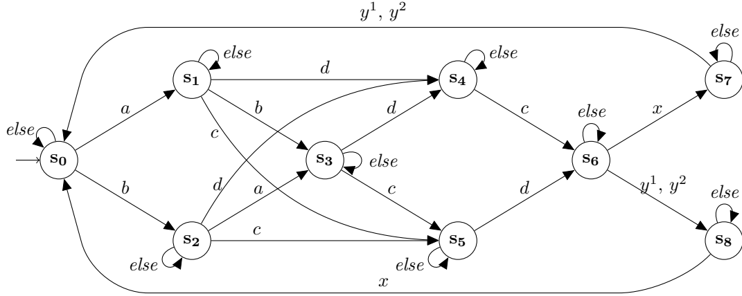
Figure B.27 The SPOT monitor for the LTL encoding of \left( (\{a, b\}, \vee) < (\{c, d\}, \wedge) \implies (\{x, y^{[1,2]}\}, \wedge) \mid t \right) . else stands for any name which is not of \{a, b, c, d, x, y1, y2\} . “ y1, y2 ” means that y1 and y2 cannot occur simultaneously. Transitions which are not defined are forbidden.
