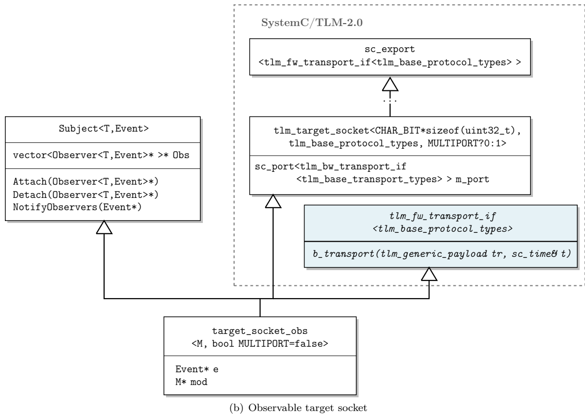
Figure 6.16 Observable SystemC/TLM sockets.
