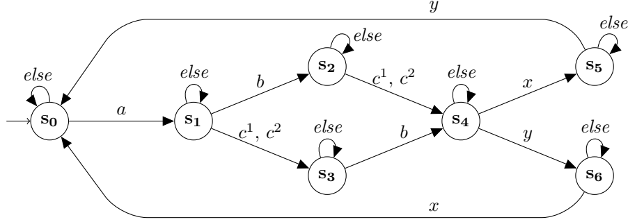
Figure B.15 The SPOT monitor of the LTL encoding of (a < (\{b, c^{[1,2]}\}, \wedge) \implies (\{x, y\}, \wedge) \mid t) . else stands for any name which is not of \{a, b, c1, c2, x, y\} . “ c1, c2 ” means that c1 and c2 cannot occur simultaneously. Transitions which are not defined are forbidden.
