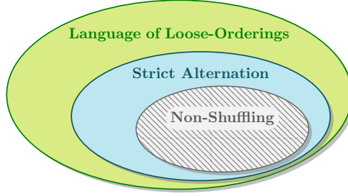
Figure 4.11 The subset of the loose-ordering language encoded into SERE and LTL (the lined area).
