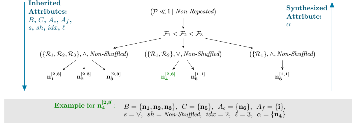
Figure 5.3 A syntax tree of the loose-ordering property ((\{n_1^{[2,3]}, n_2^{[2,3]}, n_3^{[2,3]}\}, \wedge, Non-Shuffled) < (\{n_4^{[2,8]}, n_5\}, \vee, Non-Shuffled) < n_6 \ll i \mid Non-Repeated) .
