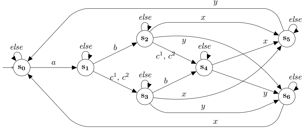
Figure B.21 The SPOT monitor for the LTL encoding of (a < (\{b, c^{[1,2]}\}, \vee) \implies (\{x, y\}, \wedge) \mid t) . else stands for any name which is not of \{a, b, c1, c2, x, y\} . “ c1, c2 ” means that c1 and c2 cannot occur simultaneously. Transitions which are not defined are forbidden.
