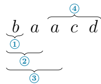
Figure 2.44 Overlapping occurrences of a regular language ba^* + acd in a sequence baacd .
