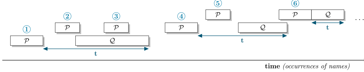
Figure 4.10 Ignoring occurrences of \mathcal{P} : the second, the third and the fifth occurrences of \mathcal{P} are ignored because they overlap with \mathcal{Q} .
