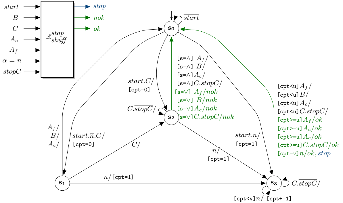
Figure 5.11 The stopping elementary recognizer \mathbb{R}^{\text{stop}}_{\text{shuffled}} of a range appearing in a fragment with the shuffled semantics ( \sqcup = \text{Shuffled} ).
