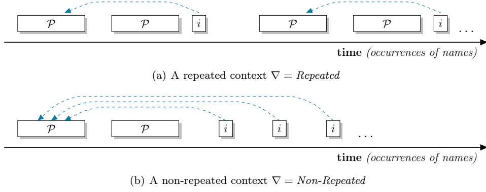
Figure 4.8 Elaborated semantics of \mathcal{A} = (\mathcal{P} \ll i \mid \nabla) .
