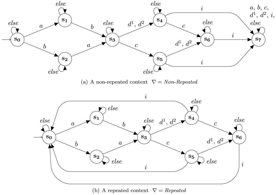
Figure B.5 The SPOT monitor for the LTL encoding of ((\{a, b\}, \wedge) < (\{c, d^{[1,2]}\}, \vee) \ll i \mid \nabla) . else stands for any name which is not of \{a, b, c, d1, d2, i\} . “ d1, d2 ” means that d1 and d2 cannot occur simultaneously. Transitions which are not defined are forbidden.
