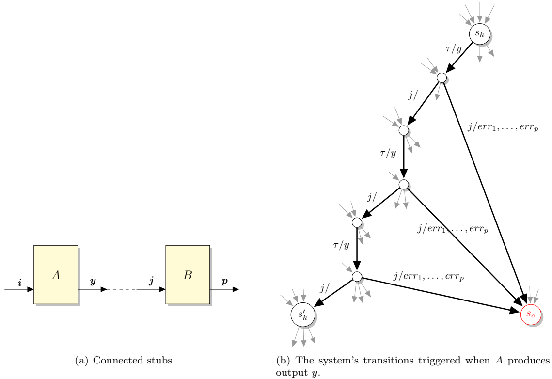
Figure 10.3 Impact of the atomicity of the SystemC processes on the execution of the stub-based system: output y of A is connected to input j of B ; \tau enables production of output y of A .
