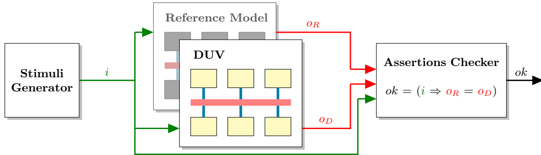
Figure 2.6 Black-box assertion checking for system level verification.
