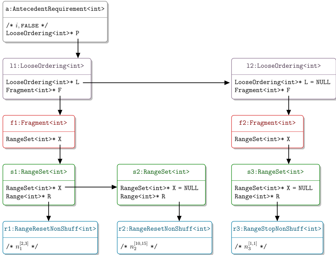
Figure 6.8 Structure of a monitor of the antecedent requirement ((\{n_1^{[2,3]}, n_2^{[10,15]}\}, \wedge, \text{Non-Shuffled}) < n_3 < i \mid \text{Non-Repeated}) .
