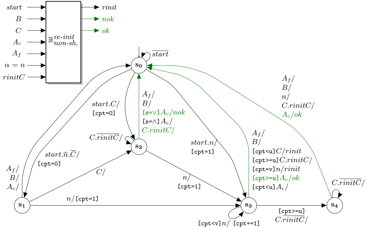
Figure 5.8 The re-initializing elementary recognizer \mathbb{R}^{re-init}_{non-shuffled} of a range appearing in a fragment with the non-shuffled semantics ( \sqcup = Non-Shuffled ).
