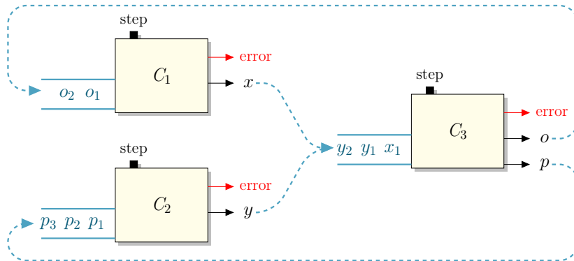
Figure 8.12 Simulation of a system made of stubs.
