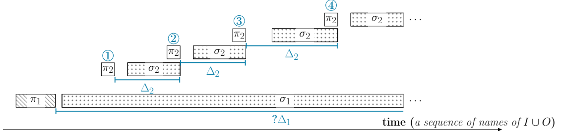
Figure 8.9 A bound \Delta_1 of \pi_1 \Rightarrow \sigma_1 cannot be computed if \pi_2 \Rightarrow \sigma_2 is a cycle such that outputs of \sigma_2 are \pi_2 -fragments.
