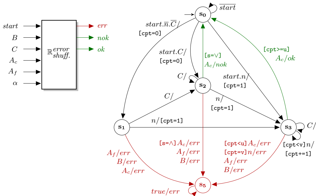
Figure 5.7 The error-reporting elementary recognizer \mathbb{R}_{shuffled}^{error} of a range appearing in a fragment with the shuffled semantics ( \sqcup = Shuffled ).
