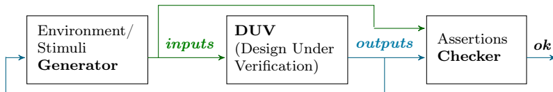
Figure 8.2 The testing framework for reactive systems.
