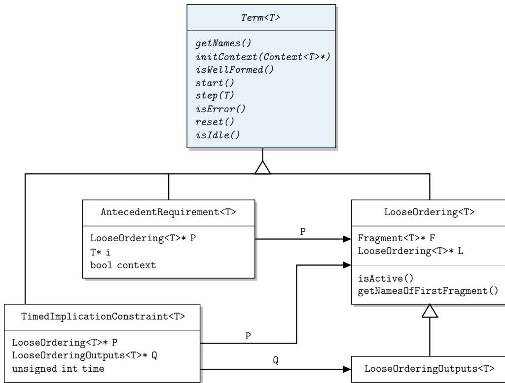
Figure 6.7 SystemC Implementation of the primitive monitors of loose-orderings: the class diagram. Part II.
