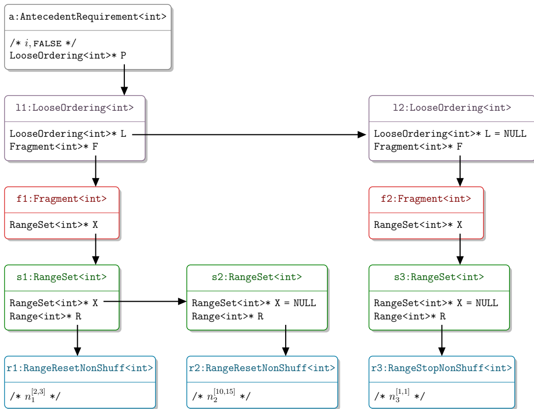
Figure 6.8 Structure of a monitor of the antecedent requirement ((\{n_1^{[2,3]}, n_2^{[10,15]}\}, \wedge, Non-Shuffled) < n_3 \ll i | Non-Repeated) .
