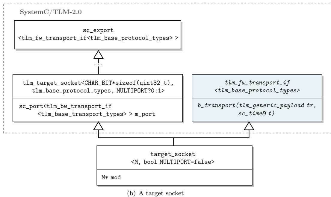
Figure 3.9 The definition of TLM sockets.
