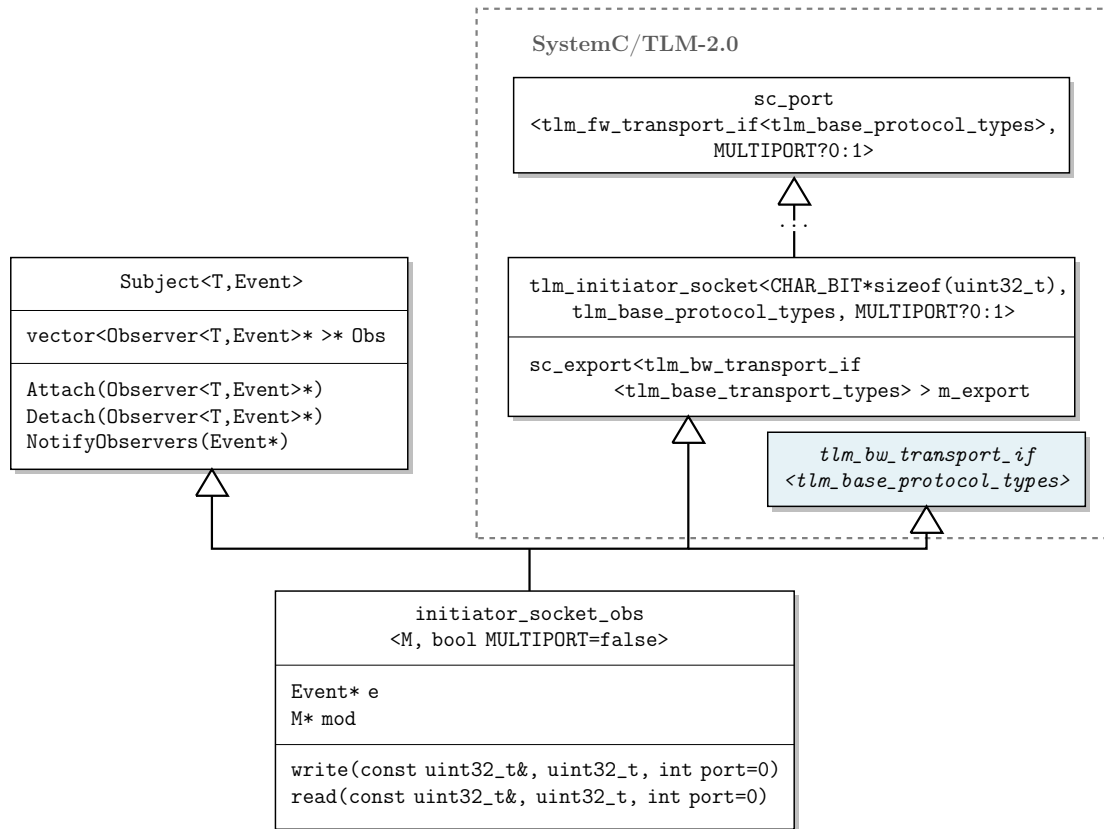
(a) Observable initiator socket
