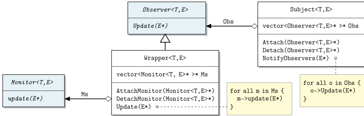
Figure 6.2 The monitoring model.
