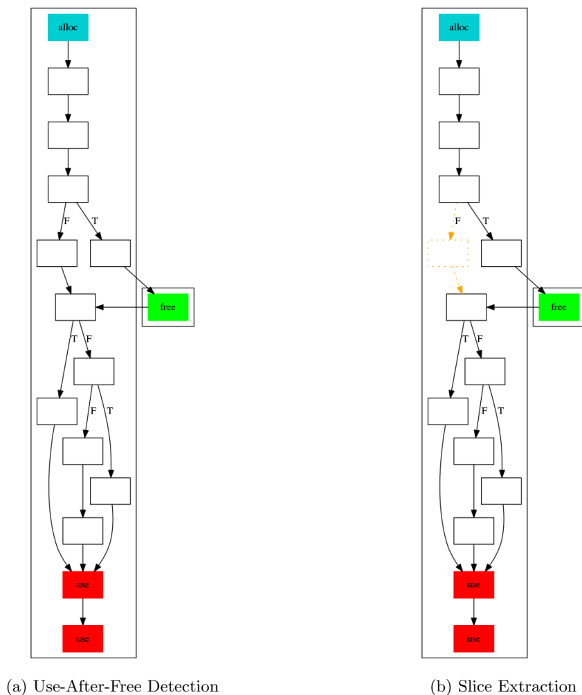
Figure 3.4: Use-After-Free detection.
