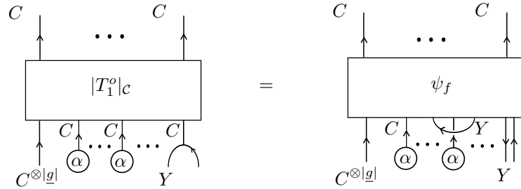
Figure 4.8 – Toward the computation of the invariant |T|_{\mathcal{C}, \alpha} using T_1^o .
