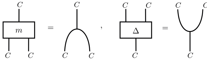
Figure 1.6 – The product and the coproduct of C .
