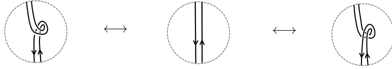
The two arcs belong to the same surgery or exit component.
