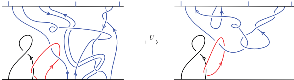
Figure 3.6 – The map U from Otang to Tang^{Cob} .
