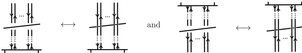
All components of the same entrance or exit boundary component can cross any component.
