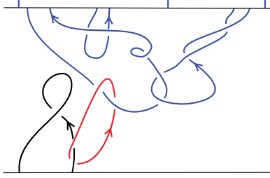
Figure 3.3 – A ribbon ((1), 1, (2, 1)) -cobordism tangle.
