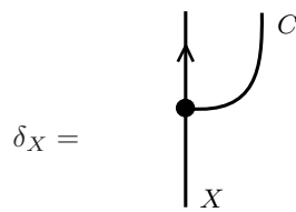
Figure 1.4 – The universal natural transformation of the coend.
