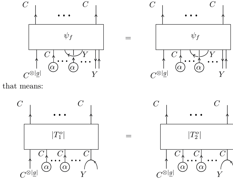
Figure 4.11 – Equal invariants.
