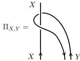
Figure 4.2 – A useful morphism
