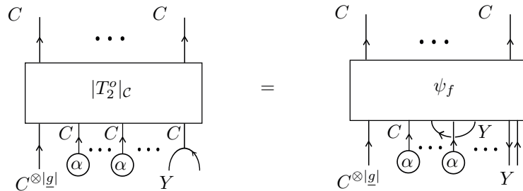
Figure 4.9 – The invariant |T|_{\mathcal{C}, \alpha} using T_2^o .
