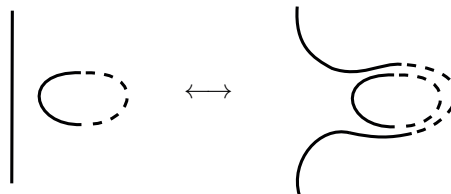
Any component can slides over a surgery component. Figure 3.13 – The move KII^g on cobordism tangles.
