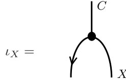
Figure 1.2 – The universal dinatural transformation of the coend.
