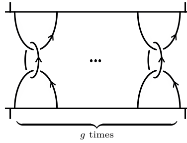
Figure 3.10 – A cobordism tangle which presents the cylinder of a surface of genus g .
