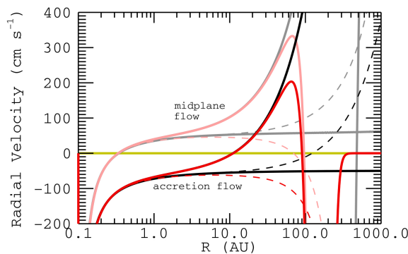
Figure 2.8: Radial advection velocities of the disk gas (black/gray) and dust (red/pink) from ?. Solid colors represent accretion flow and paler colors represent midplane flow case. Solid lines are for t=0 and dashed lines for t=1 Myr.
