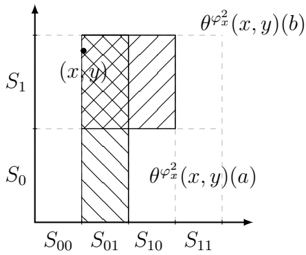
Figure 8.5: After the announcement of \varphi_x^2 , we obtain the following smaller neighbourhoods given by the updated function \theta^{\varphi_x^2} : \theta^{\varphi_x^2}((x, y))(a) = S_{01} \times \{0, 1\}^\infty , and \theta^{\varphi_x^2}((x, y))(b) = (S_{01} \cup S_{10}) \times S_1 .
