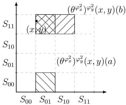
Figure 8.6: After further announcing \varphi_y^2 , the updated function (\theta^{\varphi_x^2})^{\varphi_y^2} gives the neighbourhoods: (\theta^{\varphi_x^2})^{\varphi_y^2}(x, y)(a) = S_{01} \times (S_{00} \cup S_{11}) , and (\theta^{\varphi_x^2})^{\varphi_y^2}(x, y)(b) = (S_{01} \cup S_{10}) \times S_{11} .
