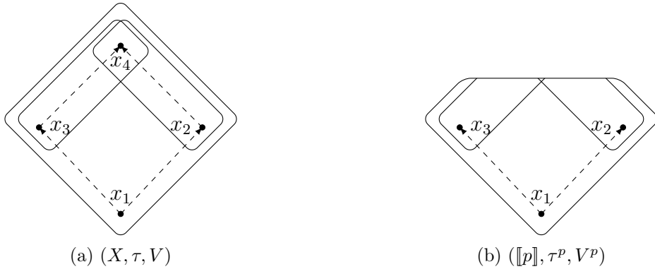
Figure 4.1: Update of (X, \tau, V) by p .
