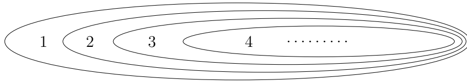
Figure 5.1: \mathfrak{M} = (\mathbb{N}, \mathcal{E}_0, V)
