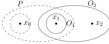
Figure 5.6: \mathfrak{M} = (X, \mathcal{E}_0, V) : The continuous ellipses represent the currently available pieces of evidence, while the dashed ones represent the other nonmisleading propositions.
