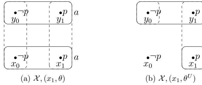
Figure 8.8: The straight round circles show the neighbourhoods of agent a , and the dashed ones are for agent b .
