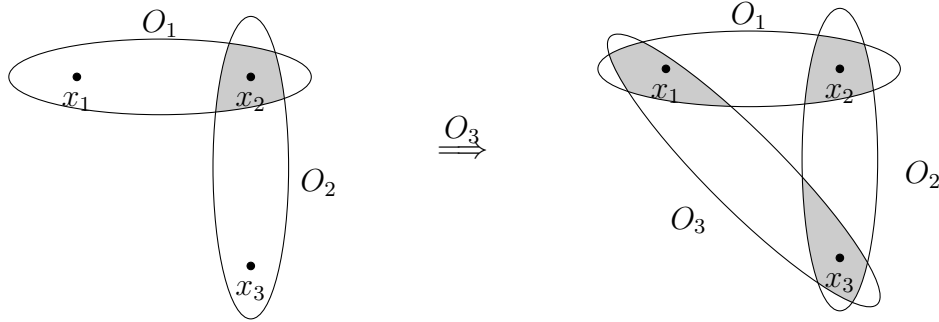
Figure 5.5: From \mathfrak{M} to \mathfrak{M}^{+O_3}
