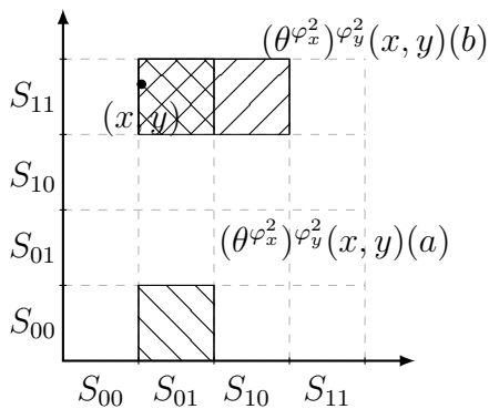
Figure 8.6: After further announcing \varphi_y^2 , the updated function (\theta^{\varphi_x^2})^{\varphi_y^2} gives the neighbourhoods: (\theta^{\varphi_x^2})^{\varphi_y^2}((x, y))(a) = S_{01} \times (S_{00} \cup S_{11}) , and (\theta^{\varphi_x^2})^{\varphi_y^2}((x, y))(b) = (S_{01} \cup S_{10}) \times S_{11} .
