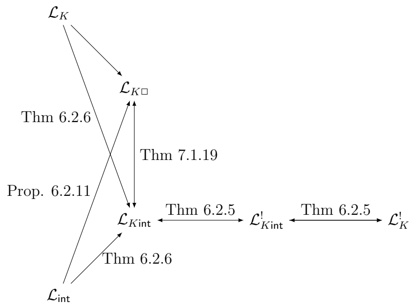
Figure 6.3: Expressivity diagram (Arrows point to the more expressive languages, and reflexive and transitive arrows are omitted. Arrows without tags can be obtained as easy consequences from the others.)
