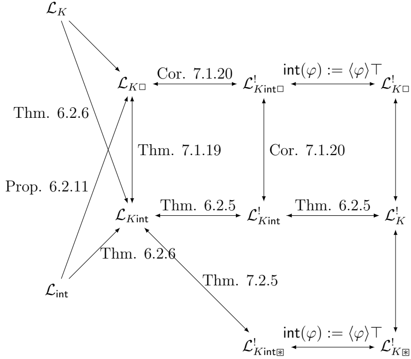
Figure 7.2: Expressivity diagram-updated with \boxtimes (Arrows point to the more expressive languages, and reflexive and transitive arrows are omitted. Arrows without tags can be obtained as easy consequences from the others.)
