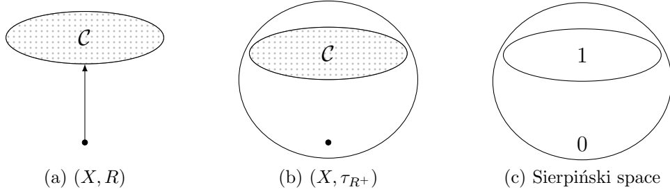
Figure 4.3: From pins to Alexandroff h.e.d. spaces
