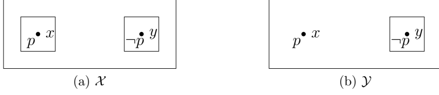
Figure 6.1: Squares represent the open sets in the corresponding topologies.
