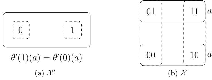
Figure 8.7: The straight round circles show the neighbourhoods of agent a , and the dashed ones are for agent b .
