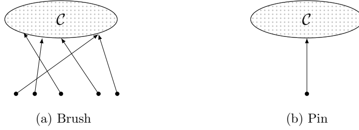
Figure 4.2: An example of a brush and of a pin, where the top ellipses illustrate the final clusters and an arrow relates the state it started from to every element in the cluster.
