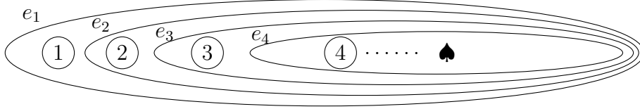
Figure 5.2: \mathfrak{M} = (\mathbb{N} \cup \{\spadesuit\}, \mathcal{E}_0, V)
