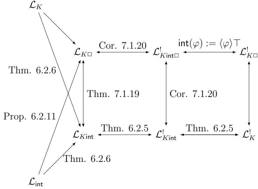
Figure 7.1: Expressivity diagram—updated with \square (Arrows point to the more expressive languages, and reflexive and transitive arrows are omitted. Arrows without tags can be obtained as easy consequences from the others.)
