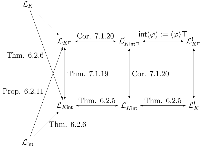
Figure 7.1: Expressivity diagram-updated with \Box (Arrows point to the more expressive languages, and reflexive and transitive arrows are omitted. Arrows without tags can be obtained as easy consequences from the others.)
