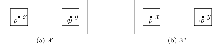
Figure 6.2: Squares represent the open sets in the corresponding topologies.
