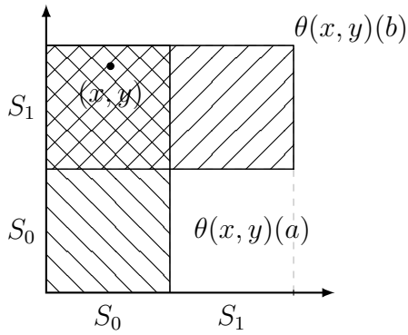
Figure 8.4: Initial situation where a knows the 1st bit of x is 0 and b knows the first bit of y is 1, and both are ignorant about the other's bit. We have \theta((x, y))(a) = S_0 \times \{0, 1\}^\infty and \theta((x, y))(b) = \{0, 1\}^\infty \times S_1 .
