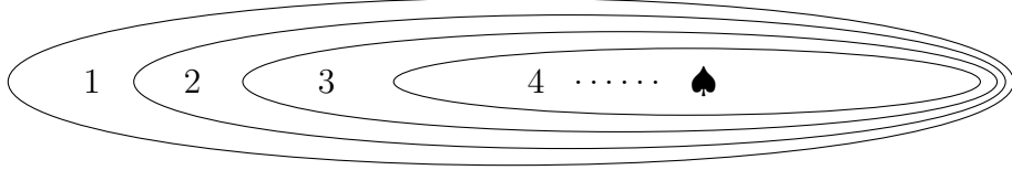
Figure 5.3: \mathfrak{M}' = (\mathbb{N} \cup \{\spadesuit\}, \mathcal{E}'_0, V)
