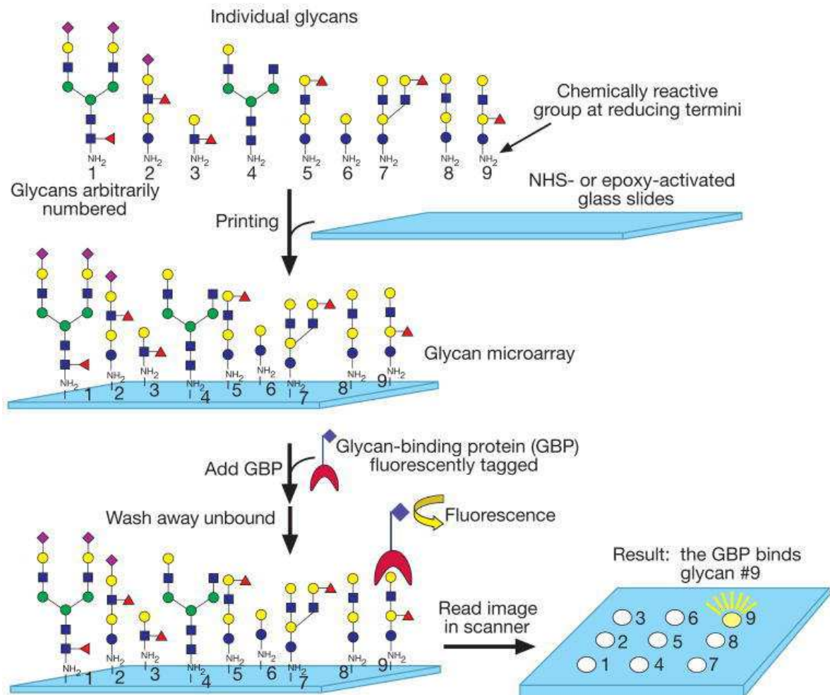
Figure 17: schematic overview of printed glycan microarrays. The glycans are covalently bound to NHS activated glass slides via a free amine at their reducing end. The glycan binding protein (GBP) is detected by fluorescence. It may be labelled directly or detected using fluorescently labelled secondary reagents. Picture reproduced from (Varki et al. 2009)
