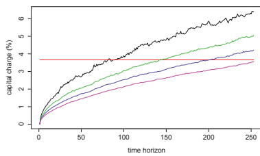
Figure 2.32: GARCH CC
