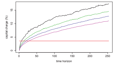
Figure 2.41: ICA CC
