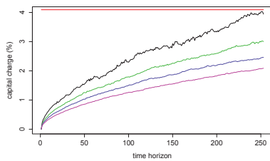
Figure 2.35: GARCH CC
