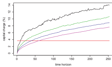
Figure 2.33: PCA CC
