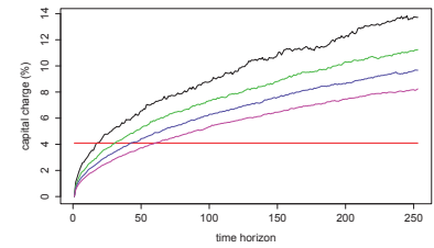
Figure 2.44: ICA CC
