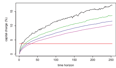
Figure 2.34: ICA CC
