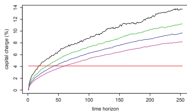
Figure 2.37: ICA CC
