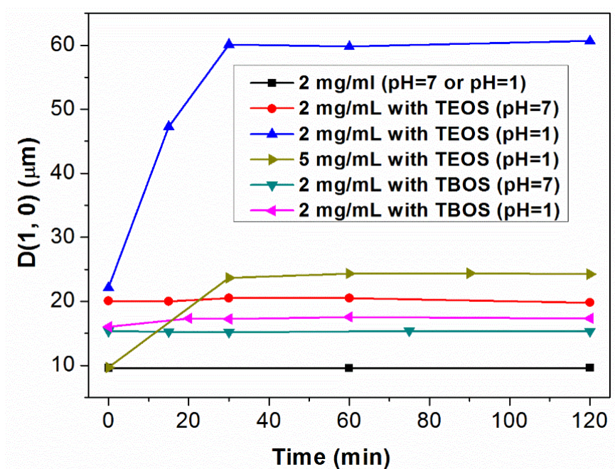
Figure 6.11. Evolution with time of the number-average diameter D(1,0) of the emulsion droplets in the Pickering systems containing TEOS or TBOS precursors ( \text{pH} = 1 or 7 ; [\text{Cin-CNC}] = 2 or 5 \text{ mg/mL} ).
