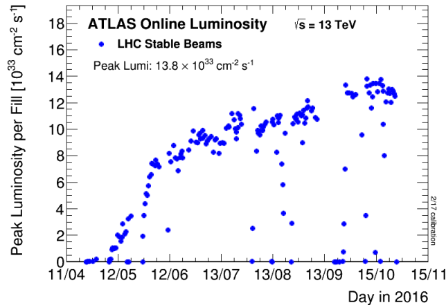
Figure 2.2: The peak instantaneous luminosity delivered to ATLAS during stable beams for pp collisions at 13 TeV centre-of-mass energy is shown for each LHC fill as a function of time in 2016.
