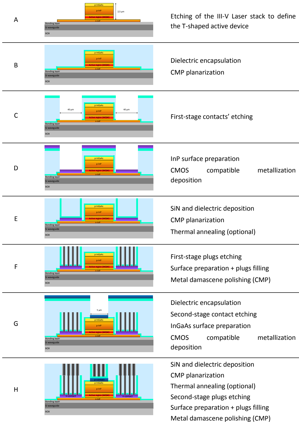
Figure 2.3: Si-compatible process flow for the integration of the contacts on a III-V laser in the framework of Silicon Photonics. Note that the width of the laser is about 100 μm while its longitudinal dimension is approximately 500 μm.
