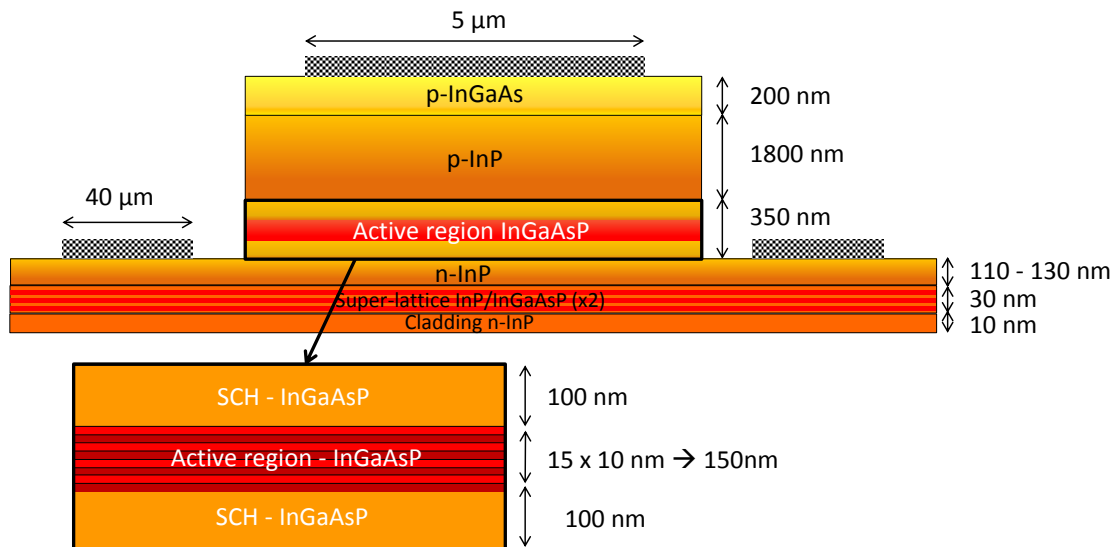
Figure 1.8: InP/InGaAsP-based laser structure used in STMicroelectronics and in the CEA-LETI. Note that the laser length is about 500 μm.
