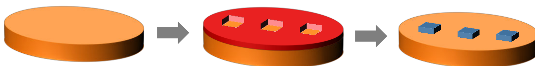
Figure 1.12: Schematic representation of a lift-off integration of contacts.
