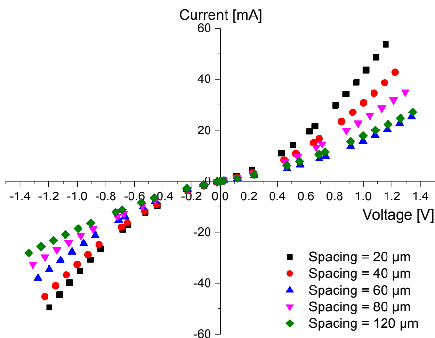
Figure 4.22: I(V) curves corresponding to each spacing of the \text{Ti}/\text{InP} system annealed at 550^\circ\text{C} for 60 seconds.
