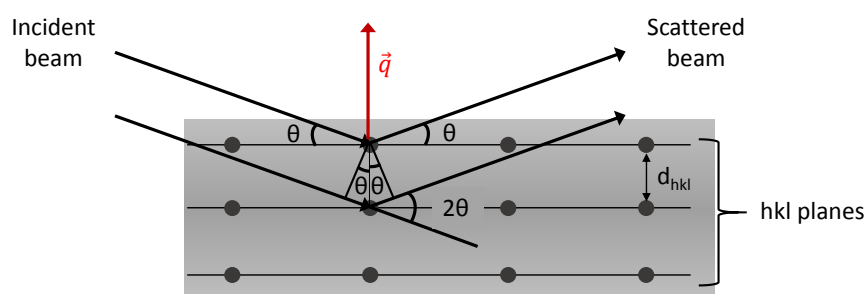
Figure 3.5: Schematic representation of diffraction of an incident X-Ray beam on atomic planes.
