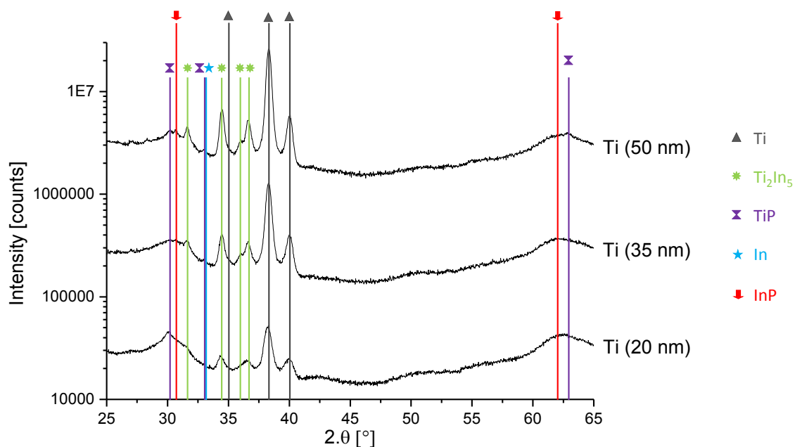
Figure 3.36: XRD detexturation pattern of the as deposited TiN (7 nm)/Ti (20 nm, 35 nm and 50 nm)/InP samples.
