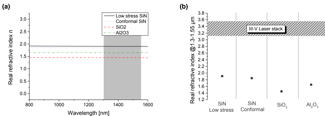
Figure 2.10: Real refractive index of low stress SiN, conformal SiN, SiO 2 and Al 2 O 3 (a) plotted as a function of the wavelength between 0.8 and 1.6 μm and (b) between 1.3 and 1.55 μm and comparison with the refractive indexes of the III-V laser stack.
