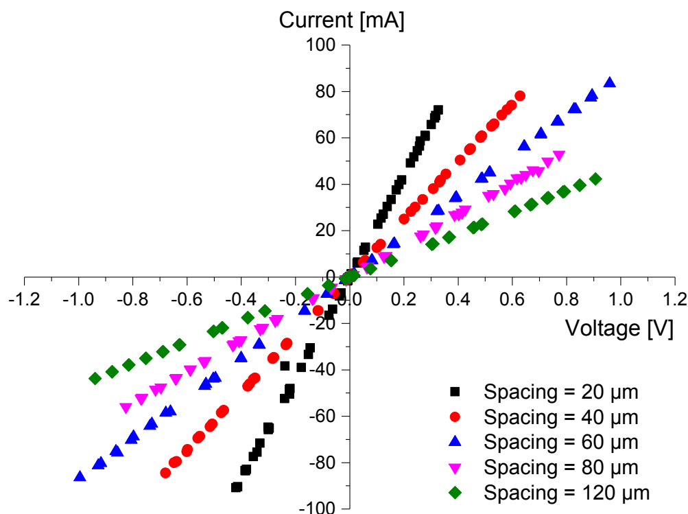
Figure 4.23: I(V) curves corresponding to each spacing of the as deposited \text{Ni}_2\text{P}/\text{n-InP} system.
