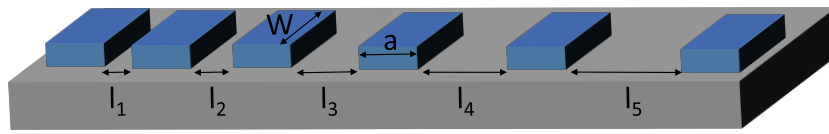
Figure 4.11: Schematic representation of a TLM structure. All contacts are identical (width W and length a , and separated by an increasing distance l_i ).
