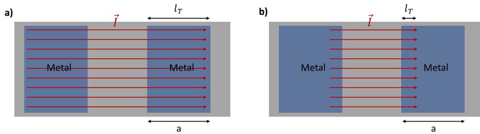
Figure 4.14: Illustration of the transfer length in the case where (a) L_T \sim a and (b) L_T \ll a .
