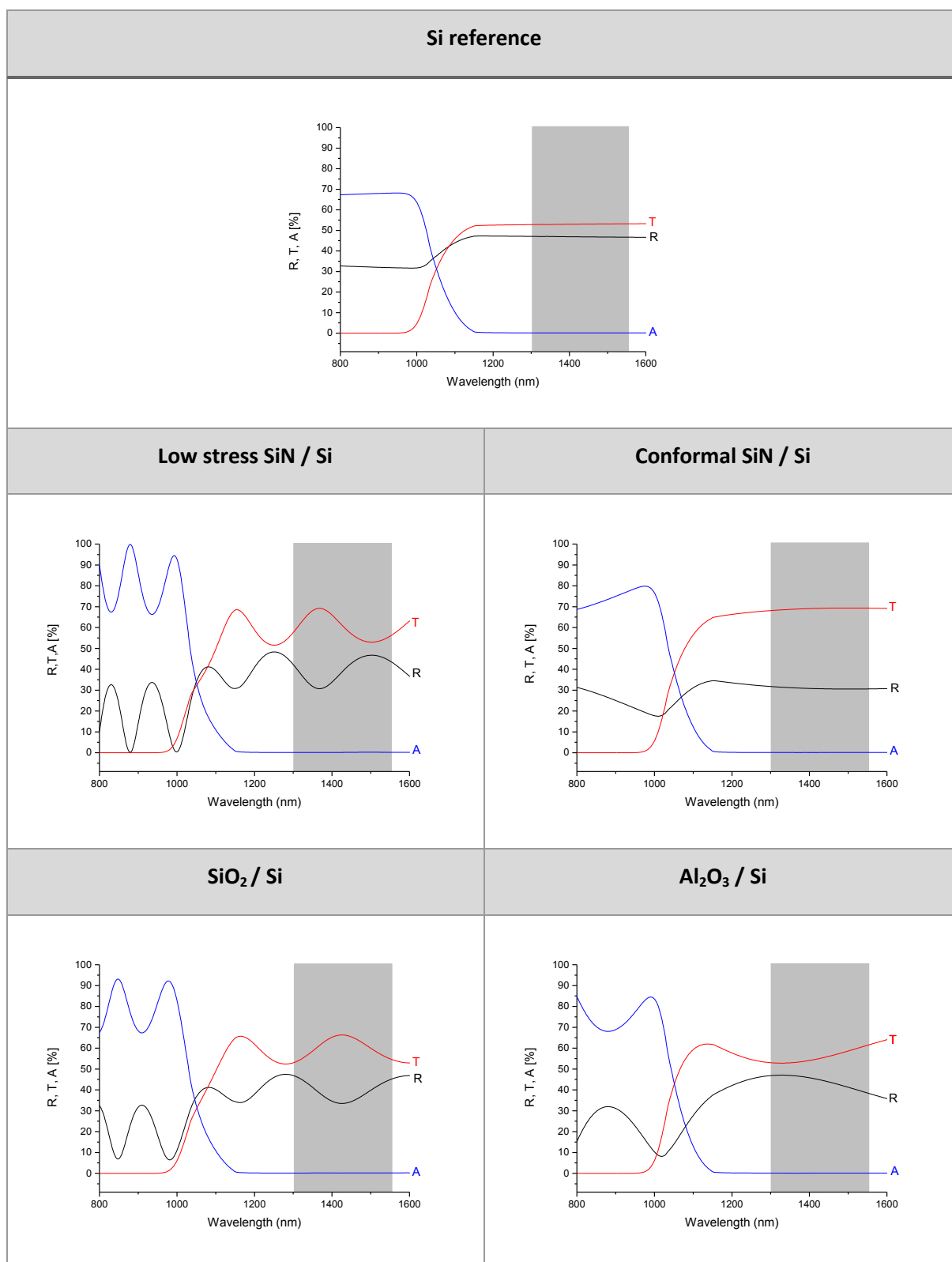
Figure A1. 2: Measured R and T and calculated A coefficients @ 0.8 – 1.6 μm for reference Si, low stress SiN, conformal SiN, SiO 2 and Al 2 O 3 .
