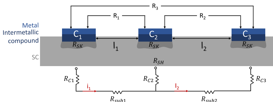
Figure 4.18: Experimental setup used for the determination of the end resistance (Setup B).
