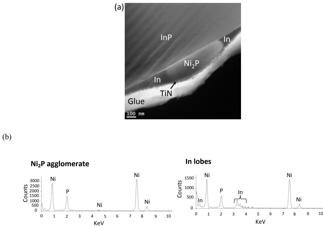
Figure 3.18: (a) Cross sectional bright field TEM image of the Ni/InP sample after a 60-second RTP at 550 °C; (b) EDS spectra of the the central Ni 2 P grain and the two In lobes.
