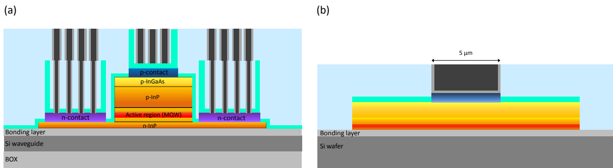
Figure 2.19: Schematic representation of the integrated contact metallization and plug contacts (a) on the III-V laser and (b) (b) on the morphological test structures.
