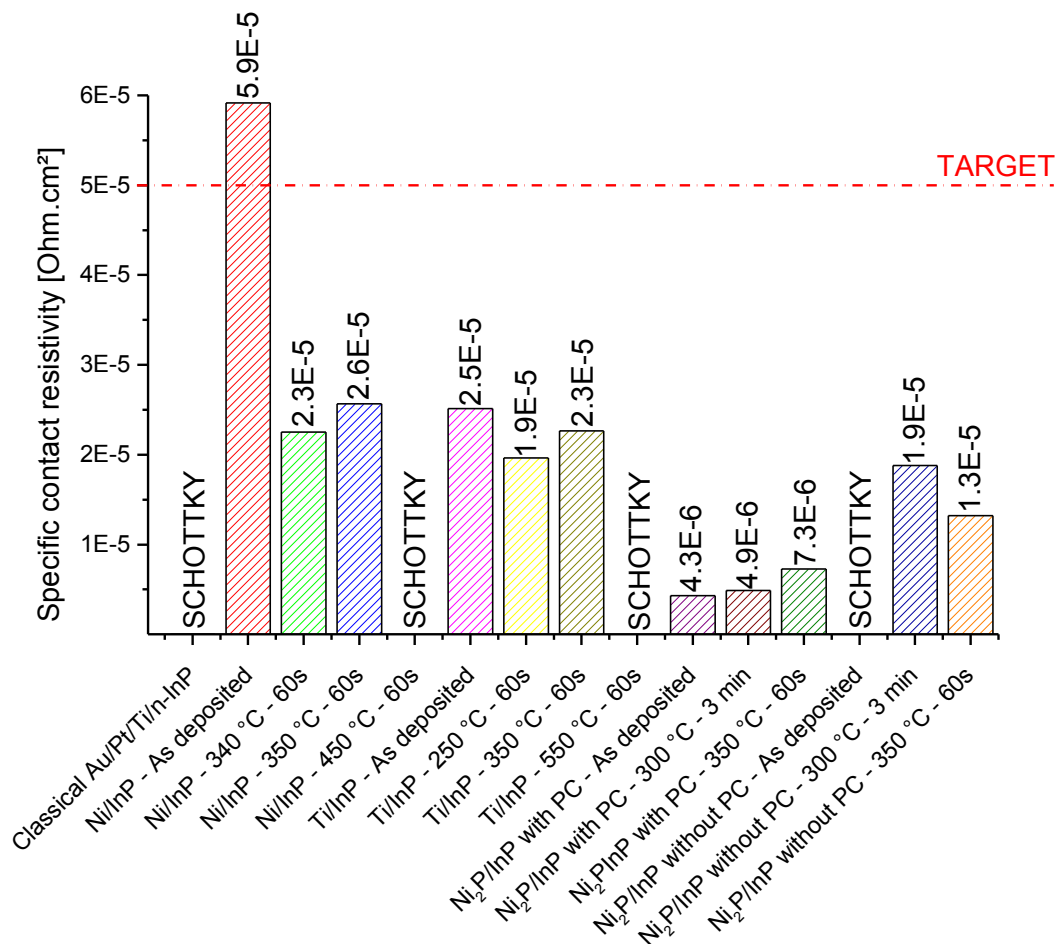
Figure 4.32: Specific contact resistivities of Ni and Ti-based metallizations to n-InP ( N_D = 3 \times 10^{18} \text{cm}^{-3} ). When encountered, PC stands for in situ \text{Ar}^+ pre clean.
