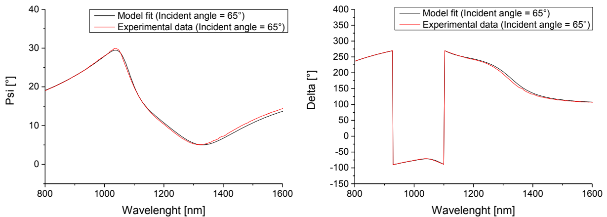
Figure A2. 2: Experimental data and corresponding fits using the Tauc-Lorentz model of \psi and \Delta angles.
