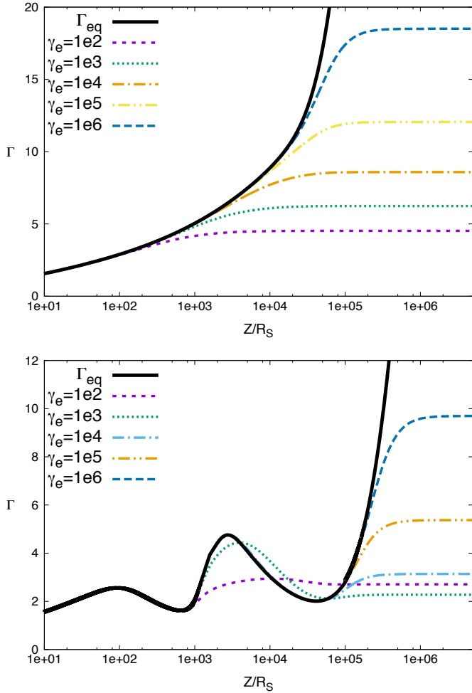
Fig. 13. Actual value of \Gamma_b as a function of the altitude in the jet Z/R_S for several values of \gamma_e . Top: standard accretion disk alone with an outer radius of 4e5R_S . Bottom: accretion disk, dusty torus, and broad line region with parameter values from Table 1.
