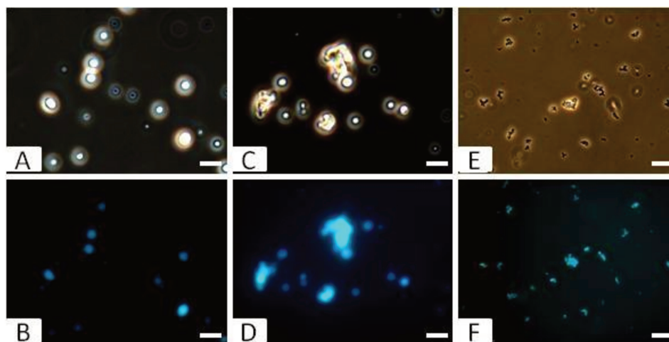
Figure 4.4. Optical microscopy images in phase contrast mode (A, C, E) and epifluorescence mode (B, C, E) for mixtures containing 0.5 mM of \alpha -LG, 0.05 mM of LF and different concentrations of ANS according to mixing order 2. Different ANS/LF molar ratios were tested: 25 (A, B), 30 (C, D) and 40 (E, F).
