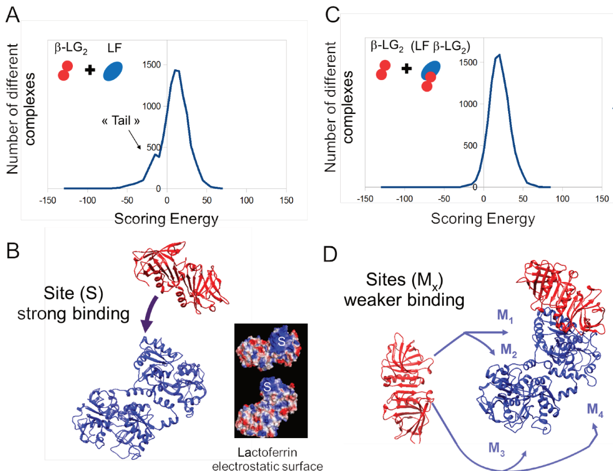
Figure 3.8. Molecular docking between \beta -LG 2 and LF (A, B), and between \beta -LG 2 and already formed LF \beta -LG 2 complex (C, D).
