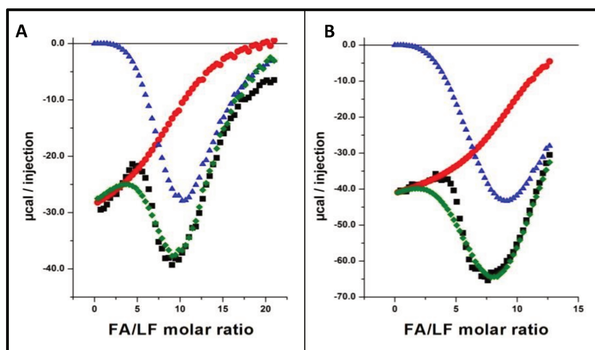
Figure 4.14. Superimposition of experimental binding isotherm (■), theoretical FA/LF binding isotherm (●), theoretical energy contribution of the LF self-association (▲) and the theoretical global isotherm (binding + self-association) (◆). Results were obtained from the raw ITC data acquired at 20°C and (A) [LF] = 0.01mM and (B) [LF] = 0.02mM.
