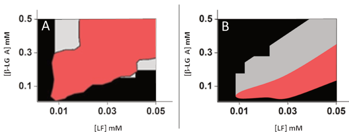
Figure 5.4. Phase boundaries of complex coacervation of LF with \beta -LG A at pH 5.5. (A) native non lactosylated sample; (B) lactosylated sample (lactosylation rate \approx 30 %). Black zone: domains without detectable supramolecular structure; Gray zone: aggregation domain; Salmon zone: coacervation domain.
