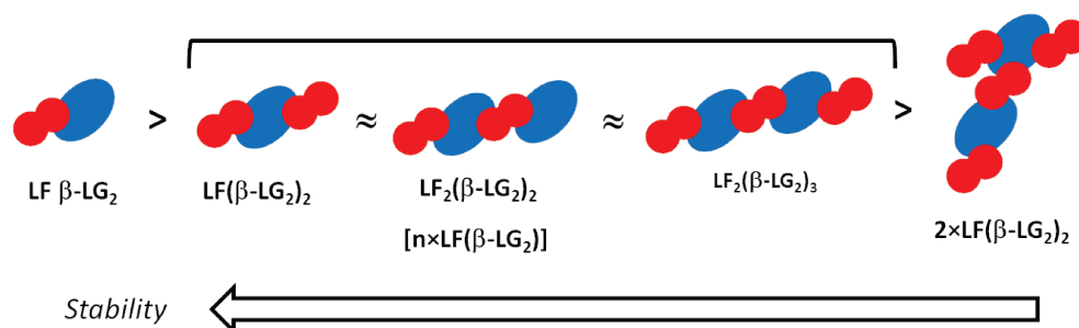
Figure 5.1. Relative stability of different \square -LG 2 - LF complexes according to the docking simulations. Blue ellipse: lactoferrin; red circle: \square -LG.
