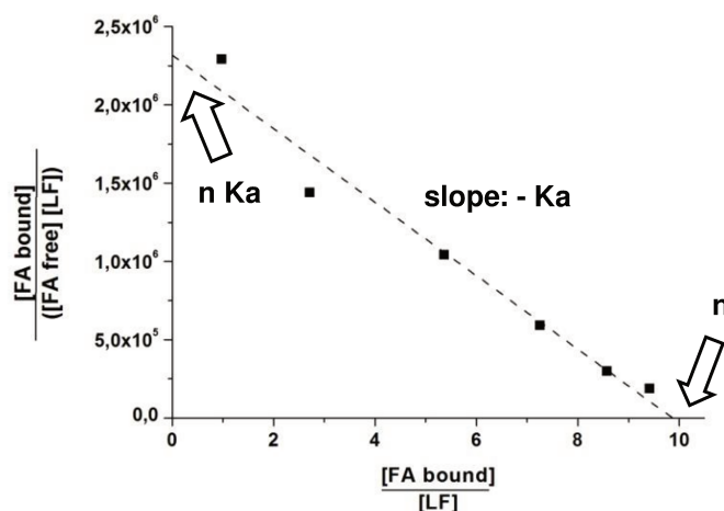
Figure 4.9. Scatchard plot for the interaction between LF (10 \mu\text{M} ) and FA (0-150 \mu\text{M} ) in 10 mM MES buffer, pH 5.5.
