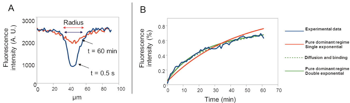
Figure 3.10. FRAP analysis of the FITC labeled \alpha -LG within the coacervate phase.
