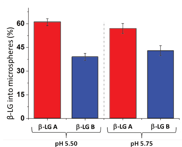
Figure 3.5. Average of the relative proportion of \beta -LG A and \beta -LG B quantified in the coacervation domains of mixture containing LF + \beta -LG A+B at pH 5.50 and pH 5.75 in 10 mM MES Buffer.
