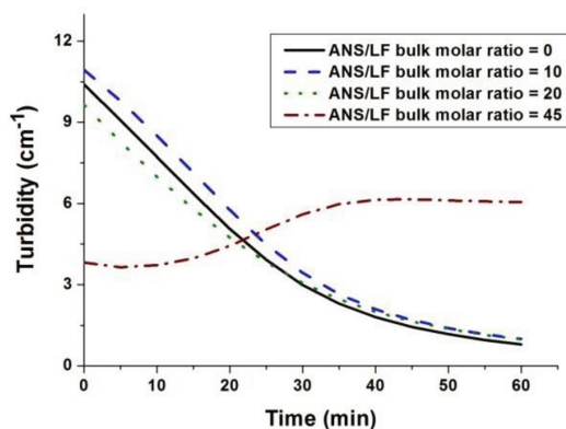
Figure 4.3. Evolution of the turbidity of mixtures containing 0.5 mM of \square -LG, 0.05 mM of LF and variable concentrations of ANS. Different ANS/LF molar ratios were tested: 0 (straight line), 10 (dashed line), 20 (dotted line) and 45 (dash-dotted line). These results correspond to mixtures performed according to the order 2 ( \square -LG+ANS+LF), given than the same behavior was found for orders 1 and 3.
