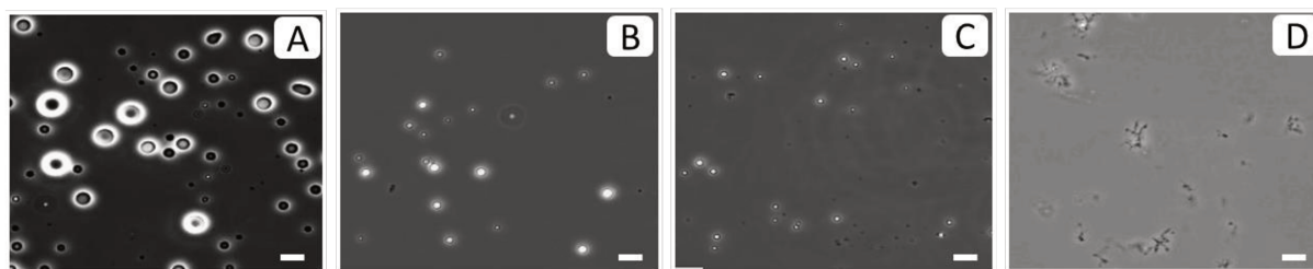
Figure 4.18. Optical microscopy images in phase contrast mode for mixtures containing 0.16 mM of \alpha -LG, 0.016 mM of LF and different concentrations of FA according to mixing order 2. Different FA/LF molar ratios were tested: (A) 0, (B) 1, (C) 2 and (D) 10. Barre = 10 \mu m.
