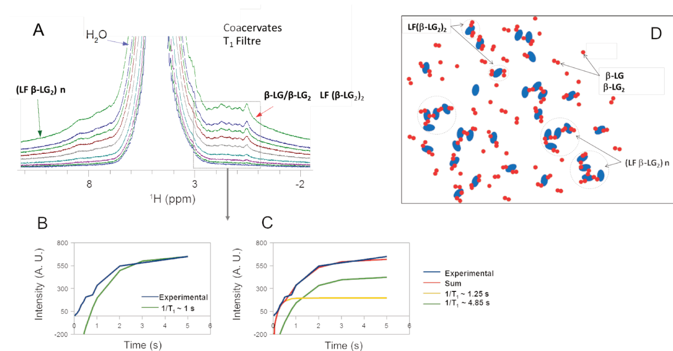
Figure 3.12. Assignment of NMR signals to different complexes in the coacervates.
