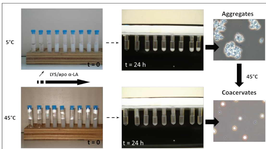
Figure 2.7. Summary of the interactions, supramolecular structure formation and phase separation of apo \alpha -LA-LYS mixture at 5 and 45 °C ranging from 0.05 to 2 LYS \alpha -LA molar ratio at fixed \alpha -LA concentration (0.266 mM) (adapted from Nigen et al. [98]).
