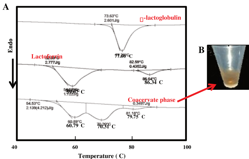
Figure 3.13. (A) DSC thermograms of the \beta -LG (~300 g/L), LF (~ 300 g/L) and the coacervate phase ( \beta -LG ~150 g/L + LF ~150 g/L). (B) Image of the coacervate phase.
