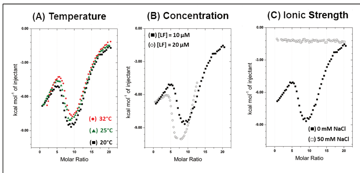
Figure 4.8. Experimental binding isotherms of the interaction of FA with LF at various: (A) Temperatures, titration of LF 0.01 mM with 1 mM FA; (B) Cell LF concentrations, titration with 1 mM FA at 20°C; (C) ionic strength, titration of LF 0.01 mM with 1 mM FA at 20°C.
