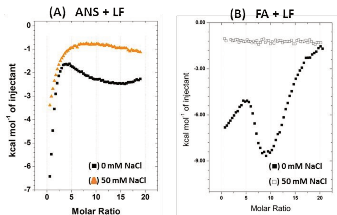
Figure 5.3. Binding isotherms of the titration of LF 0.05 mM with 4.25 mM ANS (A) and LF
