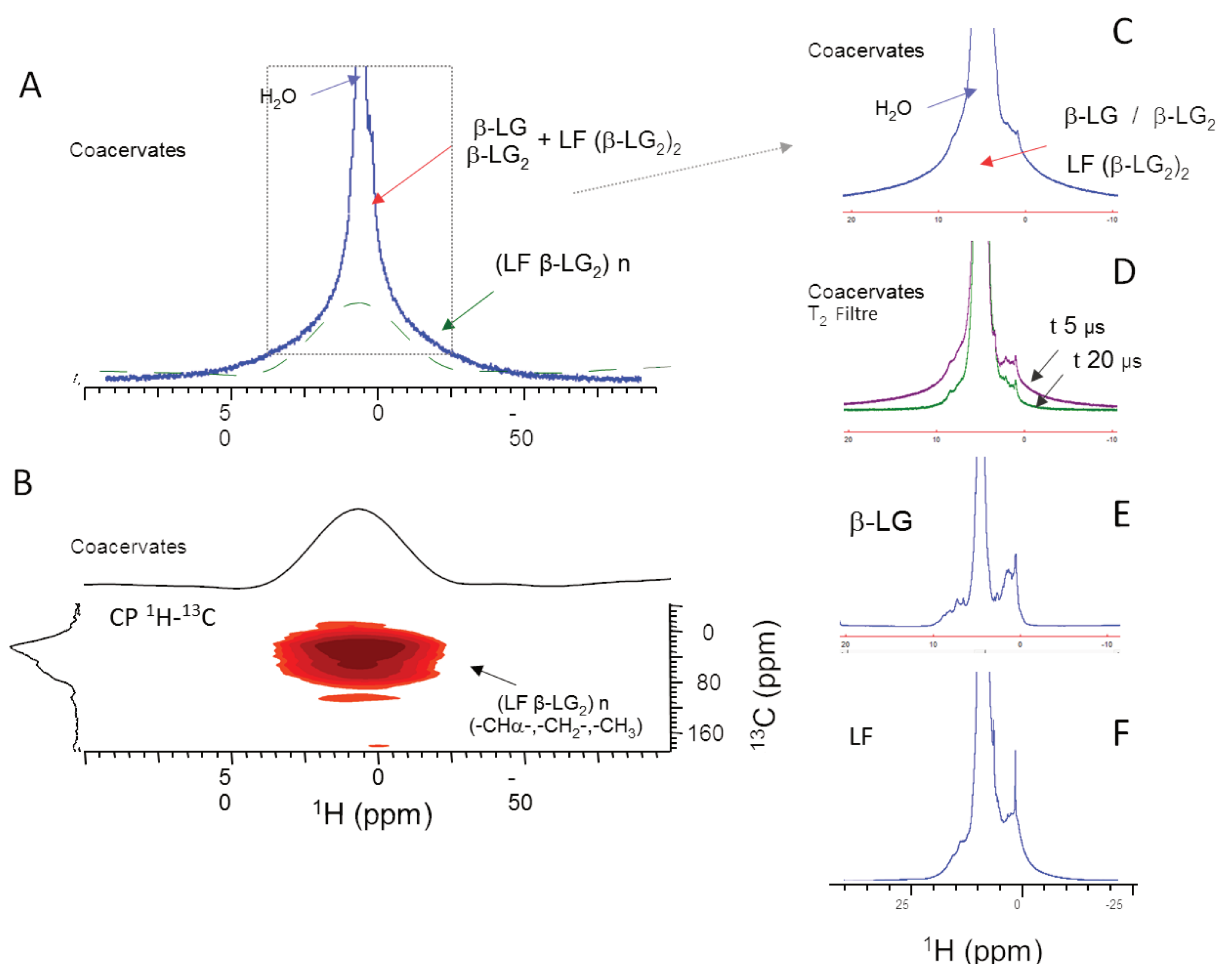
Figure 3.11. NMR signal Assignments.
