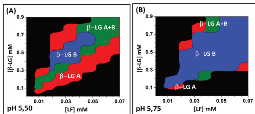
Figure 3.3. Superposition of the coacervation domains obtained by mixing LF and \beta -LG A (red), \beta -LG B (blue) or \beta -LG A+B (green) at pH 5.50 (A) and pH 5.75 (B). Co-assembly experiments were conducted at 25°C in MES buffer 10 mM.
