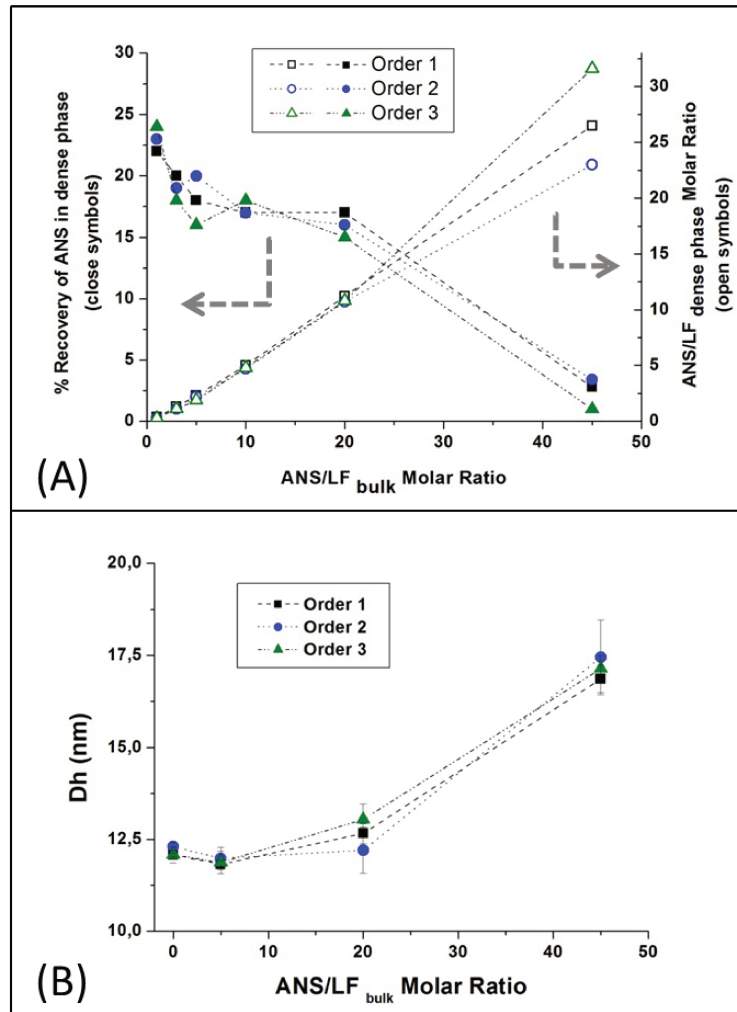
Figure 4.5. Evolution of recovered ANS (in %) and corresponding ANS/LF molar ratio in the dense phase (A) and of Dh of the structures remaining in the dilute phase after centrifugation of the mixtures (B) as a function of the initial ANS/LF molar ratio. Protein concentrations were 0.05 mM for LF and 0.5 mM for \beta -LG. The squares, circles and triangles correspond to mixing order 1, 2 and 3, respectively.
