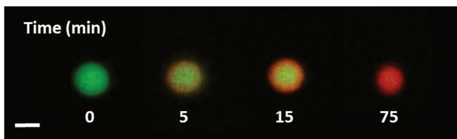
Figure 2.8. Internal dynamic of apo \alpha -LA-LYS coacervates and time-dependent protein exchange between coacervates and dilute phase (adapted from Nigen et al. [107]).
