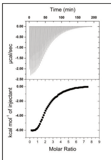
Figure 4.16. Raw data (upper panel) and binding isotherm (bottom panel) of the titration of 0.06 mM LF with successive injections of sodium citrate stock solution. The experiment was carried out at 25°C in 10 mM MES buffer, pH 5.5.
