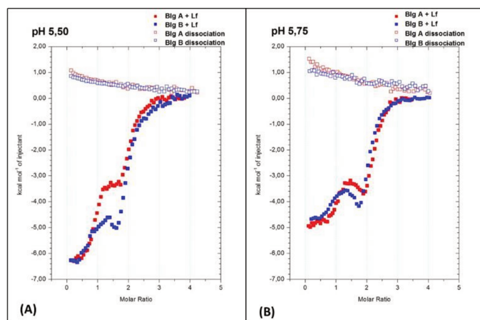
Figure 3.6. Binding isotherms of LF with (■) \beta -LG A or (■) \beta -LG B and dissociation isotherms upon dilution of (□) \beta -LG A and (□) \beta -LG B dimers. LF 0.1 mM was titrated with successive injections of \beta -LG 2 mM. ITC experiments were conducted at 25 °C in 10 mM MES buffer at pH 5.50 (A) and pH 5.75.
