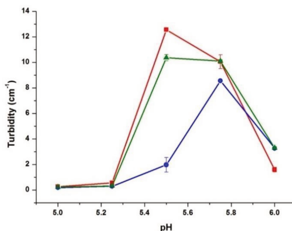
Figure 3.1. Change in turbidity of mixtures containing 40 \mu\text{M} of LF and 500 \mu\text{M} of (■) \beta\Pi\text{LG} A, (●) \beta\Pi\text{LG} B or (▲) \beta\Pi\text{LG} A+B in 10 mM MES buffer at different pHs.
