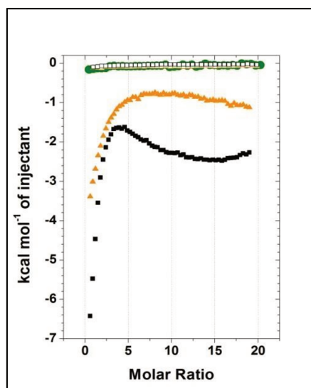
Figure 4.1. Binding isotherms of the titration of LF 0.05 mM and L-LG 0.05 mM with 4.25 mM ANS in MES buffer pH 5.5 at 25 °C. LF without (■) and with (▲) 50 mM NaCl; L-LG without NaCl (●). Injection of ANS in the MES buffer without (□) and with 50 mM NaCl (△).
