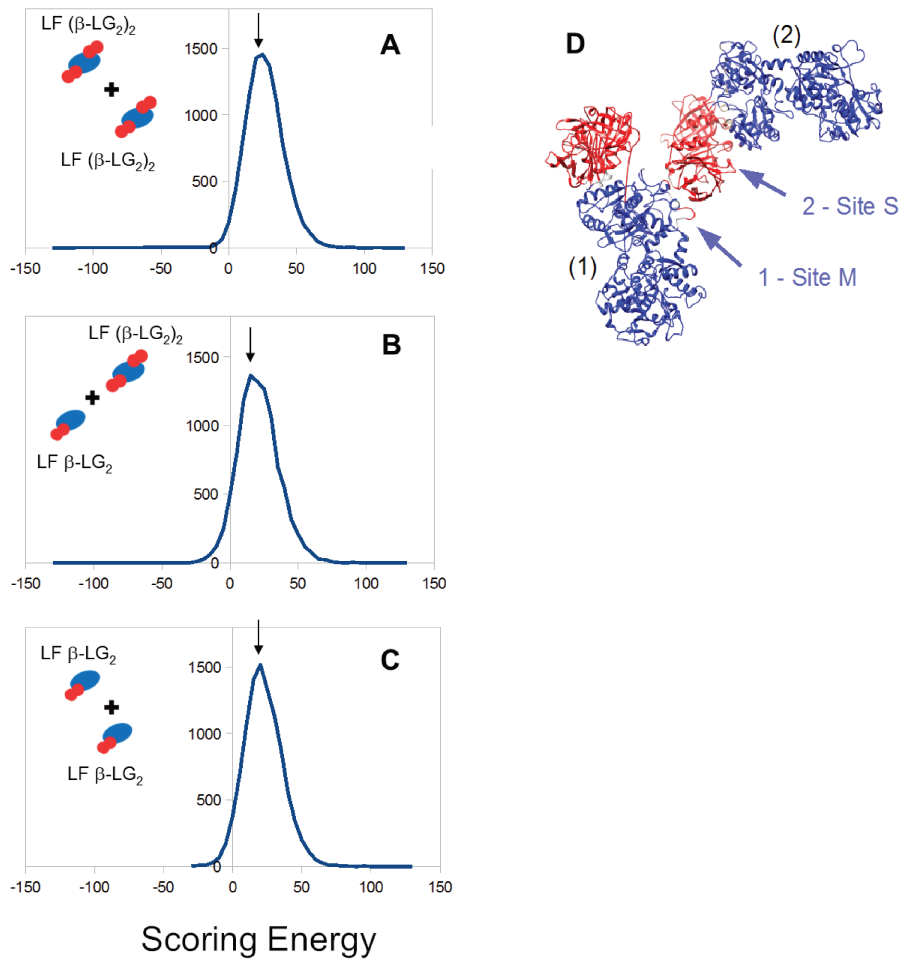
Figure 3.9. Molecular docking between trimeric and pentameric complexes of LF and \beta -LG 2 . Histogram of the energy scores of 10,000 large complexes formed by association of different complexes of \beta -LG 2 (red) and LF (blue). Docking results for the association between two LF( \beta -LG 2 ) 2 complexes (A), LF \beta -LG 2 and LF( \beta -LG 2 ) 2 (B) and two LF \beta -LG 2 complexes (C). (D)
