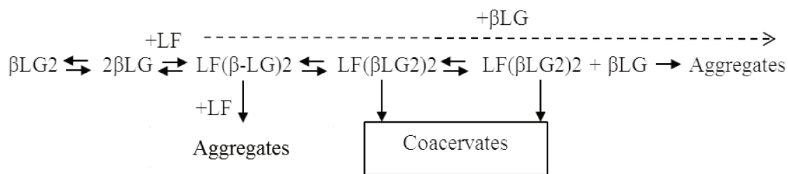
Figure 3.7. Proposed steps for the coacervation process involving LF and \beta -LG co-assembly.
