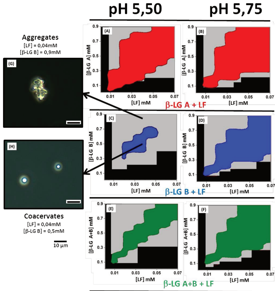
Figure 3.2. Phase boundaries of co-assembly of LF with \beta -LG isoforms at pH 5.50 and pH 5.75. (A,B): LF - \beta -LG A; (C,D): LF - \beta -LG B; (E,F) LF - \beta -LG AB. Black zones: domains without detectable supramolecular structures; Gray zones: aggregation domains. Red, Blue and Green zones: coacervation domains. Optical microscopy of aggregates formed by mixing for example 40 \mu M LF and 900 \mu M \beta -LG B at pH 5.50 (G) versus coacervates formed by mixing for example LF 40 \mu M and \beta -LG B 500 \mu M at pH 5.50 (H).
