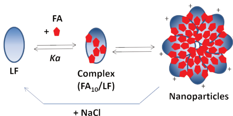
Figure 4.15. Proposed mechanism for the formation of folic acid/lactoferrin nanoparticles of finite size.
