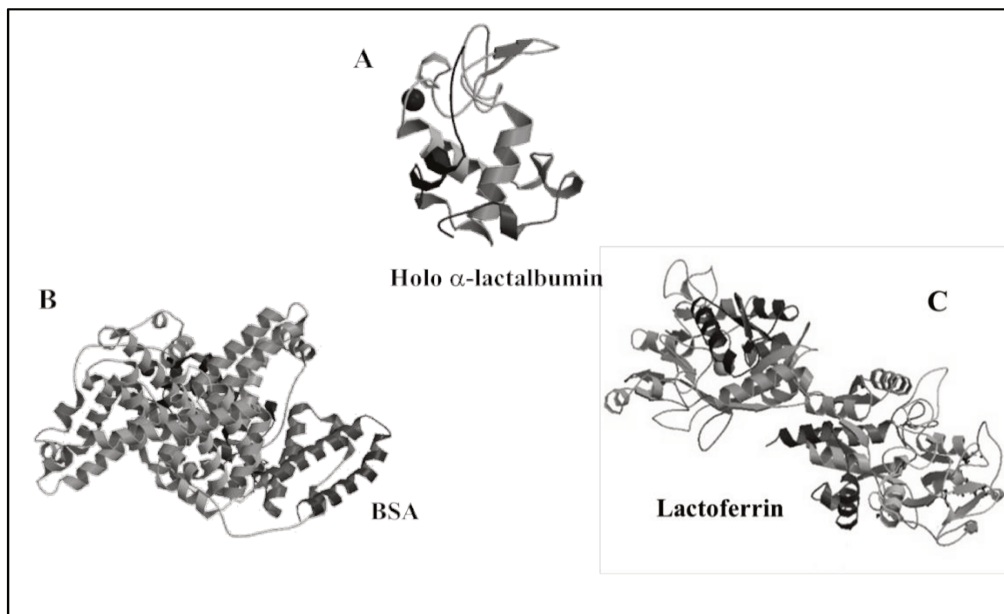
Figure 2.2. Tertiary structure of (A) \alpha -lactalbumin (RCSB PDB code: 1ALC), (B) BSA (RCSB PDB code: 3V03) and (C) Lactoferrin (RCSB PDB code: 1BLF).
