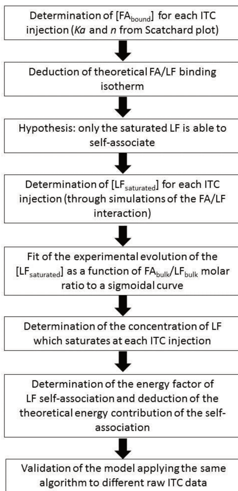
Figure 4.11. Algorithm used to develop the proposed model for FA binding to LF and subsequent self-association of FA/LF complexes.
