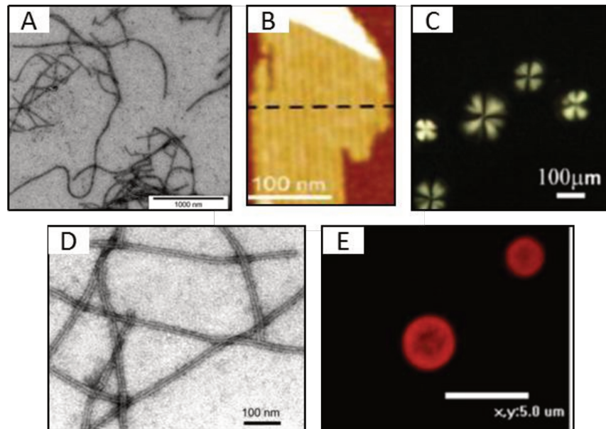
Figure 2.5. Different supramolecular structures obtained from whey proteins. (A) TEM micrograph of whey protein isolate (WPI) obtained from 2 % of WPI at pH 2 solution heated at 80 °C for 16h (adapted from Loveday et al. [104]). (B) AFM micrograph of \beta -LG ribbons obtained after heating \beta -LG (2 %wt.) at 90 °C and pH 2 (adapted from Lara et al. [95]). (C) Polarised light microscopy micrograph of \beta -LG spherulites (adapted from Krebs et al. [105]). (D) TEM micrograph of hydrolysed \alpha -LA nanotubes (adapted from Graveland-Bikker et al. [106]). (E) Confocal scanning laser micrograph of heteroprotein complex coacervates obtained from apo \alpha -LA (0.2 mM) and LYS (0.2 mM) mixture (adapted from Nigen et al. [107]).
