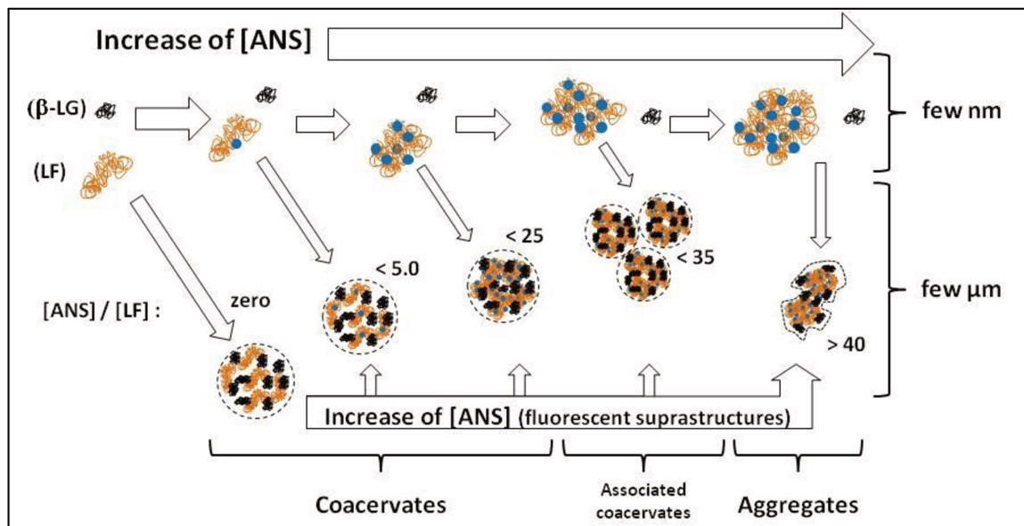
Figure 4.6. Proposed mechanism describing how increasing ANS concentration (represented by the blue circle) affects \beta -LG-LF coacervation process at constant protein concentration.
