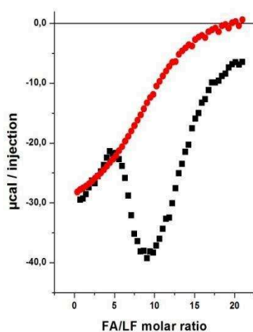
Figure 4.12. Superimposition of the experimental (■) and theoretical (●) FA/LF binding isotherms. Experimental titration of 0.01 mM LF was performed with FA in 10 mM MES buffer pH, 5.50, at 20°C.
