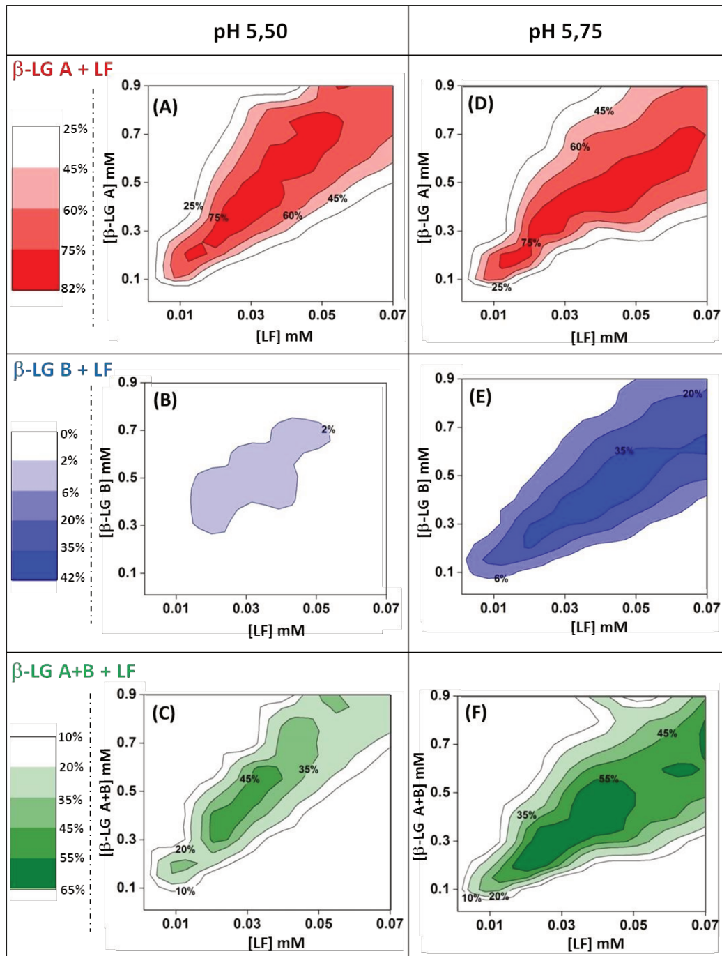
Figure 3.4. Fraction of LF recovered in the coacervates (dense phase) formed with \beta -LG A (A and D), \beta -LG B (B and E) or \beta -LG A+B (C and F) at pH 5.50 and pH 5.75 in 10 mM MES buffer and at 25°C.
