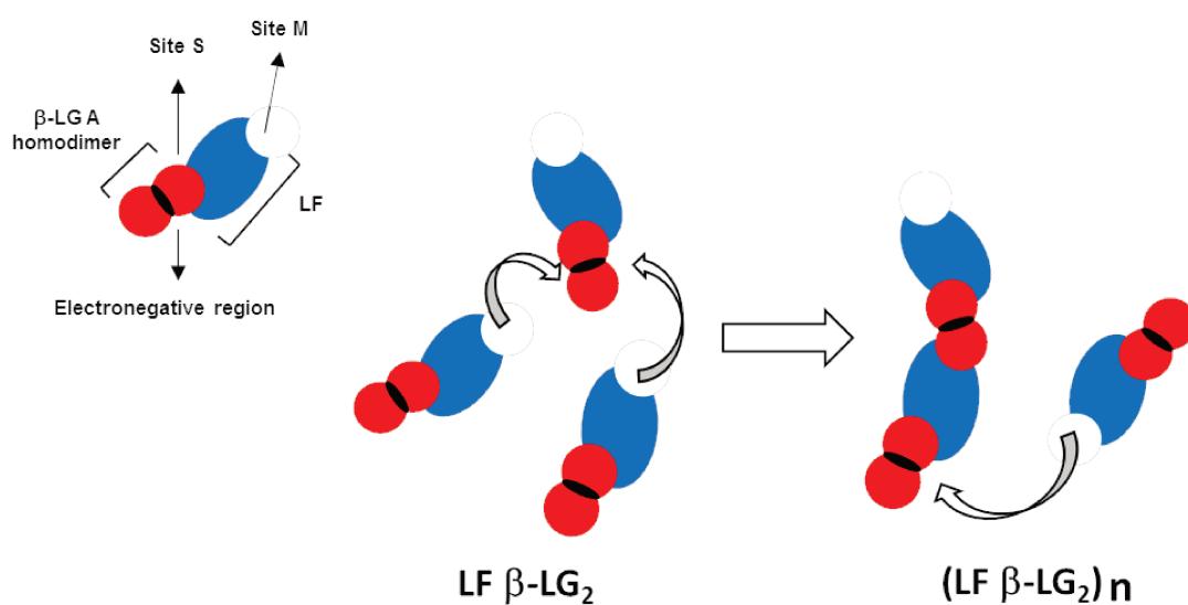
Figure 5.2. Hypothetic scheme of the self-assembly of trimers \text{LF } \beta\text{-LG}_2 formed by LF and \beta -LG A homodimers. Representation of the role of the electronegative region on the \beta -LG A homodimers interface promoting the self-assembly into coacervates.
