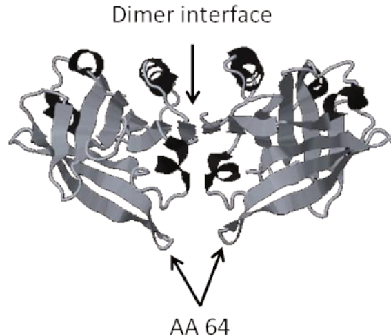
Figure 2.1. \beta -LG dimer (RCSB PDB code: 2Q2M). The arrows show the dimer interface and the position of the AA64, an important substitution between isoforms A and B.
