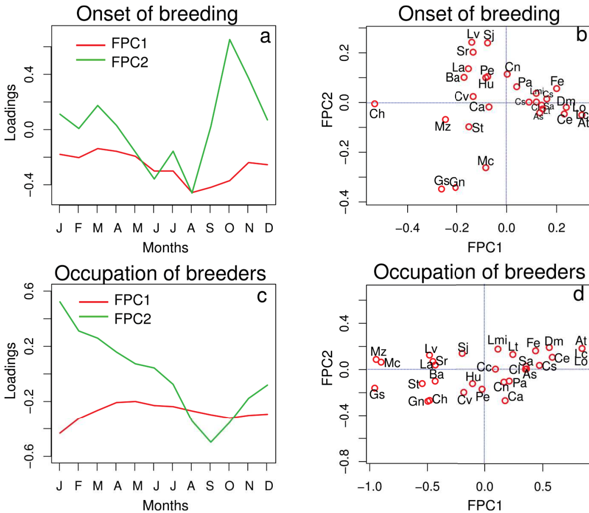
Figure 3.4. Functional Principal components of onset and occupancy of booby. Loadings of timing and magnitude of onset of breeding of pelican were represented on the left (a and c) and the bivariate plot of scores of each colony for FPC1 and FPC2 (b and d) were represented on the right. Extended names of the nesting sites are described in Appendix A.
