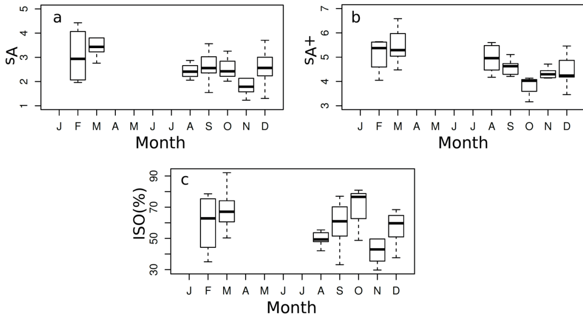
FIG. F2. Monthly variations of anchovy abundance (a) s_A , (b) s_{A+} and (c) index of space occupation (ISO). The boxplots were constructed from the monthly variations of the metrics between 6° and 14°S over the period 1999-2011.
