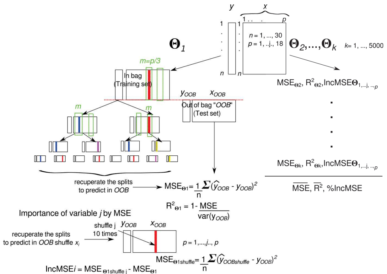
Figure C1. Schema of procedure in Random forest.
