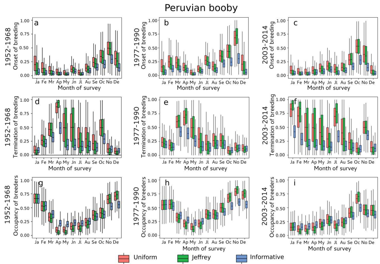
Figure S6. Output of a-c) onset, d-f) termination, and g-i) occupancy of breeding for Peruvian boobies for the periods 1952-1968, 1977-1990 and 2003-2014 with different hyperparameters: Uniform (red boxes), Jeffrey (green boxes) and Informative (blue boxes).
