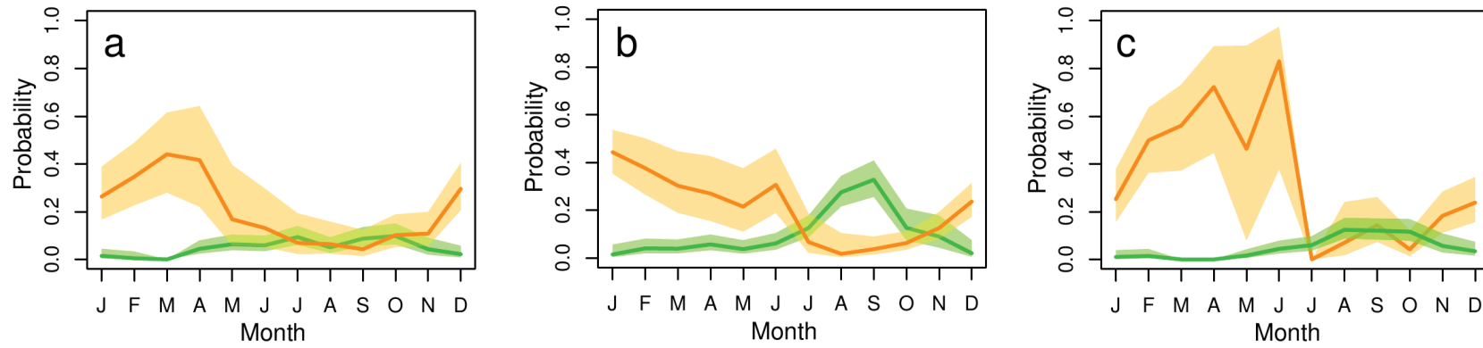
FIG. 11. Estimates of monthly probabilities of breeding onset (green solid line) and breeding termination (orange solid line) for (a) cormorants, (b) boobies and (c) pelicans in the Northern Humboldt Current System over 10 years. Shaded areas correspond to 95% confidence intervals.
