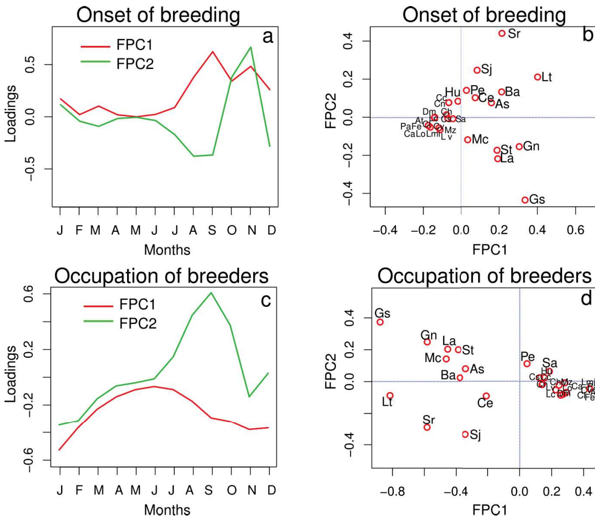
Figure 3.5. Functional Principal components of onset and occupancy of pelican. Loadings of timing and magnitude of onset of breeding of pelican were represented on the left (a and c) and the bivariate plot of scores of each colony for FPC1 and FPC2 (b and d) were represented on the right. Extended names of the nesting sites are described in Appendix A.
