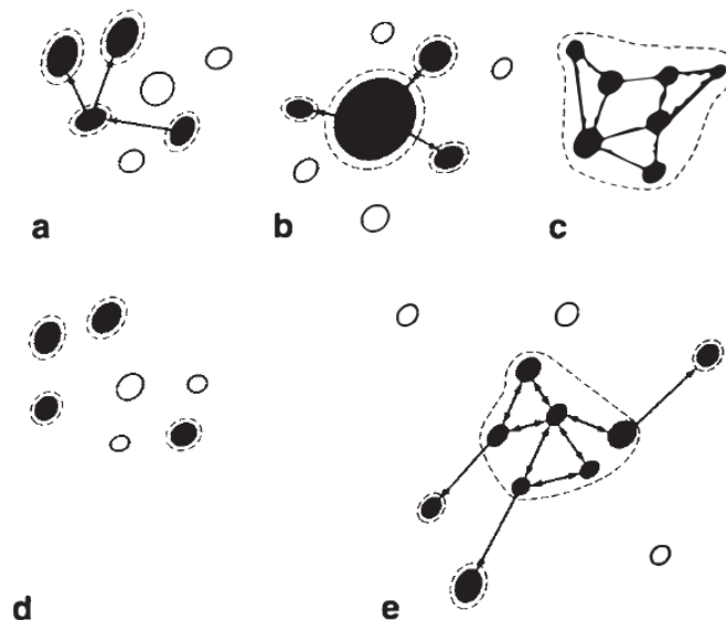
Figure 1.36. Different types of metapopulation. Filled circles represent occupied habitat patches; empty circles represent vacant habitat patches; dotted lines represent boundaries of local populations; arrows represent dispersal. a) Classic boundaries of Levins; b) mainland-island; c) patchy population; d) nonequilibrium metapopulation; e) intermediate case combining features of (a), (b), (c), and (d). Source Harrison & Taylor 1997.
