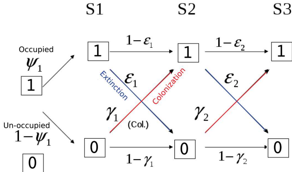
Figure 1.37. Schema of the estimation of parameters in multiseason occupancy models. \Psi is the initial occupancy ( \psi=1 , or 1-\psi=0 ), then in the next seasons (S1, S2 and S3) extinction ( \text{Pr}(h_t=10)=\epsilon ) or colonization ( \text{Pr}(h_t=01)=\gamma ) parameter are estimated.
