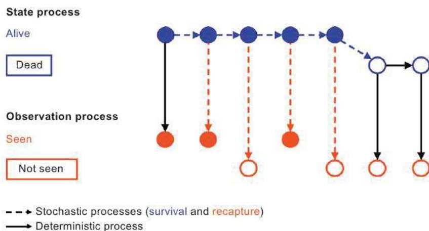
Figure 5.2. Example of the state and observation process of a marked individual over time for the Cormack Jolly Seber model. The sequence of true states in this individual is z = [1, 1, 1, 1, 1, 0, 0] , and the observed capture-history is y = [1, 1, 0, 1, 0, 0, 0] . Source Kéry & Schaub 2012.
