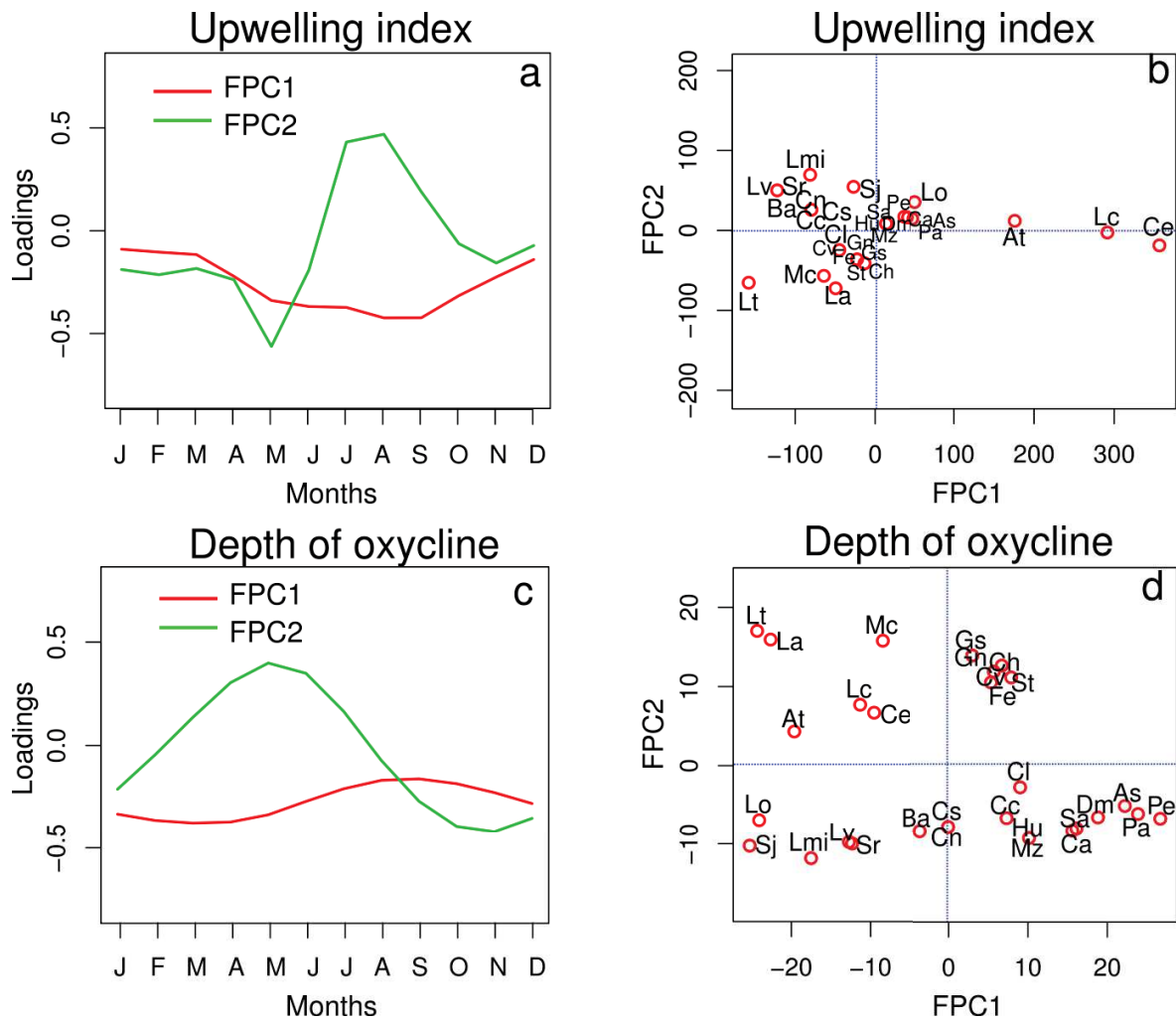
Figure 3.2. Functional Principal components of Upwelling index and Depth of oxycline. Loadings (a and c) were represented on the left and the bivariate plot of scores of each colony for FPC1 and FPC2 (b and d) were represented on the right. Extended names of the nesting sites are described in Appendix A.
