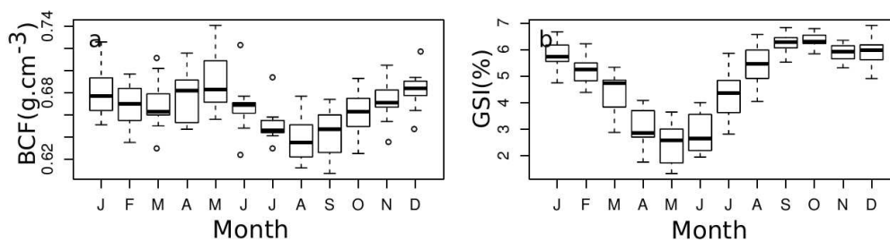
FIG. G1. Monthly variations of anchovy physiological condition metrics (a) body condition factor, BCF; and (b) Gonado-somatic index: GSI. Boxplots were constructed from monthly variations of the metrics between the 6^\circ to 14^\circ S over the 2000-2012 period.
