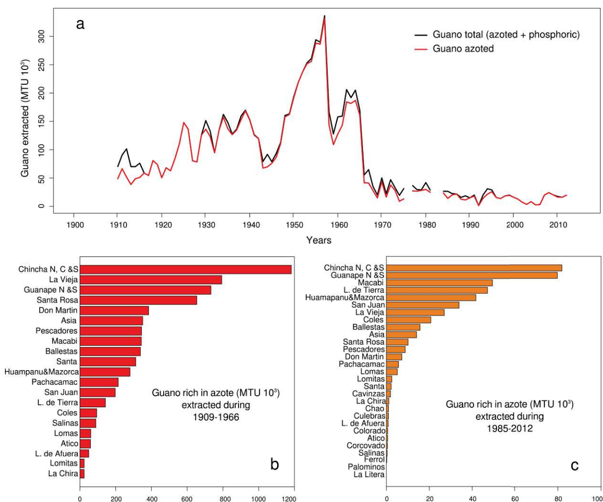
Figure 1.16. a) Guano extracted per year during the last century in the main seabird colonies (Data source AGRORURAL), b) Guano extracted by nesting site from 1909-1966, period of large abundance of anchovy and under the CAG administration and c) guano extracted during 1985-2012, period of less abundance and posterior recuperation of anchovy but not of seabirds. Data source for b and c were Cushman 2003 and AGRORURAL pers.com.
