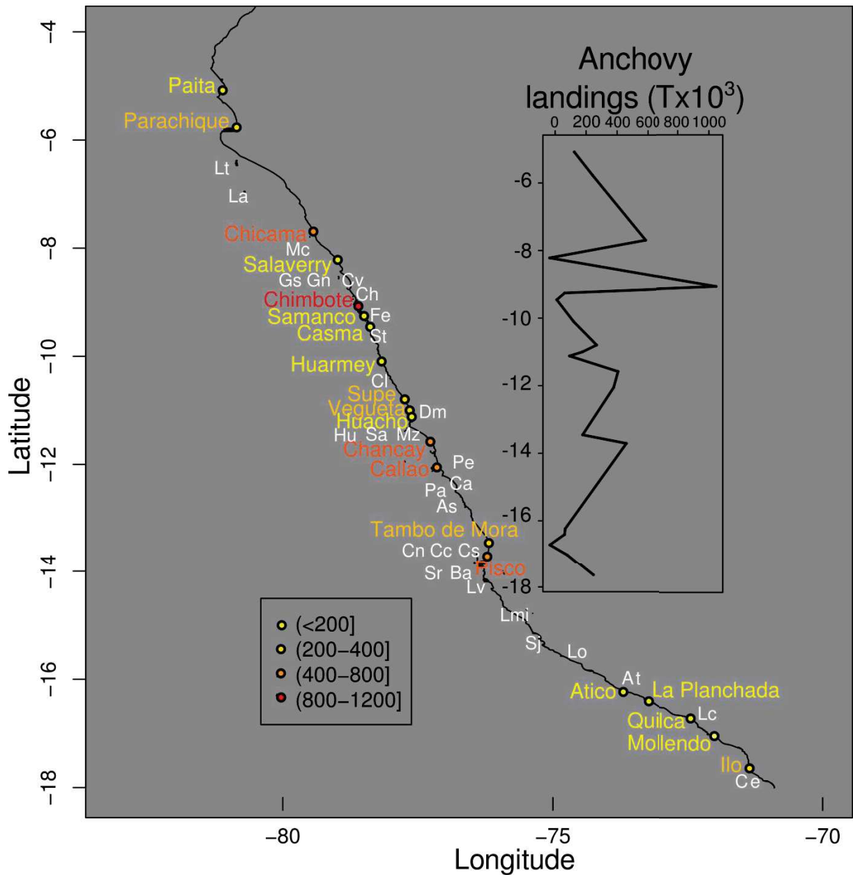
Figure A2. Main ports of landings of anchovy, in gray letters nesting colonies near the ports.
