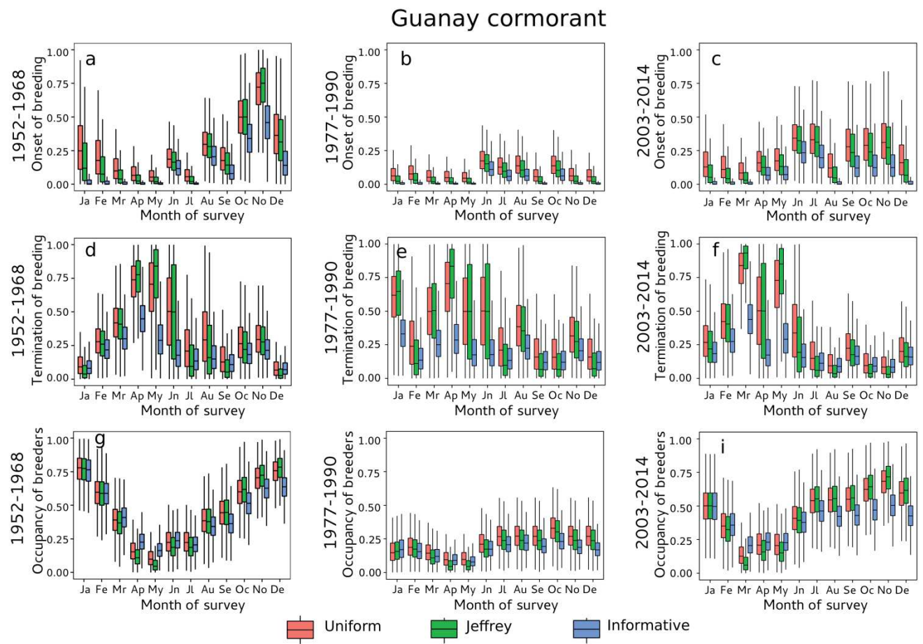
Figure S5. Output of a-c) onset, d-f) termination, and g-i) occupancy of breeding for Guanay cormorants for the periods 1952-1968, 1977-1990 and 2003-2014 with different hyperparameters: Uniform (red boxes), Jeffrey (green boxes) and Informative (blue boxes).
