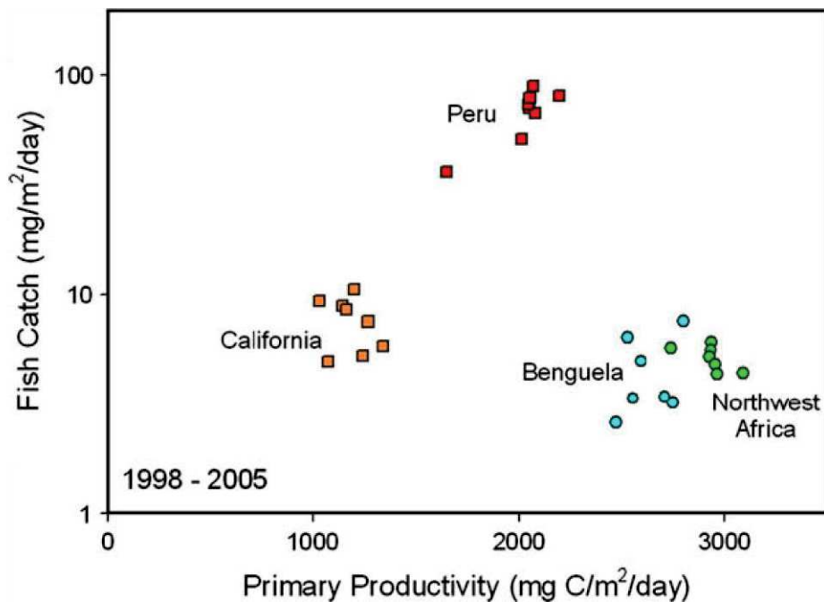
Figure 1.2. Fish catch versus primary productivity for the four main eastern boundary coastal upwelling ecosystems for the years 1998–2005. It was assumed that the reported fish catches (Fish and Agriculture Organization, FAO) were made within 100 km from the coast. The catches were then normalized by area. Primary productivity was estimated from satellite remote sensing of chlorophyll and the Behrenfeld and Falkowski (1997) model. Even during the El Niño year of 1998 Peru fish catch still exceeded that from the other areas by several fold. Is Peru exceedingly efficient in the transfer of primary production to fish or are Benguela and Northwest Africa exceedingly inefficient? Source Chavez et al. 2008.
