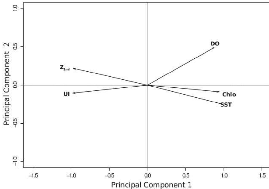
FIG. E2. Results from a principal component analysis of oceanographic covariates. The x-axis represents the first principal component (89.1% of the variance) and the y-axis represents the second principal component (7.3% variance).
