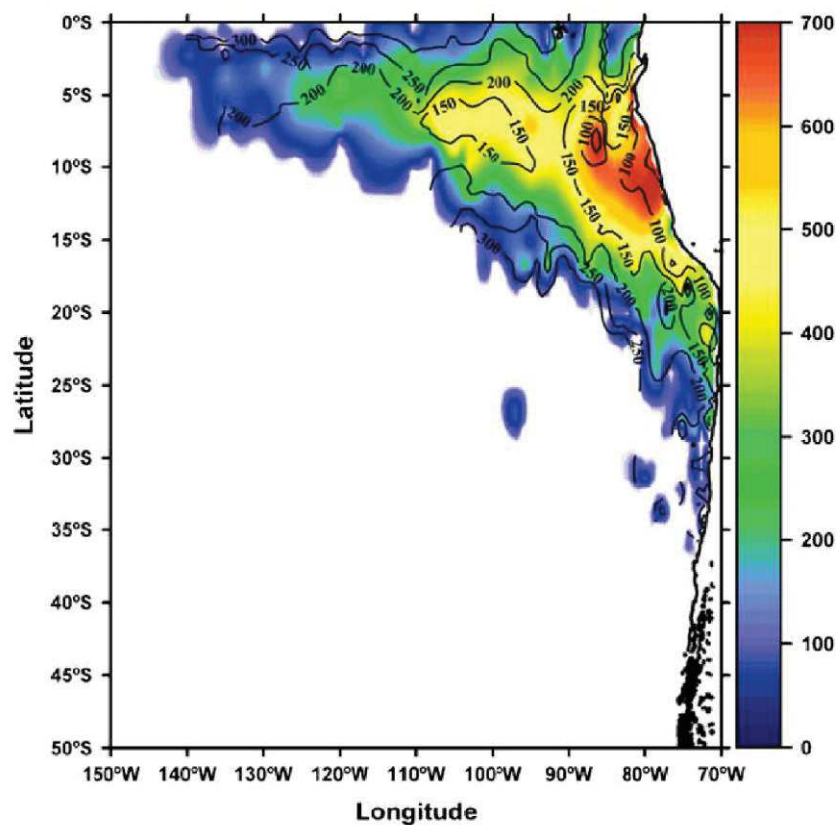
Figure 1.7. Oxygen Minimum Zone (OMZ, < 20 μmol kg -1 ) thickness (m) in the south-eastern Pacific. Thickness is colour-coded according to the color bar on the right-hand side of the figure. The upper boundary of the OMZ is shown in black contour lines with 50 m intervals. Source Fuenzalida et al. 2009.
