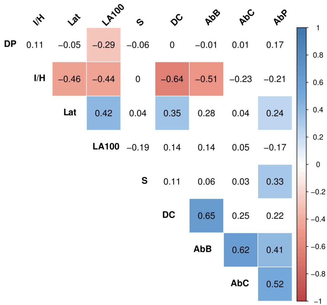
Figure A4. Correlation matrix of Site-specific, abundance of seabirds and fisheries variables.
