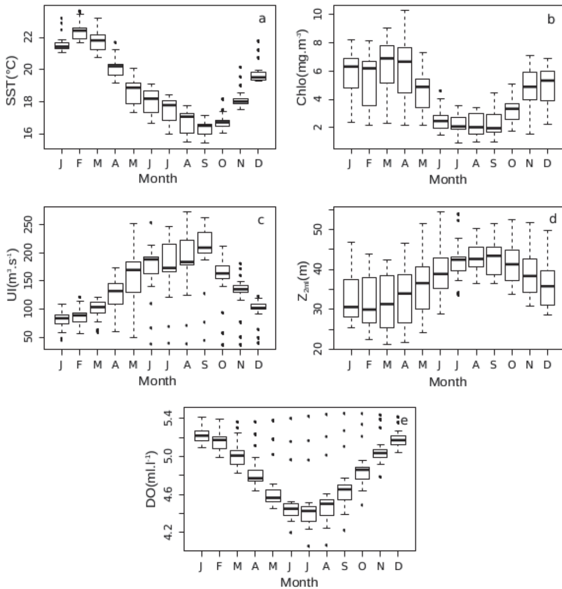
FIG.. E1. Monthly climatology profiles of (a) sea-surface temperature (SST), (b) chlorophyll (Chlo), (c) upwelling index (UI), (d) oxycline depth ( Z_{2ml}l^{-1} ) and (e) dissolved oxygen concentration (DO) at the surface. The boxplots were constructed from the site-specific climatology profiles built over an area covering a radius of 100 km around each breeding site. Periods encompassed 1999-2009 for SST, Chlo and UI and 1960-2010 for DO and Z_{2ml}l^{-1} .
