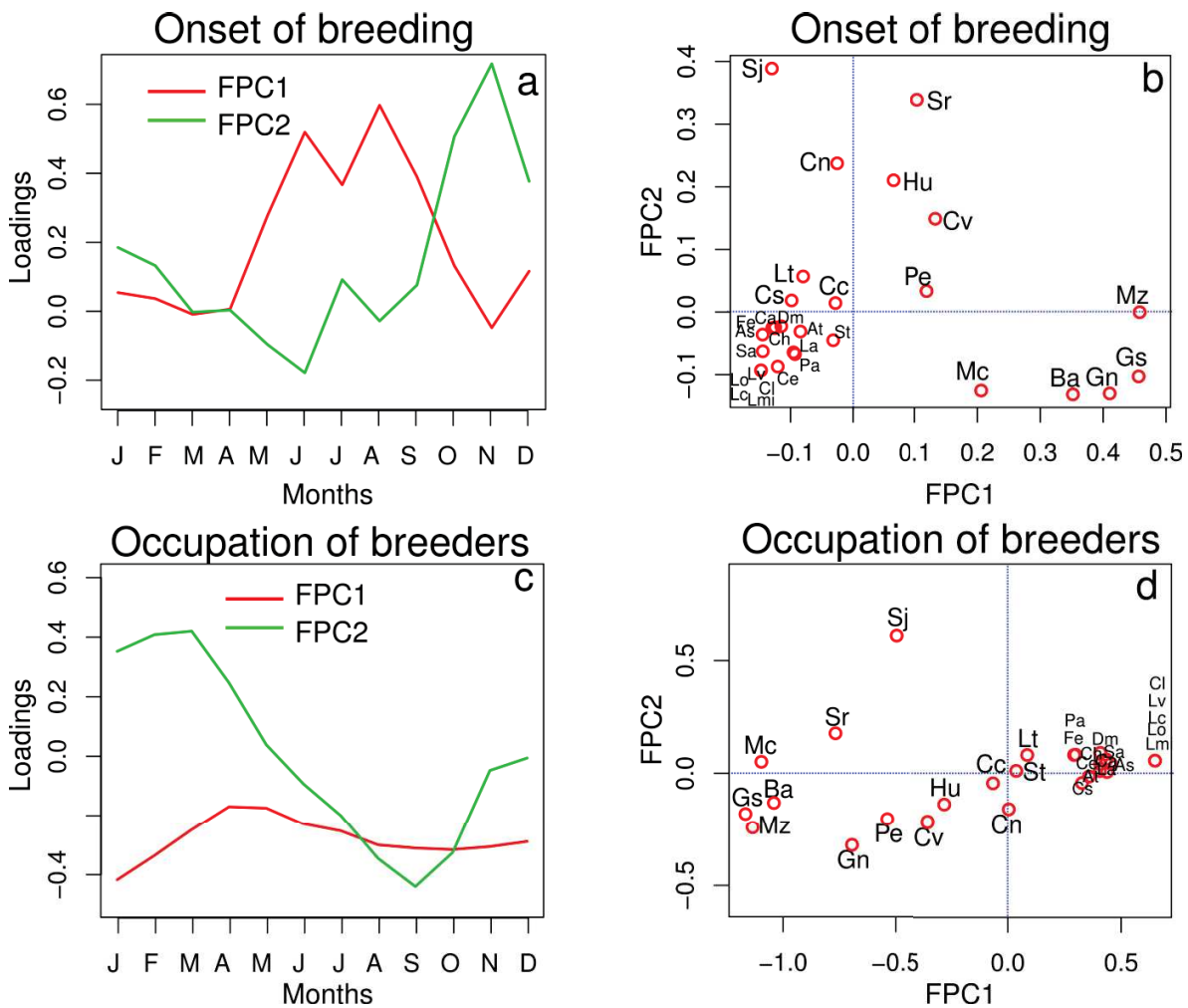
Figure 3.3. Functional Principal components of onset and occupancy of cormorant. Loadings of timing and magnitude of onset of breeding of cormorant were represented on the left (a and c) and the bivariate plot of scores of each colony for FPC1 and FPC2 (b and d) were represented on the right. Extended names of the nesting sites are described in Appendix A.
