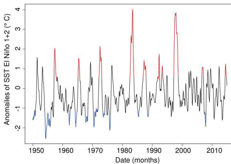
Figure 1.23. Time series of the SST anomalies in the El Niño 1+2 are. Red portions of the line refer to EN conditions according to Trenberth 1997 and portions in blue refer to LN conditions according to Trasmonte and Silva 2008. Source of time series:
