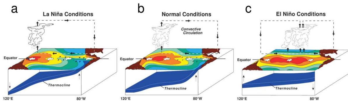
Figure 1.21. Schematic representation of a) La Niña, b) Normal conditions and c) El Niño conditions in the Pacific Ocean. Source: NOAA / PMEL / TAO Project Office.
