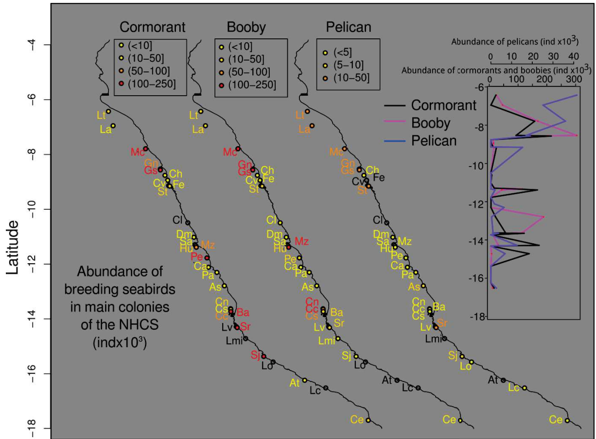
Figure A3. Map of localization of nesting colonies for the three seabirds. Colony size is represented by colors. Largest colonies are represented in red (100 000 – 250 000 for cormorant and booby and 10 000 – 50 000 for pelican) and smallest colonies in yellow (<10 000 for cormorant and booby and <5 000 for pelican). In the left panel longitude is suppressed and latitudinal effect on colony size is showed for the thee species.
