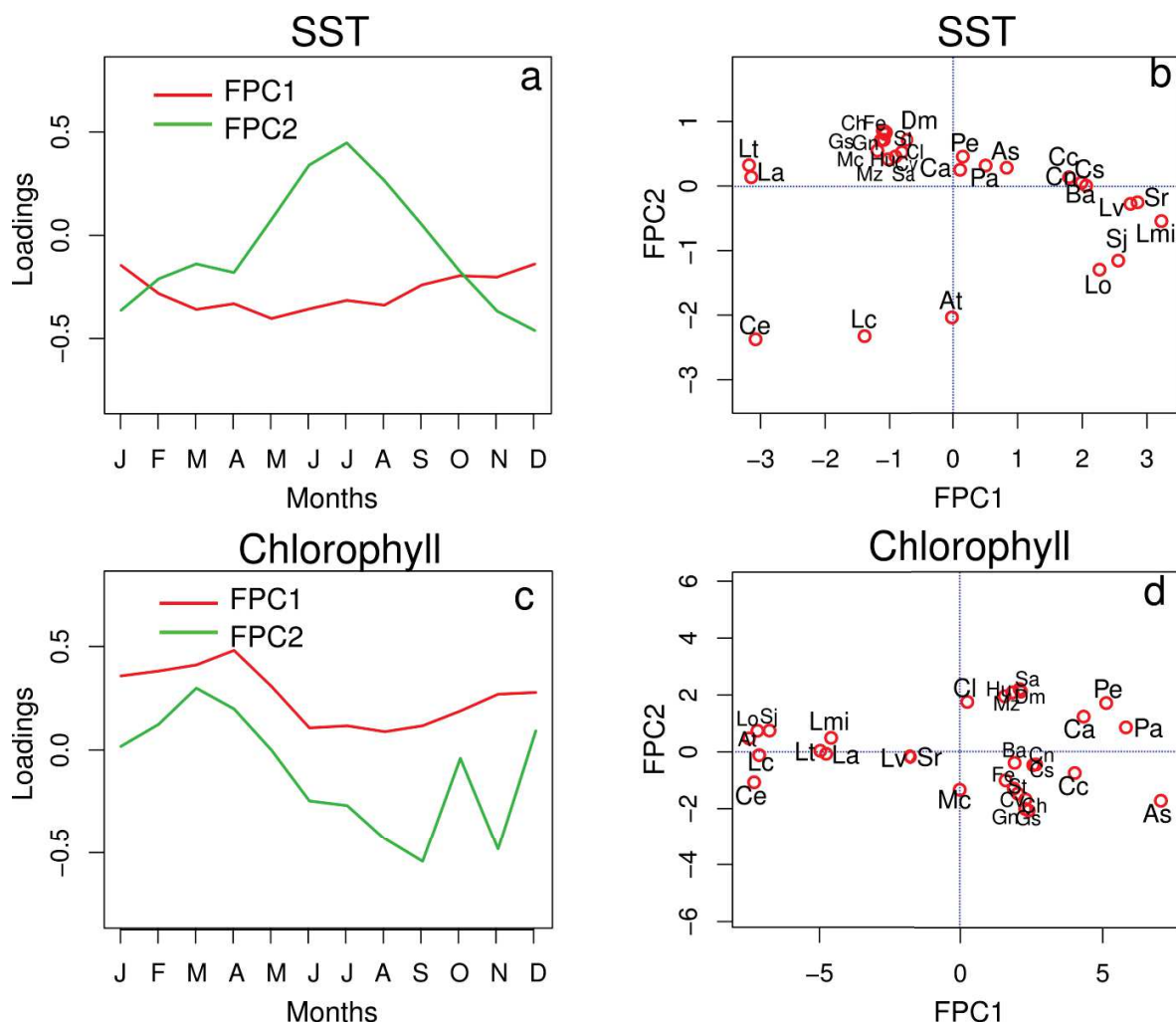
Figure 3.1. Functional Principal components of SST and Chlorophyll. Loadings (a and c) were represented on the left and the bivariate plot of scores of each colony for FPC1 and FPC2 (b and d) were represented on the right. Extended names of the nesting sites are described in Appendix A.
