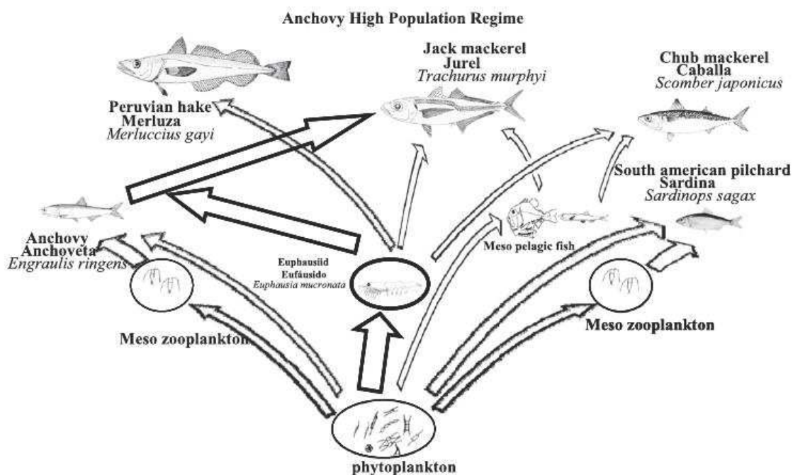
Figure 1.8. Simplified food web of NHCS, centered on euphausiid Euphausia mucronata during a period of high biomass of anchovy Engraulis ringens . Thickness of the arrows indicates the relative flow of biomass between components. Souce Antezana 2010.
