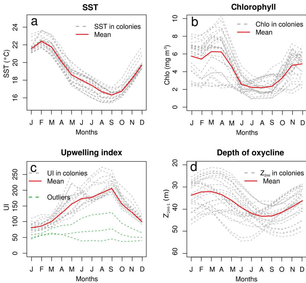
Figure D2. Mean (red lines) and outliers (green lines) of oceanographic conditions.
