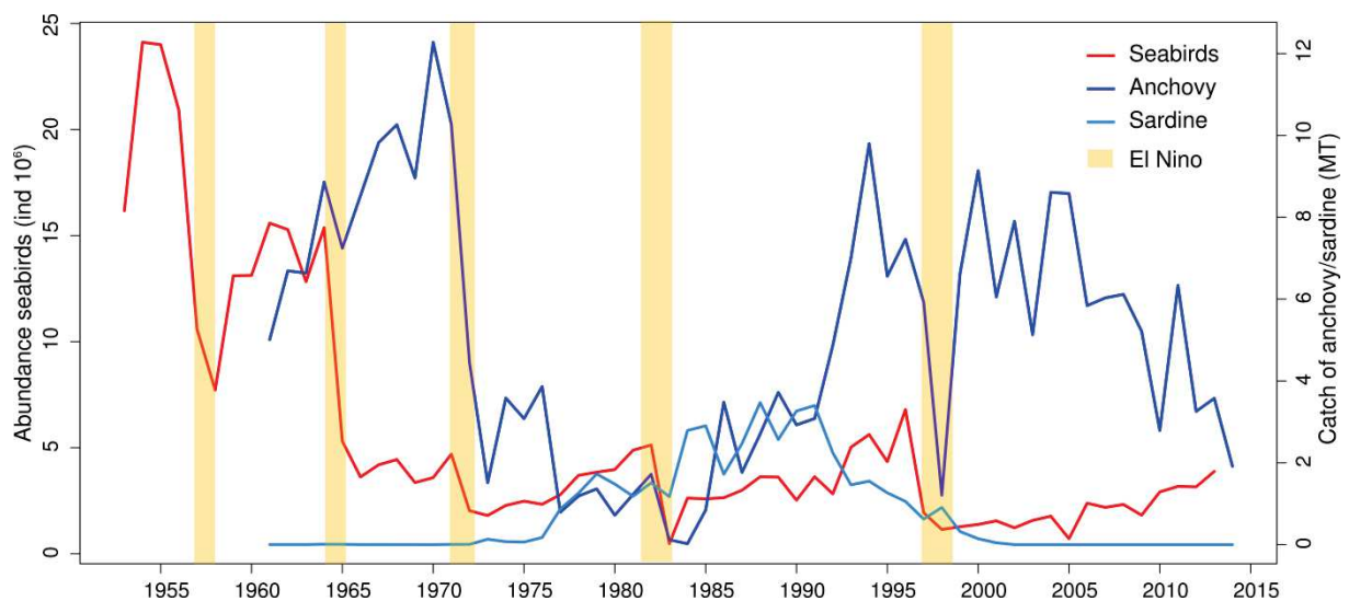
Figure 1.14. Abundances of seabirds (cormorants, boobies and pelicans) from 1952 to 2014, and catch of anchovy and sardine. Years when strong El Niño events occurred are marked by orange bars. Data source AGRORURAL and IMARPE.
