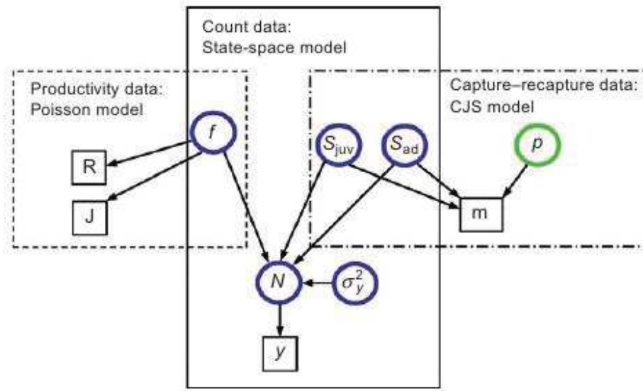
Figure 5.3. Graphical representation of an integrated population model (IPM) within a Bayesian approach. Small squares represent the data, circles the parameters (blue: target parameters, green: nuisance parameters), large squares the individual submodels, and arrows the flux of information. Circles appearing in two submodels indicate that they are informed from two data sources. IPM model represent three data types: i) count data where y is the observed data, N is the true abundance and \sigma^2y is the observational error; ii) productivity data where J is the number of nestling recorded and R is the annual number of surveyed broods; and iii) capture-recapture data where m is the number of released individuals never captured, S_{juv} and S_{ad} are survival of juveniles and adults respectively and p is the observational error. Source Kéry & Schaub 2012.
