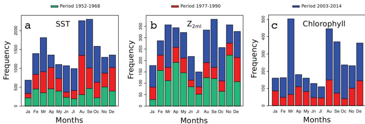
Figure S2. Barplots of data available of a) SST, b) Z_{2ml}^{-1} and c) Chlorophyll for each month during the periods: 1952-1968 (green), 1977-1990 (red) and 2003-2014 (blue).
