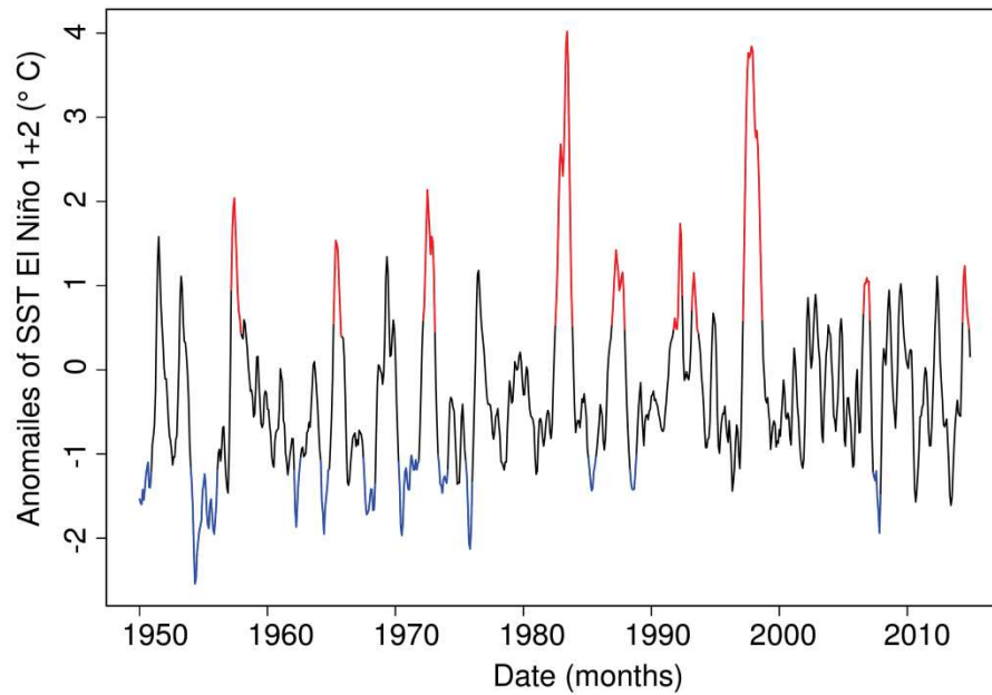
Figure S3. Anomalies of sea surface temperature of the zone El Niño 1+2 since 1950 to 2014. Base climatology to analyze the anomalies was built from 1981-2010 ( http://www.cpc.ncep.noaa.gov/data/indices/ersst3b.nino.mth.81-10.ascii ). Continuous anomalies for more than 5 months and higher than 0.4^{\circ}\text{C} are identified as El Niño events (Trenberth 1997, red lines) and continuous anomalies for more than 5 months and lower than -1.0^{\circ}\text{C} are identified as La Niña (Trasmonte & Silva 2008, blue lines).
