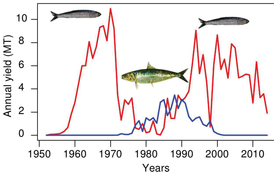
Figure 1.13. Time series of annual yield (MT) of anchovy and sardine in the NHCS. Source of data, IMARPE.
