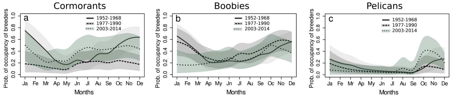
Figure 4.3. Monthly average estimates of probability of occupancy of breeders for cormorants (a), boobies (b) and pelicans (c) during 1952-1968 (solid lines), 1977-1990 (dashed lines) and 2003-2014 (dotted lines). Shaded areas represented the 95% and 5% of the posterior distribution of monthly probability of onset of breeding. Breeding onset probability lines were smoothed with a loess model with 0.45 of span.
