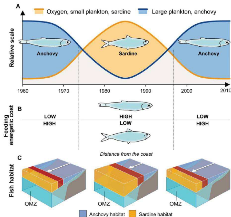
Figure 1.20. Conceptual model of decadal changes in anchovy and sardine populations in the southeastern tropical Pacific. Schematic representation of a) the temporal changes in abundance of large plankton and anchovy (blue) and small plankton and sardine (orange) during 1960-2010. b) Energetic costs of feeding on dominant plankton size-spectra for anchovy and sardine according to the scenarios from a. c). Schematic of the available habitat for anchovy (blue shaded area) and sardine (red shaded area). Source, Bertrand et al. 2011.
