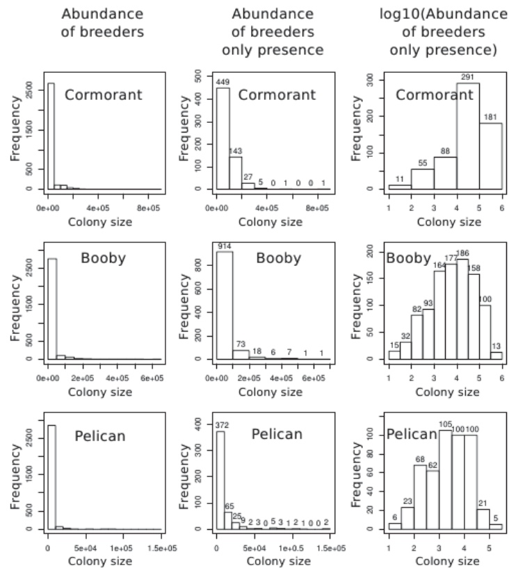
FIG. D1. Colony size frequency distribution for the three species of cormorants, boobies and pelicans. Histograms correspond to the raw abundance data (left column), the abundance data without breeder absences (central column), the abundance data without breeder absences once log10-transformed (right column).
