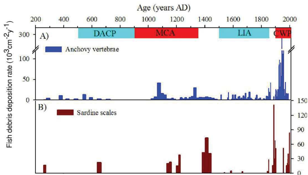
Figure 1.19. Fish debris deposition rates off Pisco, Peru for A) Anchovy vertebrae fluxes ( \# \text{vertebrae} \cdot 10^3 \text{y}^{-1} \text{cm}^{-2} ) and B) Sardine scale fluxes ( \# \text{scales} \cdot 10^3 \text{y}^{-1} \text{cm}^{-2} ). Highlighted areas indicate the Current Warm Period (CWP from \sim 1900 to the present), Little Ice Age (LIA, from 1500 to 1850AD), the Medieval Climate Anomaly (MCA, from 900 to 1350AD) and the Dark Ages Cold Period (500 – 900 AD). Source Salvattecchi 2013.
