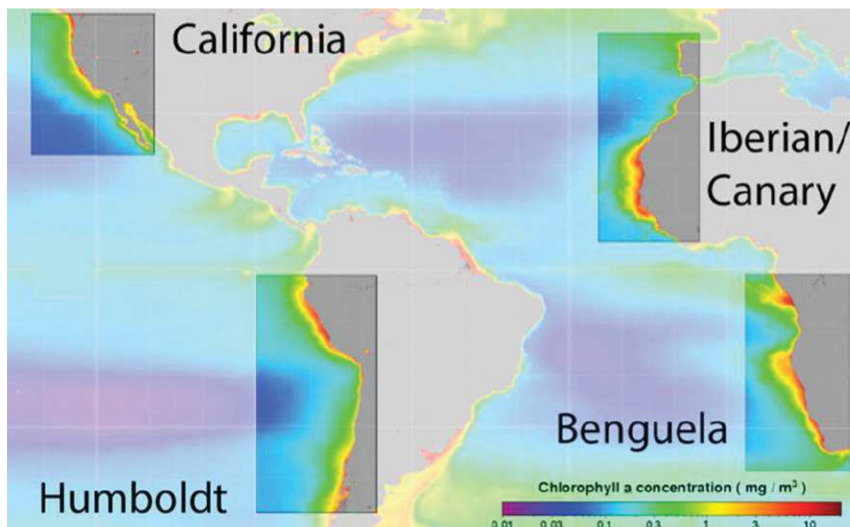
Figure 1.1. EBUS localization and their chlorophyll-a annual average concentrations. Source Bakun et al. 2015.
