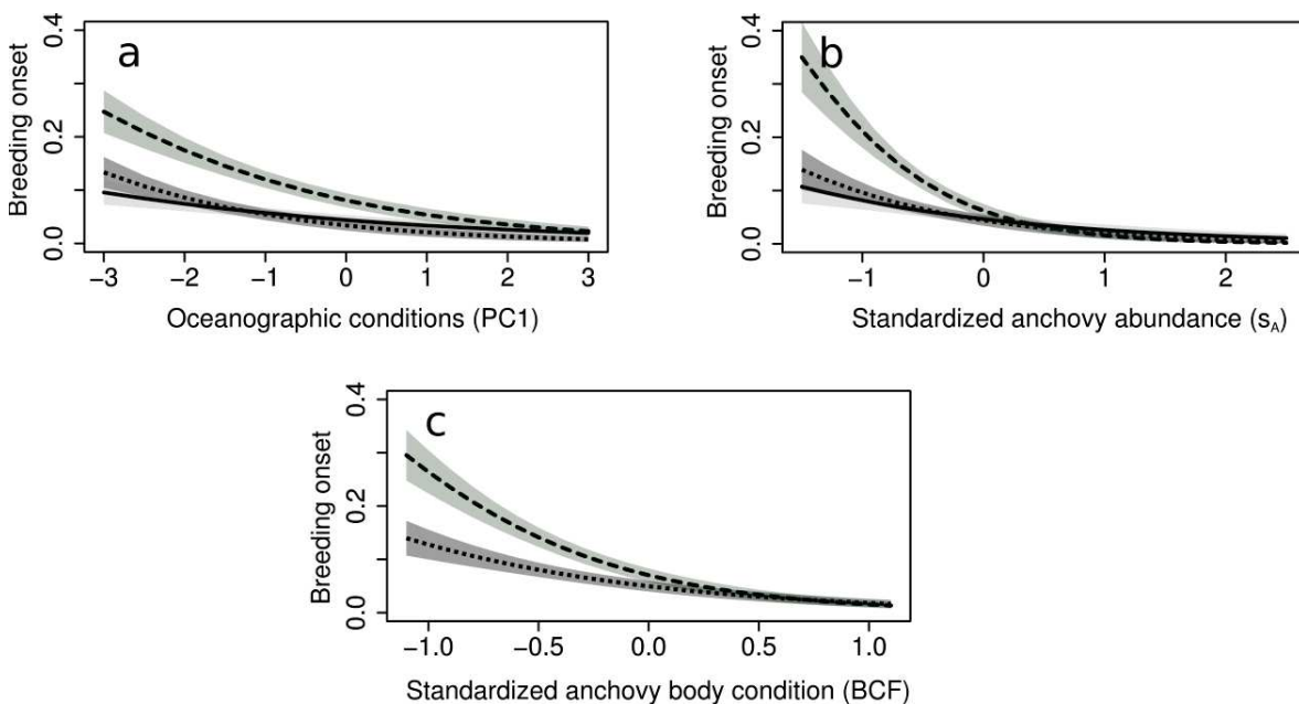
FIG.2.3. Modeled probabilities of breeding onset as a function of (a) oceanographic conditions (PC1 standardized), (b) the standardized regional anchovy abundance ( s_A ), and (c) standardized anchovy body condition factor (BCF) for boobies (dashed lines) and pelicans (dotted thick lines). The functional relationships were obtained from the selected models for each species ( P < 0.005 and highest R^2 ). Shaded areas represent = 95% confidence intervals.
