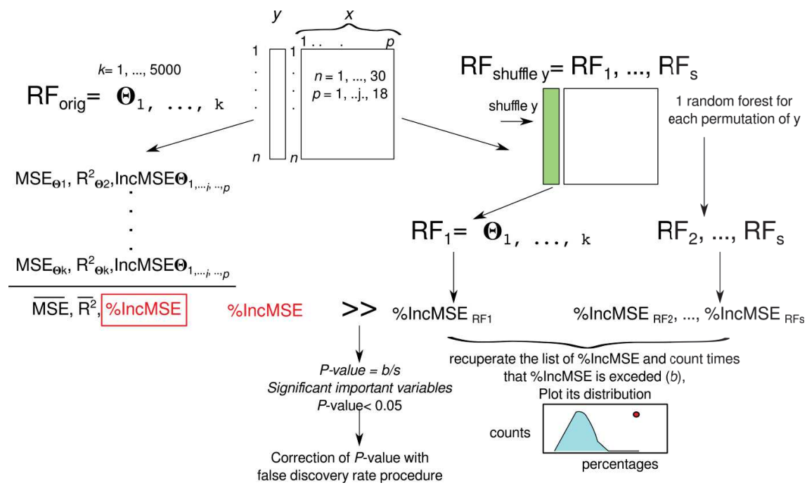
Figure C2. Schema of PIMP procedure for correct categorical variable bias importance and select only significant important variables.
