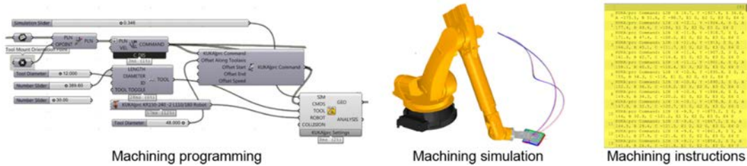
Figure 218. Kuka|Prc workflow.
