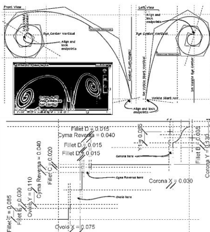
Figure 72. Parametric setup for a Volute and an architrave using Autodesk Revit. On: Renaissance Revit, by P.Aubin 2013.
