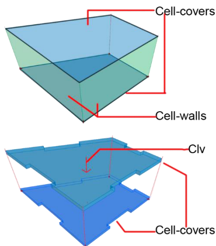
Figure 209. Cell cover rebuilding and joint definition. Top. Cell-wall boundaries are used to recover cell-cover geometry. Bottom. After joint profiles are added, cell-covers are extruded along a Clv vector.
