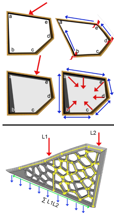
Figure 161. Load transmission in cellular systems. Top , left to right, top to bottom. An open cell receiving a vertical load cannot stand by itself as no combining or bracing elements are present to keep cell-walls together; theoretically, joints would fail to maintain the cell stable. In a second scenario, a closed cell undergoes the same vertical load. Charges are uniformly distributed through cell-walls with the help of a diaphragm (cell cover) avoiding the cell from collapsing. Bottom . A theoretic gravity effort, caused by two transformed gravity loads L1 and L2, acts over a set of confined cells. All elements work as a whole despite being open. Loads, as grouped in \Sigma L1L2 , are transmitted through cell-walls and confinements to a lower member that uniformly distributes them to the ground.
