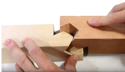
Figure 141. Top. Scarf-like Japanese beam-joint. (Building Channel, 2016) Bottom. Three-way Japanese interlocking joint (Wandel, 2015).
