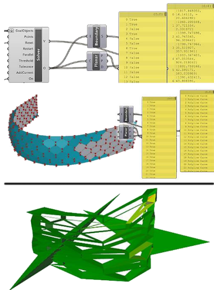
Figure 196. Planarizations using Kangaroo for GH. Top. A planarization test on a regular pattern as applied to a given W_r . With the right parameters, the add-on achieves the given goals in a matter of seconds. Bottom. When constraints are too difficult to fulfill the solving tool will however output a morphologically and topologically altered geometry set.
