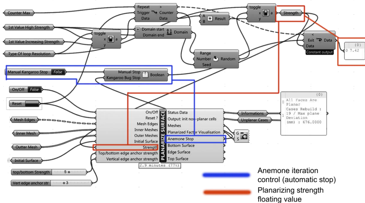
Figure 200. Fab-Cell's morphologic solver (planarization). Planarizing forces are regulated by loop component that dispatches and tests values for positive planarization. When the correct value is found, anemone stops iterating and lets Kangaroo to go on until it completes the solution.
