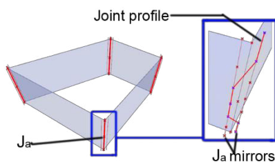
Figure 207. Creation of a joint profile in a cell-set knot.
