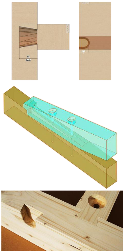
Figure 126. Top. Joint definition using HSBcad ( https://hsbcad.uservoice.com ). The program has a direct link to Autodesk Revit, allowing it to import framing models thus giving the base parameters to define the best jointing method for a set of structural members. Middle. Joist-rafter joint (including drillings) as calculated through a CAD-and-CAM software. Bottom. Machined wood joinery as derived from CAD-to-CAM or CAD-and-CAM workflows.
