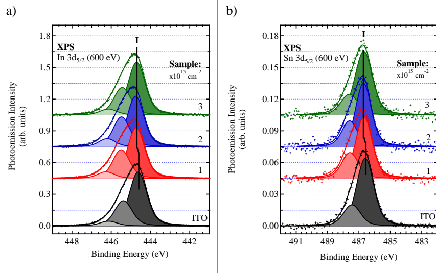
Figure III.5 – a) In 3d 5/2 and b) Sn 3d 5/2 spectra of the chemically cleaned ITO sample and covered with increasing layers of DIPO-Ph 4 . The photon energy is indicated. The spectra were recorded at the TEMPO beamline. Coverages are obtained from QB-coverage.
