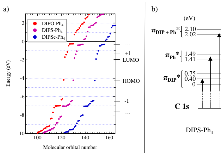
Figure V.1 – a) DFT calculated molecular orbital levels; b) Electronic scheme of the C 1s of DIPS-Ph 4 . Indicated energies are related to the LUMO.
