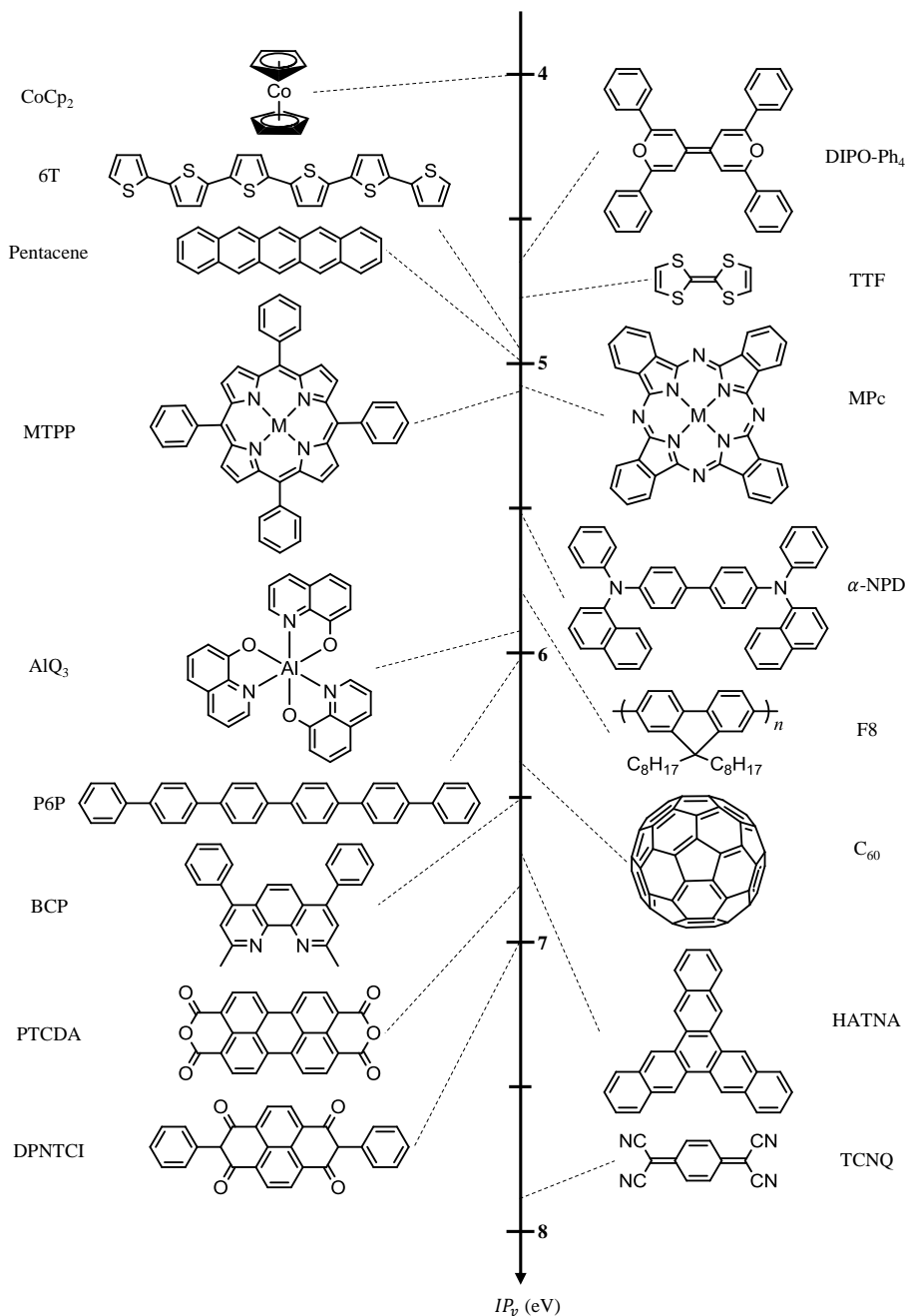
Figure I.5 – The structure and ionization energy IP_v (in eV) of common materials used for organic electronics study. The full names of the compounds are: cobaltocene (CoCp 2 ), tetraphenyl-dipyranlydene (DIPO-Ph 4 ), tetrathiafulvalene (TTF), sexithiophene (6T), metal phtalocyanine (MPc), metal tetraphenyl-porphyrin (MTPP), N,N'-di(1-naphthyl)-N,N'-diphenyl-(1,1'-biphenyl)-4,4'-diamine ( \alpha -NPD), poly(9,9-di-n-octylfluorenyl-2,7-diyl) (F8), fullerene (C 60 ), bathocuproine (BCP), hexaazatrinaphthylene (HATNA), perylenetetracarboxylic dianhydride (PTCDA), N,N'-diphenyl-1,4,5,8-naphthyltetracarboxyldiimide (DPNTCI), tetracyanoquinodimethane (TCNQ).
