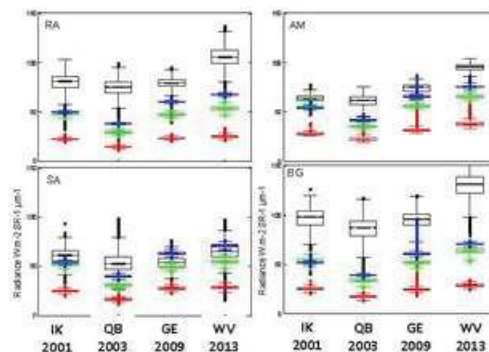
Fig. 6. Radiance signatures of the four forest types as observed by all sensors.
